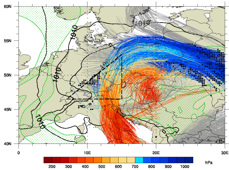
Fig. 1. As Figure 6b BUT with a weaker ascent criterion of 500hPa (48h) \{ \} \{-1\} , and trajectories plotted only with six-hourly position output.
