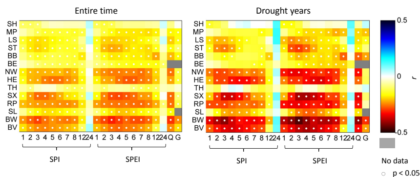
Figure 1: Rank correlation coefficients ( r ) between timeseries of drought indicators ( \overline{SPI} or \overline{SPEI} or streamflow ( \overline{Q} ) or groundwater level ( \overline{G} ) percentiles) and drought impact occurrences ( I ) per federal state. The left panel displays r based on the entire timeseries ( n=504 ), while the right panel shows r based on the months of selected drought years ( n=204 ). The right panel is the same as the top left panel in Figure 3 of the manuscript except for the adapted colour scheme as suggested by referee # 1.
