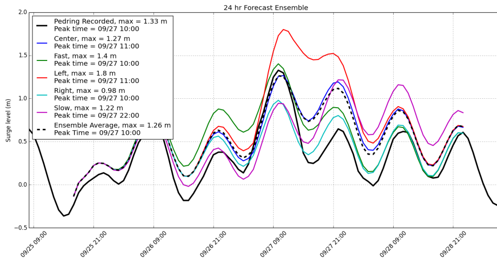
Fig. 2. JMA Storm Surge Model Validation
