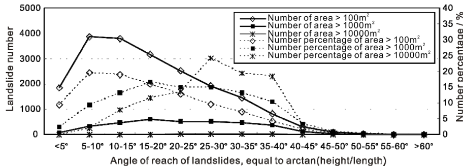
Fig. 16. Landslide angle of reach [ \arctan(\text{height}/\text{length}) ] distribution.
