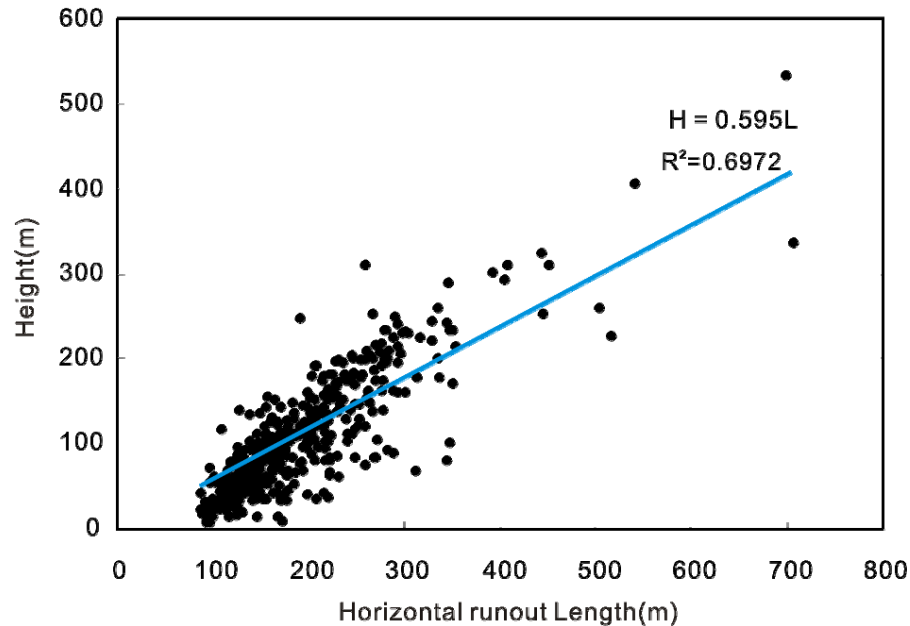
Fig. 15. Relationship between landslide height and horizontal runout length. A total of 453 landslides of area larger than 10\,000\text{ m}^2 triggered by the Haiti earthquake were used to carry out the statistics.
