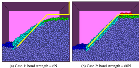
(a) Case 1: bond strength = 6N (b) Case 2: bond strength = 60N Figure 11 Eventual failure of two modeling cases under loading raft in XY direction (with external load 500N)
