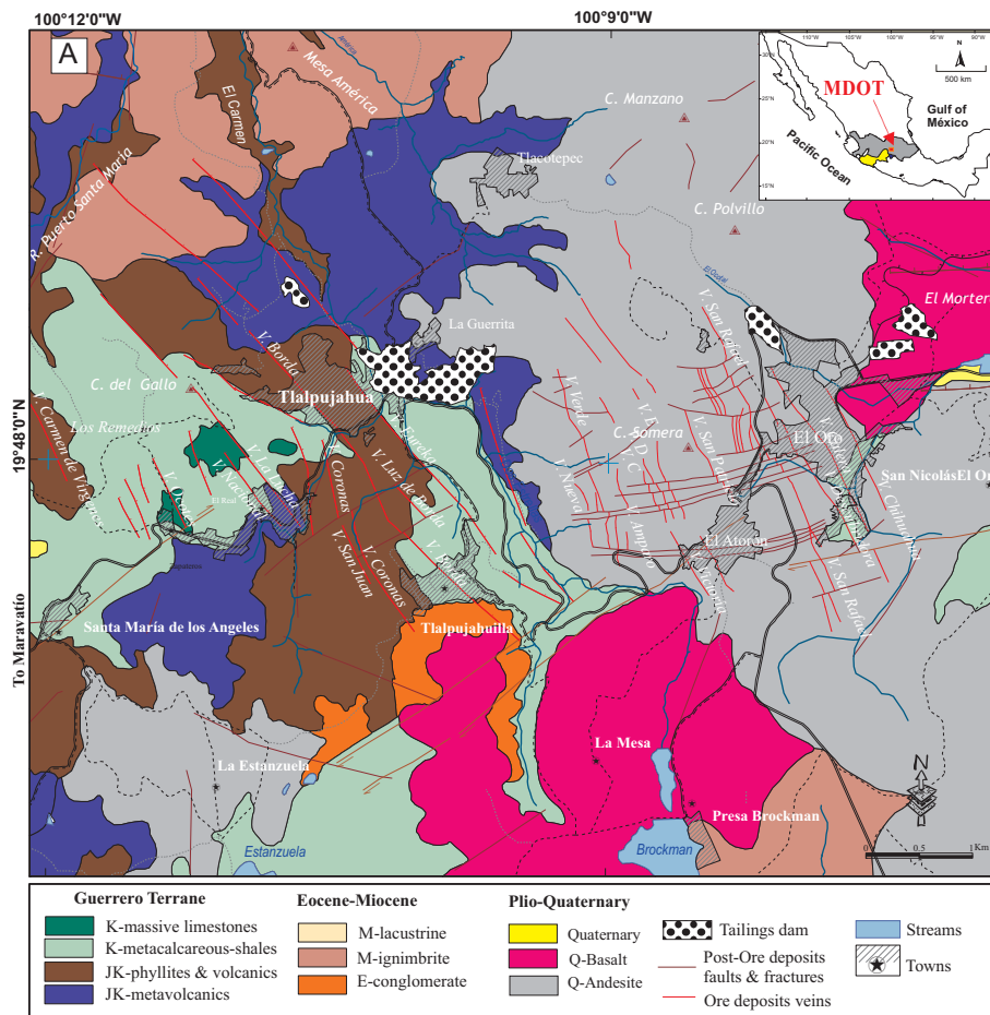
Figure 1. Location of the Mining District of El Oro-Tlalpujahua (MDOT) in Central Mexico (inset), showing the principal rock types, ore veins, and tailings dams. Geological map of the MDOT from Corona-Chavez et al. (2010).
