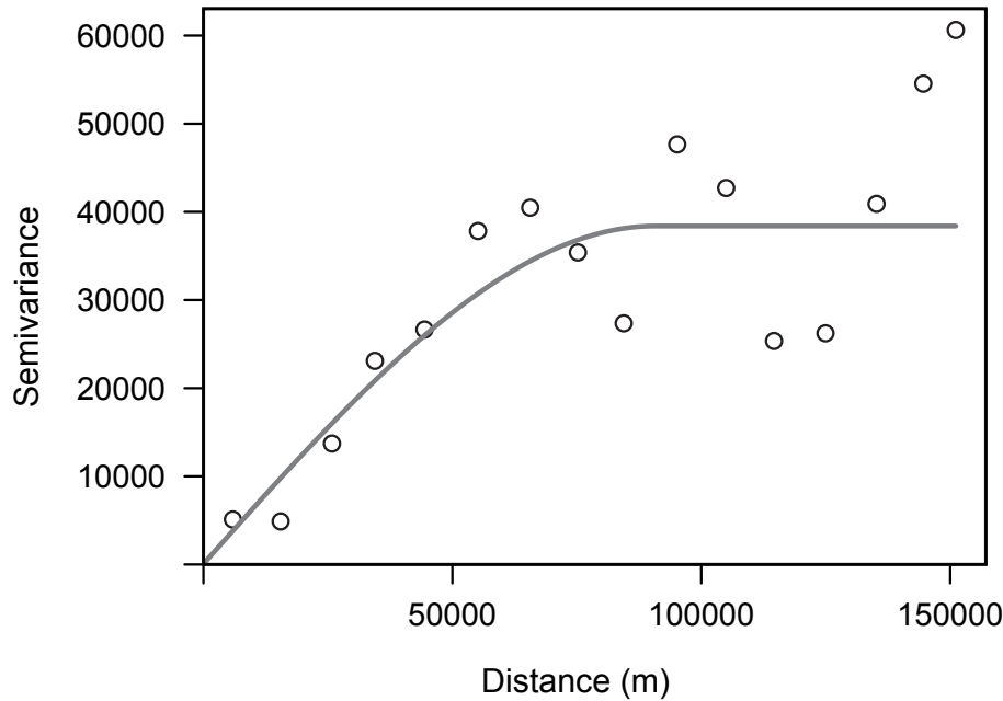
Figure 4. Empirical residual semivariogram of two-week antecedent precipitation after accounting for elevation, and a fitted spherical semivariogram model.
