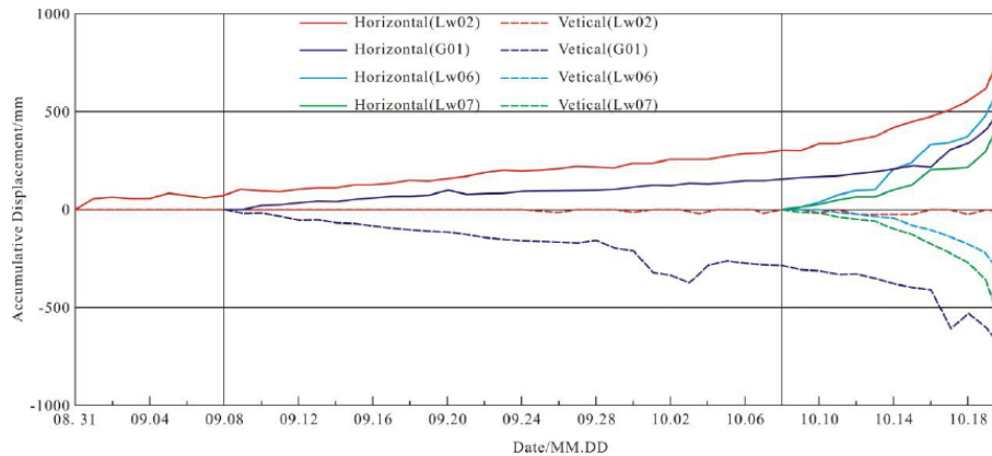
Figure 12. Cumulative displacement at monitoring stations at the Wangxia rock slump (Le et al., 2011).
