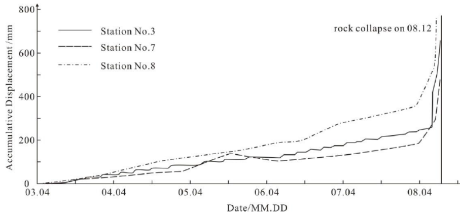
Figure 9. Cumulative displacement of monitoring stations at the crest of Zengzi Cliff in 2004 (Ren, 2005).
