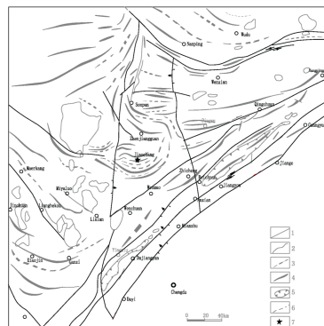
1. Main faults; 2. Boundary of intrusive rock; 3. Syncline; 4. Anticline; 5. Klippe; 6. Inferred fault; and 7. the Diexi barrier lake
