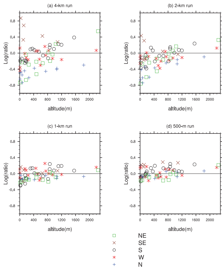
Fig. 9. Bias of 4 day rainfall at each rain gauge station, as a function of the altitude and locations for the (a) 4, (b) 2, (c) 1 and (d) 0.5 km runs. The data are divided into 5 geographical zones: NE (green squares), SE (brown crosses), S (black circles), W (red stars) and N (blue +).
