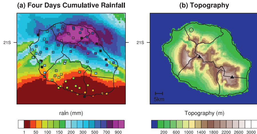
Fig. 2. (a) Cumulative precipitation (in mm) during the four days measured by rain gauges (squares) and estimated by the weather radar (colored areas). A black square means that there is at least one-hour missing record at such rain station. (b) Topography of La Reunion (in m) with five areas (N, W, S, SE and NE) defined by the local disaster management service. The location of the weather radar is indicated by the circle and the black triangles represent the Piton de la Fournaise at the south-east and Piton des Neiges in the center.
