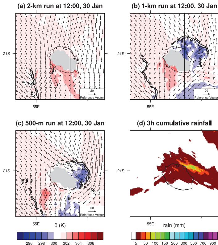
Fig. 10. Simulated horizontal wind field ( \text{m s}^{-1} ) and potential temperature (K, colors) at 950 hPa in the (a) 2 km, (b) 1 km and (c) 500 m runs. The black contours represent the vertical velocity at 1 \text{ m s}^{-1} at 950 hPa. The north-south line segments correspond to the locations of the vertical cross sections in Fig. 11; (d) 3 h cumulative rainfall (12:00 to 15:00 UTC; in mm) estimated by radar with the positions of two meteorological stations: Gillot-Airport (triangle) and Le Colosse (square).
