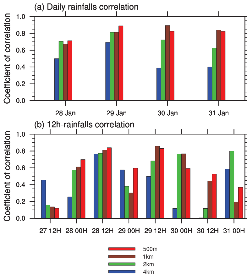
Fig. 6. Spatial correlation coefficient between simulated and observed rainfall (in mm) cumulated over (a) 24h and (b) 12h for the four runs: 4 km (blue bars), 2 km (green bars), 1 km (brown bars) and 500 m (red bars).
