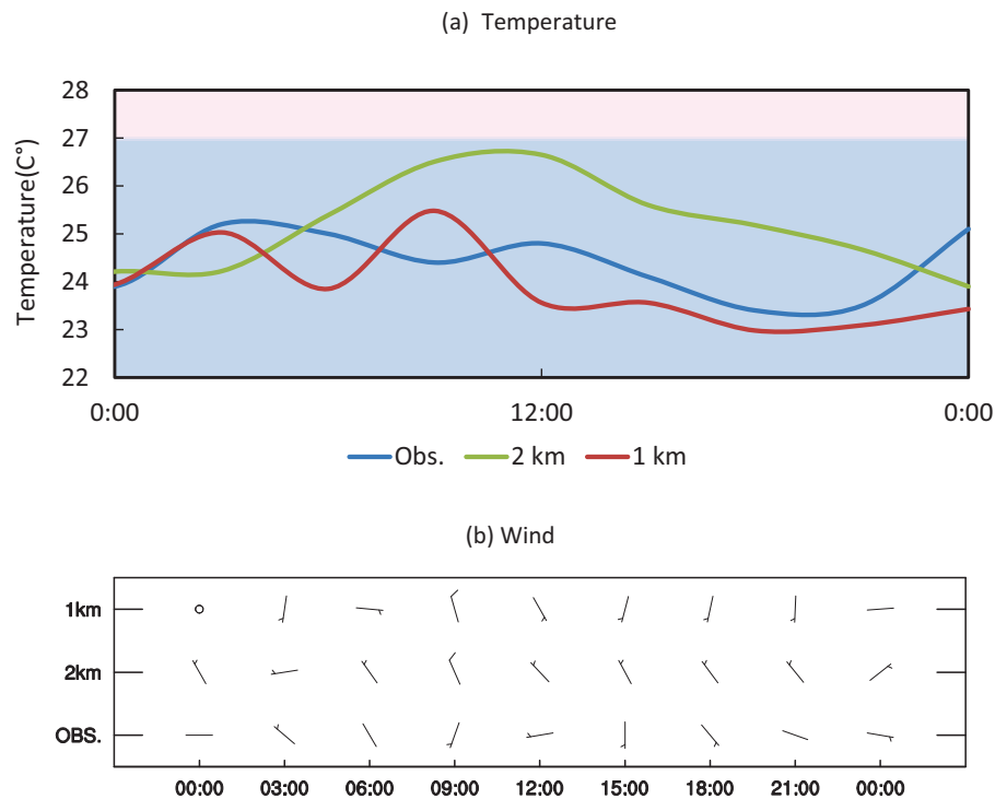
Fig. 12. (a) Average temperature (°C) simulated by the 2 km (green curve) and 1 km (red curve) runs and observed (blue curve) at Le Colosse and Gillot-Airport stations. The background boundary indicates the climatological temperature in January at La Réunion; (b) observed and simulated horizontal wind at Gillot-Airport station during the last day of the event.
