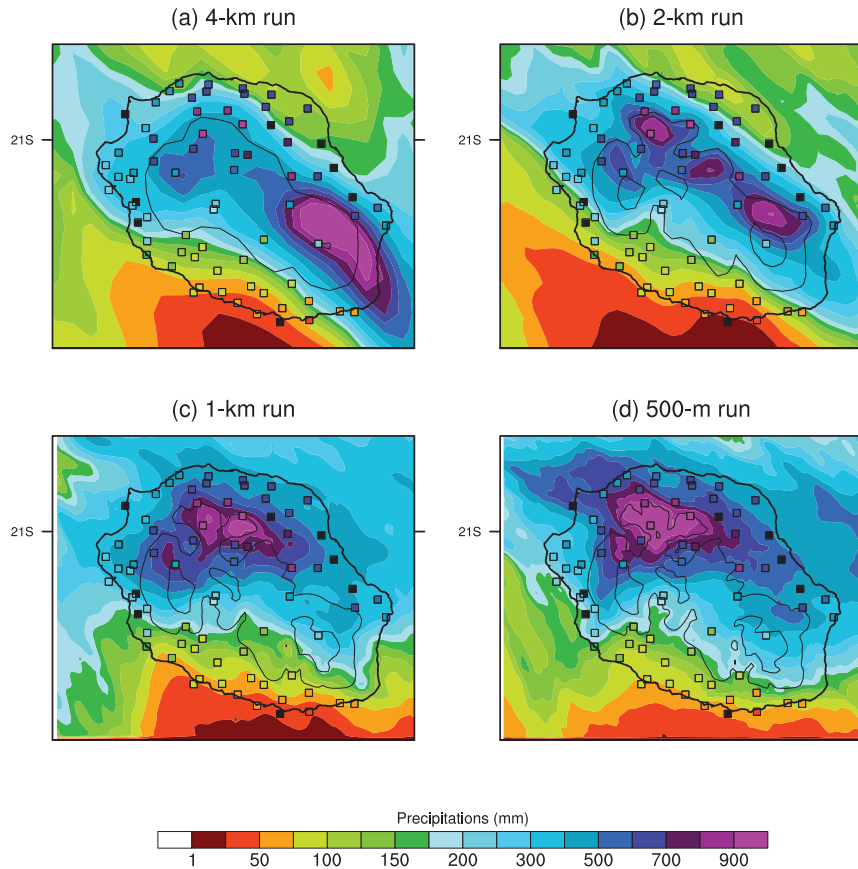
Fig. 3. 4 day cumulative rainfall (in mm) produced by the (a) 4 km, (b) 2 km, (c) 1 km and (d) 500 m simulations (colored area), superimposed with the raingauges measurements (squares). The black contours display the 1000 m and 2000 m altitude isolines as reproduced by the model at different resolutions.
