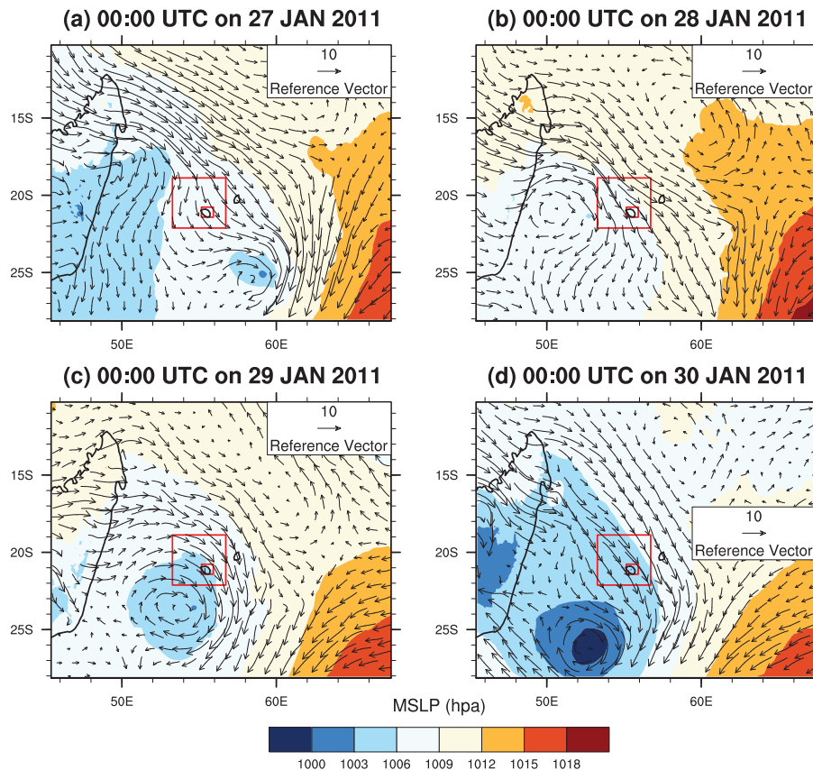
Fig. 1. Mean sea level pressure and horizontal wind at 850 hPa obtained from the Aladin-Réunion analyses at 00:00 UTC on 27 (a), 28 (b), 29 (c) and 30 (d) January. The red rectangles represent the two Meso-NH domains simulations: D1 (large one), D2 (small one).
