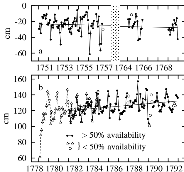
Figure 6. Corrected monthly means for Venice (a) and Chioggia (b). Straight lines represent linear fits. The horizontal axis in (a) is interrupted for display purposes.
