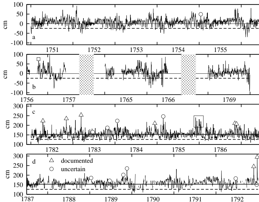
Figure 4. Daily sea level maxima for Venice ( a , b ) and Chioggia ( c , d ) in the original height scales converted to centimetres. Symbols indicate storm surge events quoted in Enzi and Camuffo (1995). The square in ( b ) indicates an event reported by Temanza (1751–1769) but not by Enzi and Camuffo (1995). The solid horizontal lines represent the CM at Venice ( a , b ) and the Mean High Water, as a proxy to the CM, at Chioggia ( c , d ). The dotted horizontal lines represent MSLs. The horizontal axis in ( b ) is interrupted for display purposes. See also text for more details.
