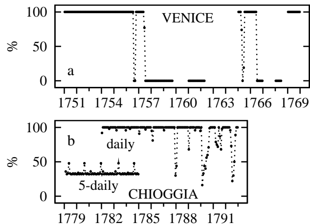
Figure 5. Monthly data availability at Venice (a) and Chioggia (b) as the percentage of days with data relative to the total. The absence of dots indicates the lack of data sources.
