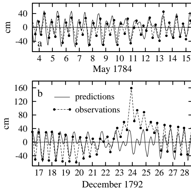
Figure 2. Comparison of observed data and tidal predictions at Chioggia from 4 to 15 May 1784 (a) and from 17 to 28 December 1792 (b) . Ticks on the horizontal axes correspond to noon.
