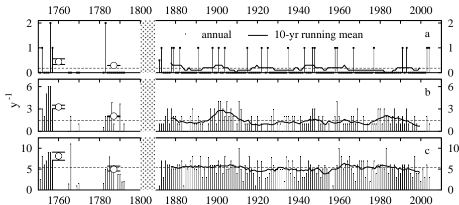
Figure 3. Frequencies of daily sea level anomalies above 55 cm (a), 37 cm (b) and 25 cm (c), corresponding to the highest 0.1, 1 and 5% of daily anomalies in 1872–2004, respectively. Annual values are represented by vertical bars, pseudo-decadal means by white circles and 10 year running means by solid lines. Dotted horizontal lines represent the 1872–2004 means. The horizontal axis is interrupted for display purposes.
