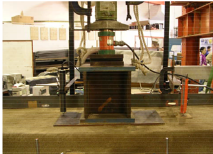
Figure 5. LVDT at top and sloping face of the model test.
