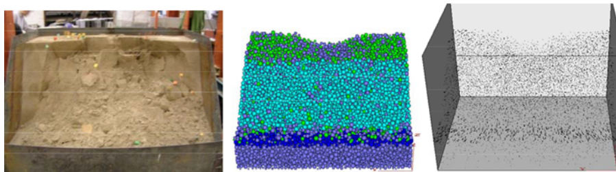
(a) Lab test - slope without soil-nail (b) DEM Case1 - bond strength = 6N (c) DEM displacement
