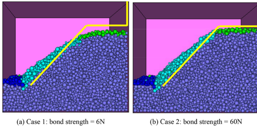
Figure 11. Eventual failure of two modeling cases under loading raft in XY direction.
