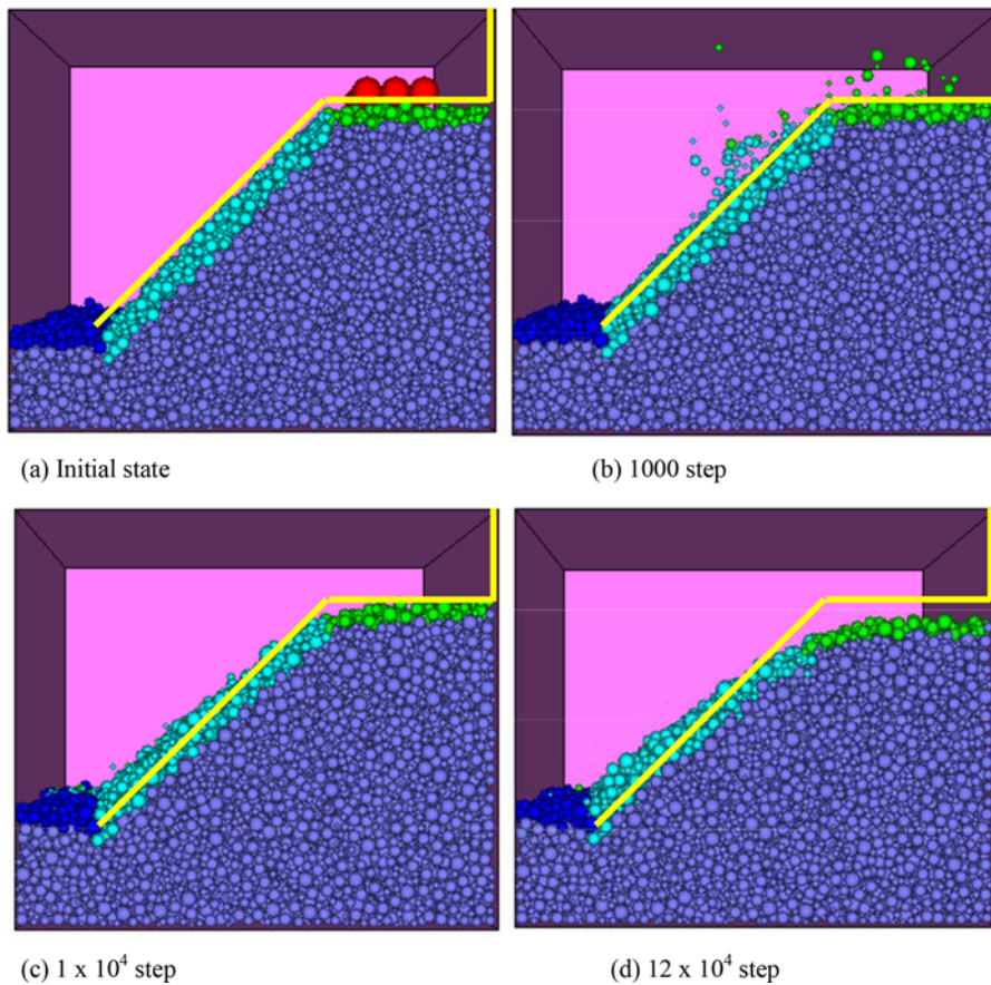
Figure 10. Failure process of numerical model under loading raft in XY direction.
