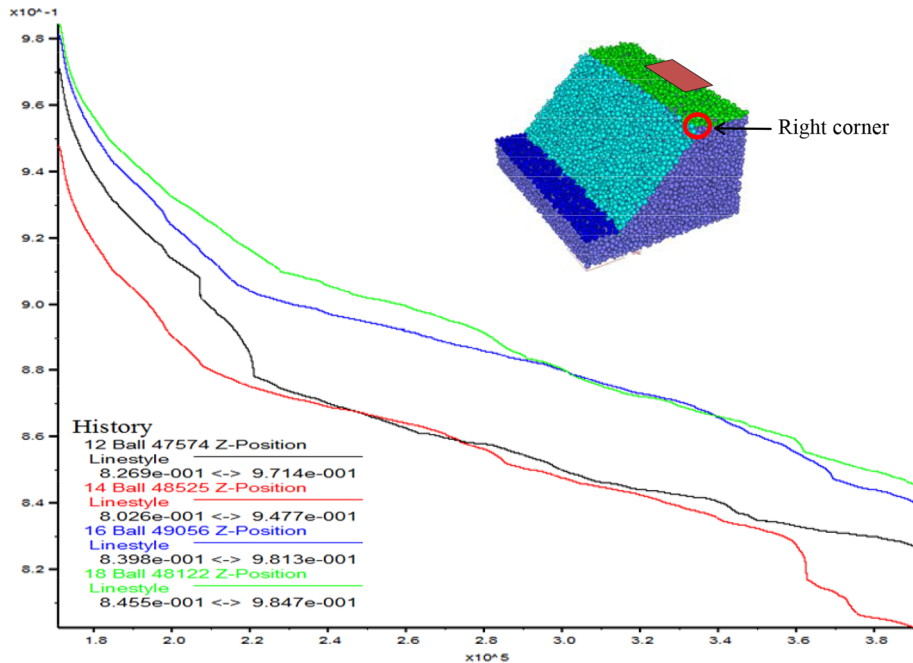
Figure 12. Vertical position history for balls at the right corner of crest.
