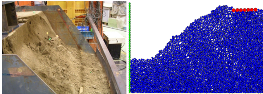
(a) Laboratory test of slope
