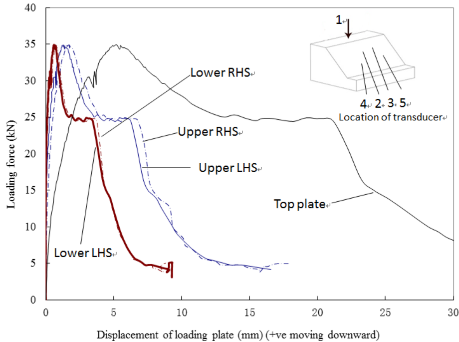
Figure 7. Loading force against the displacement of slope surface.
