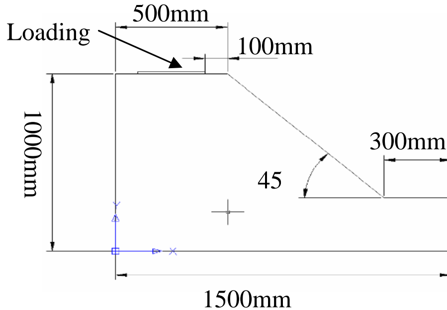
Figure 2. Section view of soil slope model.
