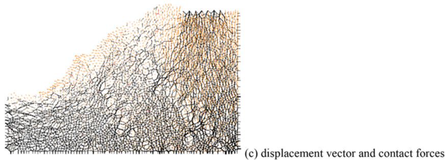
Figure 15. Side view for the final failure from laboratory test and DEM modelling.
