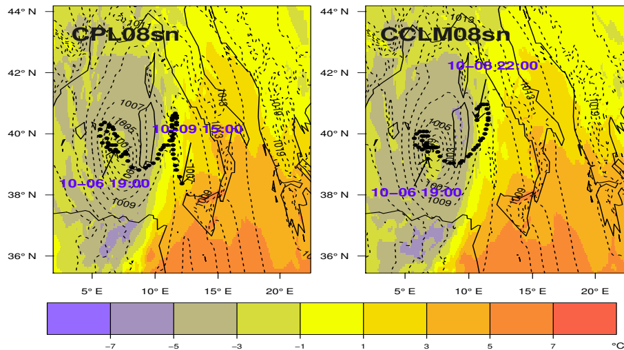
Fig. 4. ME08; mean sea level pressure (hPa; dotted contours lines at 2 hPa intervals) and temperature ( ^{\circ}\text{C} : colored contours at 2^{\circ}\text{C} intervals) at 700 hPa in coupled and atmosphere-only ( 0.08^{\circ} ) with spectral nudging simulations, on 7 October 1996 at 18:00 UTC.
