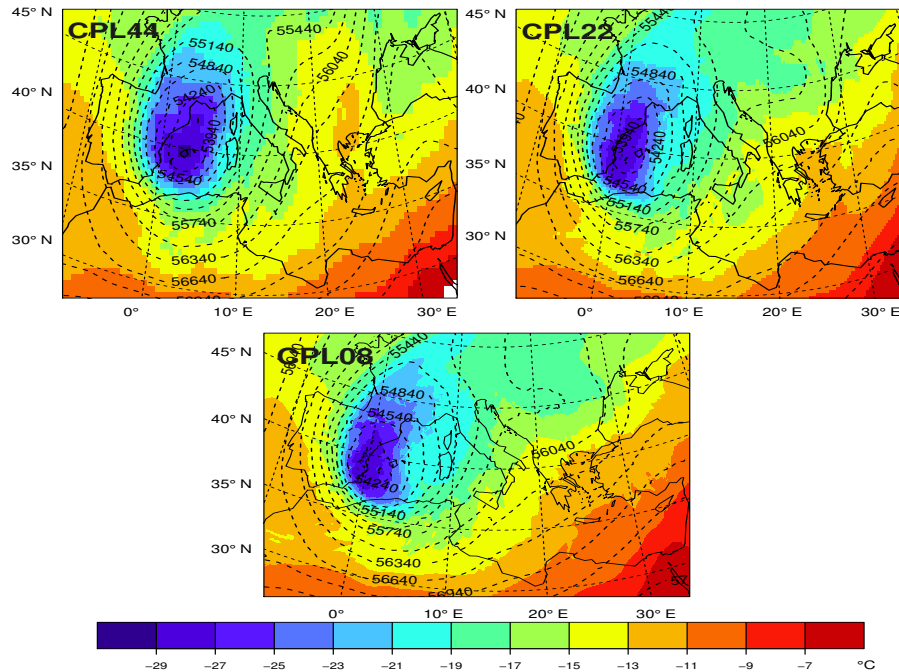
Fig. 1. ME08; geo-potential height ( \text{m}^2 \text{s}^{-2} ; dotted contours lines at 300 \text{m}^2 \text{s}^{-2} intervals) and temperature ( ^{\circ}\text{C} ; colored contours at 2^{\circ}\text{C} intervals) at 500hPa in coupled ( 0.44^{\circ} , 0.22^{\circ} , and 0.08^{\circ} ) simulations on 6 October 1996 at 03:00 UTC.
