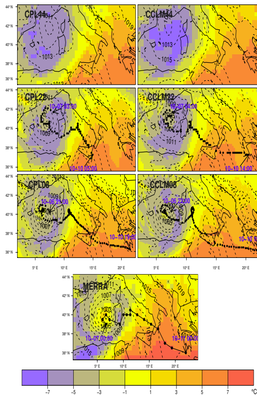
Fig. 2. ME08; mean sea level pressure (hPa; dotted contours lines at 2hPa intervals) and temperature ( ^{\circ}\text{C} : colored contours at 2^{\circ}\text{C} intervals) at 700hPa in coupled and atmosphere-only ( 0.44^{\circ} , 0.22^{\circ} , and 0.08^{\circ} ) simulations and the MERRA reanalysis data on 7 October 1996 at 18:00 UTC.
