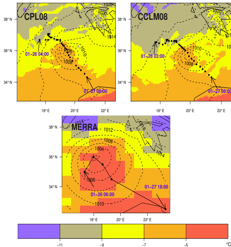
Fig. 10. ME10; mean sea level pressure (hPa; dotted contours lines at 2hPa intervals) and temperature (°C: colored contours at 2°C intervals) at 700 hPa in coupled and atmosphere-only (0.08°) simulations and the MERRA reanalysis data on 27 January 1998 at 00:00 UTC.
