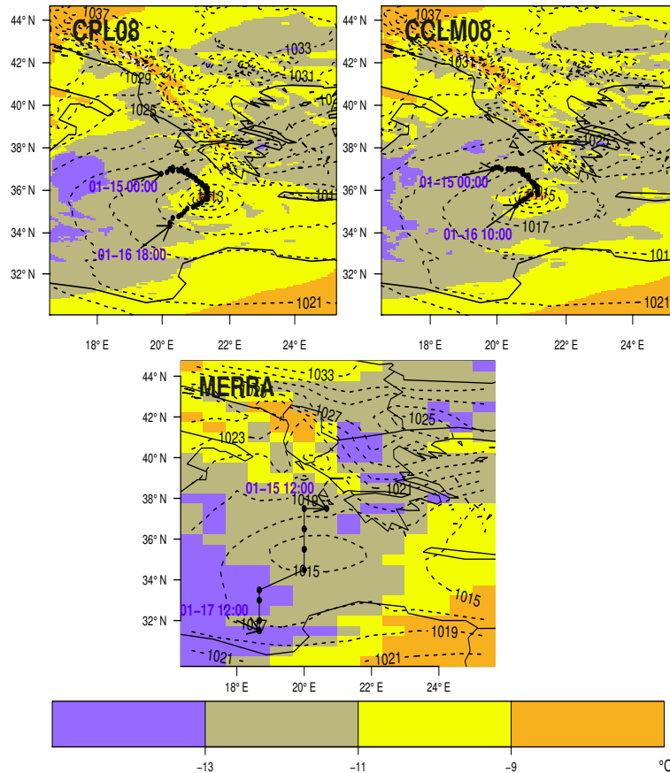
Fig. 8. ME06; mean sea level pressure (hPa; dotted contours lines at 2 hPa intervals) and temperature (°C: colored contours at 2°C intervals) at 700 hPa in coupled and atmosphere-only (0.08°) simulations and the MERRA reanalysis data on 16 January 1995 at 12:00 UTC.
