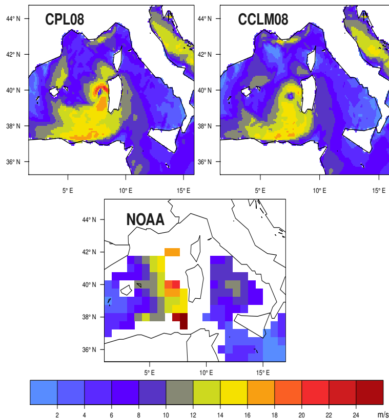
Fig. 7. ME09; 10 m wind speed ( \text{ms}^{-1} ) in coupled and atmosphere-only ( 0.08^\circ ) simulations and the NOAA “Blended Sea winds” on 10 December 1996 at 18:00 UTC.
