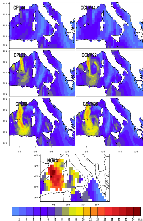
Fig. 3. ME08; 10 m wind speed ( \text{ms}^{-1} ) in coupled and atmosphere-only ( 0.44^\circ , 0.22^\circ , and 0.08^\circ ) simulations and the NOAA “Blended Sea winds” on 7 October 1996 at 18:00 UTC.
