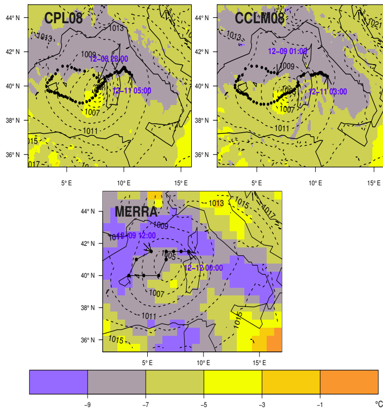
Fig. 6. ME09; mean sea level pressure (hPa; dotted contours lines at 2 hPa intervals) and temperature (°C: colored contours at 2°C intervals) at 700 hPa in coupled and atmosphere-only (0.08°) simulations and the MERRA reanalysis data on 10 December 1996 at 18:00 UTC.
