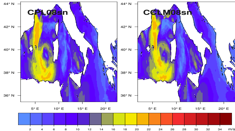
Fig. 5. ME08; 10 m wind speed ( \text{ms}^{-1} ) in coupled and atmosphere-only ( 0.08^\circ ) with spectral nudging simulations, on 7 October 1996 at 18:00 UTC.
