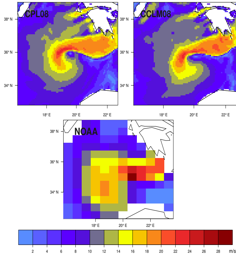
Fig. 11. ME10; 10 m wind speed ( \text{ms}^{-1} ) in coupled and atmosphere-only ( 0.08^\circ ) simulations and the NOAA “Blended Sea winds” on 27 January 1998 at 00:00 UTC.
