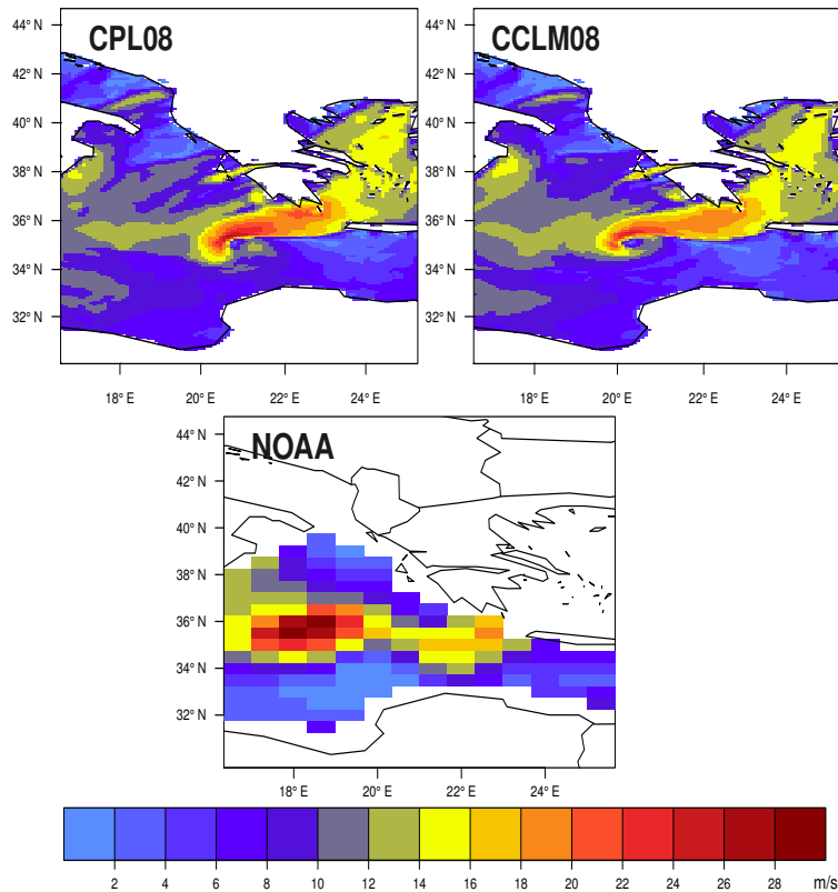
Fig. 9. ME06; 10 m wind speed ( \text{ms}^{-1} ) in coupled and atmosphere-only ( 0.08^\circ ) simulations and the NOAA “Blended Sea winds” on 16 January 1995, at 12:00 UTC.
