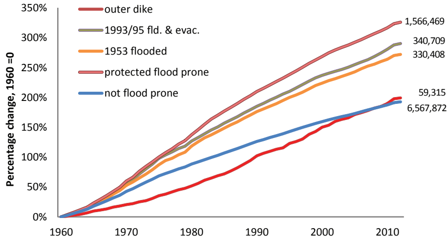
Fig. 2. Relative changes in the number of exposed properties per hazard zone, between 1960 and 2012. The absolute labels present the count of properties in each hazard zone in 2012.
