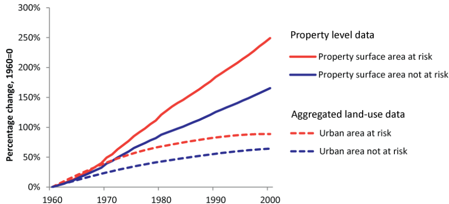
Fig. 3. Comparison of trends in property surface area, estimated using the property-level database, and aggregated data on historical urban land-cover (Knol et al., 2004). The figure shows that while the total urban area has stabilized over time, the property area at risk shows a continuous increase. This demonstrates that risk analysis using aggregated land-use information does not account for increases in urban density and thus might underestimate trends in exposure.
