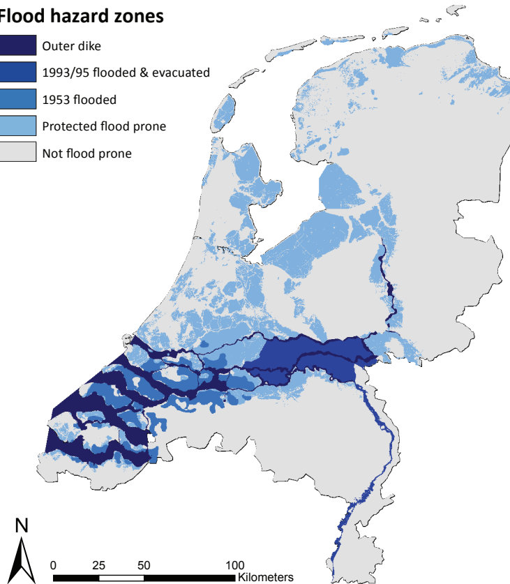
Fig. 1. Map of the flood hazard zones. Note that there is a slight overlap between some of the hazard zones, in which case the area is assigned to the hazard zone with the lowest number (see Table 1).
