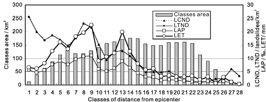
Fig. 24. Relationship of co-seismic landslides and distance from epicenter. 28 classes were divided according to 2 km intervals from the epicenter.
