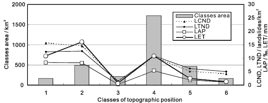
Fig. 21. Relationships between co-seismic landslides and topographic position. 1: Valleys, 2: lower slopes, 3: gentle slopes, 4: steep slopes, 5: upper slopes, and 6: ridges.
