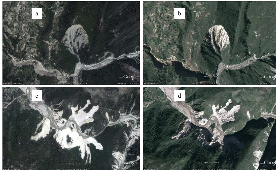
Fig. 3. Pre-earthquake landslides are shown in two locations. (a) and (b) is located at 18^{\circ}29'02.70'' N, 72^{\circ}11'22.28'' W; (c) and (d) is located at 18^{\circ}29'46.48'' N, 72^{\circ}11'37.86'' W. Images (a) and (c) were taken on 10 May 2008 and (b) and (d) were taken on 13 January 2010.
