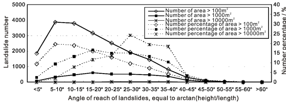
Fig. 16. Landslide angle of reach [ \arctan(\text{height}/\text{length}) ] distribution.
