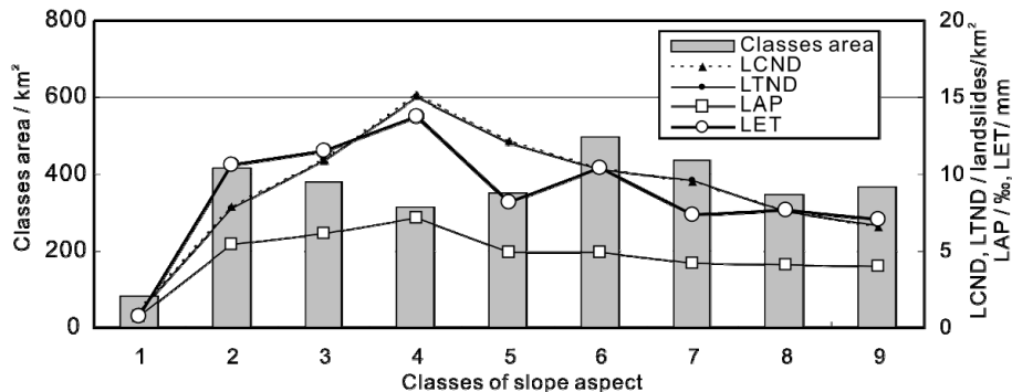
Fig. 19. Relationships of co-seismic landslide abundance with slope aspect. 1: Flat, 2: north, 3: northeast, 4: east, 5: southeast 6: south, 7: southwest, 8: west, and 9: northwest.
