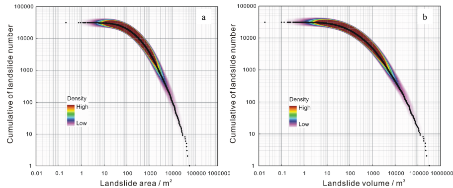
Fig. 13. Correlations between cumulative landslide number and landslide scale. (a) Landslide area, (b) landslide volume.
