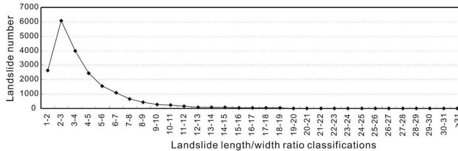
Fig. 14. Landslide length/width ratio distribution.
