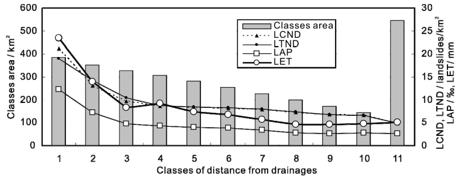
Fig. 22. Relationships of co-seismic landslides and distance from drainages. 1: 0–100 m, 2: 100–200 m, 3: 200–300 m, 4: 300–400 m, 5: 400–500 m, 6: 500–600 m, 7: 600–700 m, 8: 700–800 m, 9: 800–900 m, 10: 900–1000 m, and 11: > 1000 m.
