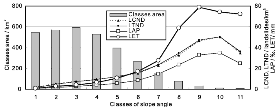
Fig. 18. Relationships of co-seismic landslide abundances with slope angles. 1: 0–5°, 2: 5–10°, 3: 10–15°, 4: 15–20°, 5: 20–25°, 6: 25–30°, 7: 30–35°, 8: 35–40°, 9: 40–45°, 10: 45–50°, 11: 50–75.83°.
