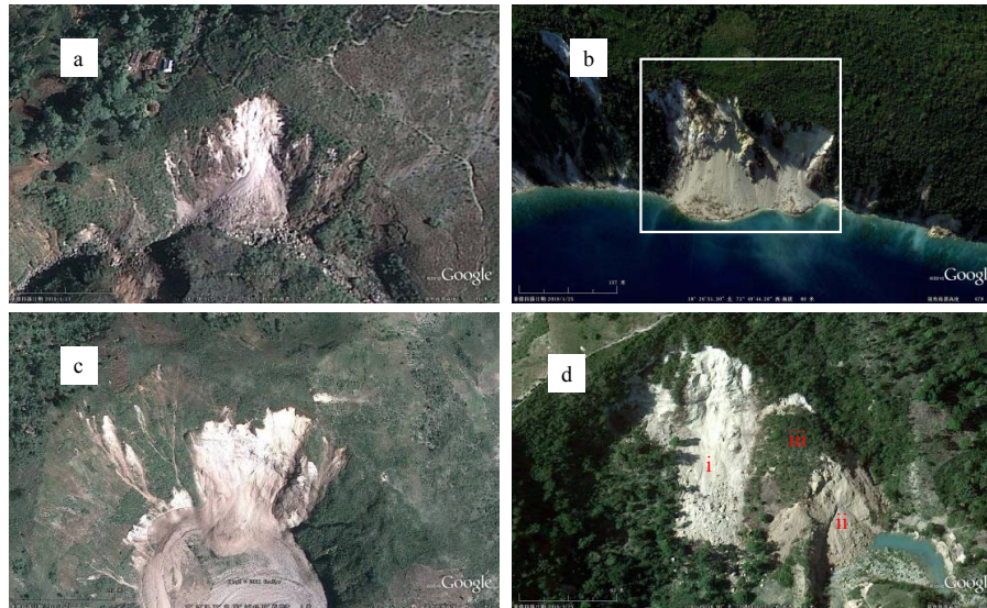
Fig. 8. (a) and (b) are two rock falls occurred at (18^{\circ}28'07.75''\text{ N}, 72^{\circ}29'15.00''\text{ W}) and (18^{\circ}26'31.30''\text{ N}, 72^{\circ}49'44.20''\text{ W}) , respectively. (a) was taken on 13 January 2010 (upward is northeast) and (b) was taken on 25 January 2010 (upward is south). (c) is located at 18^{\circ}28'51.78''\text{ N}, 72^{\circ}26'42.00''\text{ W} , taken on 13 January 2010 and upward is north. (d) shows several rock falls at 18^{\circ}19'38.90''\text{ N}, 72^{\circ}40'01.32''\text{ W} , and the images was taken on 25 January 2010 (upward is west).
