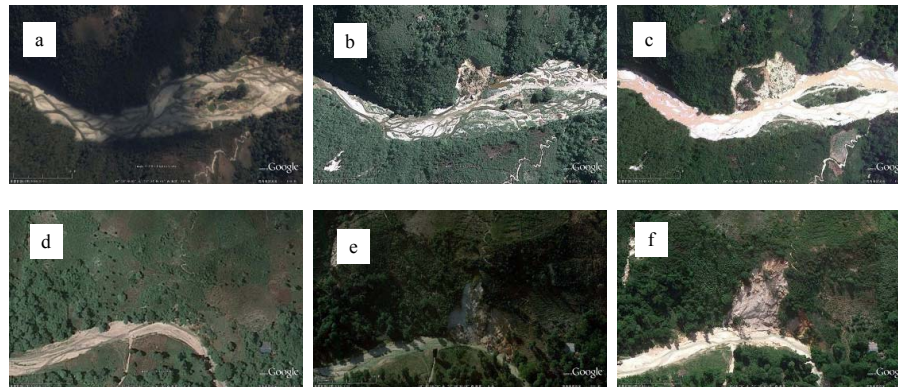
Fig. 5. Two places of co-seismic landslides probably enlarged by rainfall. (a), (b), and (c) are images showing a landslide located at 18^{\circ}29'40.75'' N, 72^{\circ}24'48.69'' W. The images were taken on 4 February 2009, 13 January 2010, and 9 November 2010, respectively. (d), (e), and (f) are images of a landslide located at 18^{\circ}30'58.78'' N, 72^{\circ}30'30.08'' W. The images were taken on 26 August 2009, 25 January 2010, and 9 November 2010, respectively.
