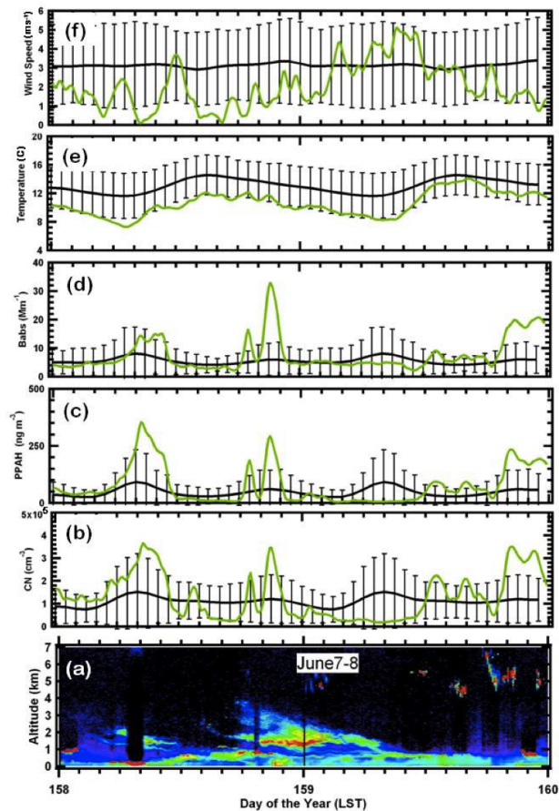
Fig. 2. Time series for June 7–8, 2011, a) the vertical profile of aerosol extinction coefficient, b) CN concentration, c) PPAH concentration, d) absorption coefficient, e) temperature and f) wind speed
