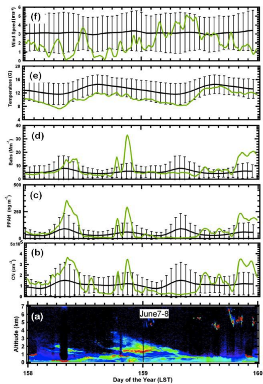
Fig. 2. Time series for June 7-8, 2011, a) the vertical profile of aerosol extinction coefficient, b) CN concentration, c) PPAH concentration, d) absorption coefficient, e) temperature and f) wind speed
