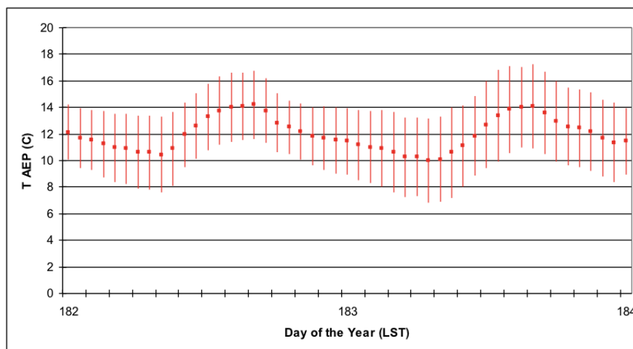
Fig. 1. Climatological diurnal evolution for 1 and 2 July at a nearby station (AEP) for our research site. The average values and one standard deviation (vertical bars) were estimated based on the period 1985
