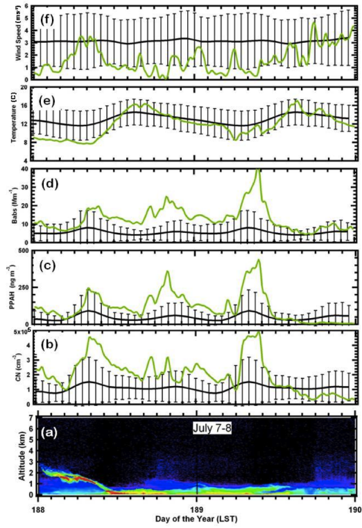
Fig. 4. Same as Fig. 2 but for the period July 7 and 8, 2011.
