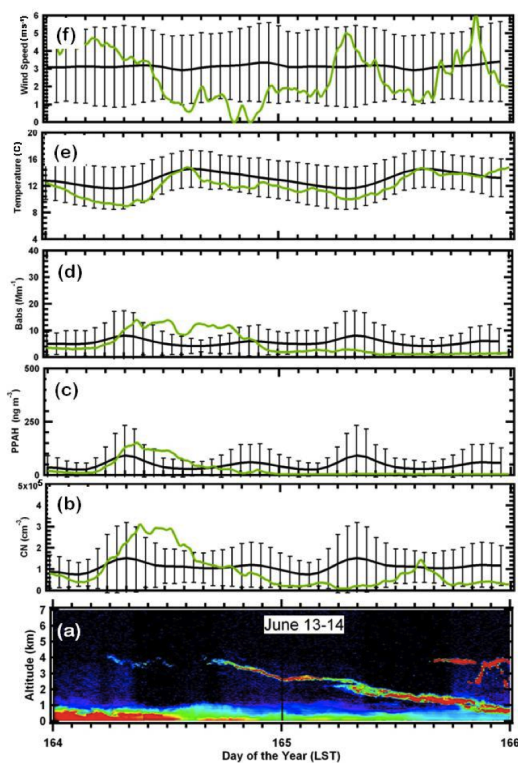
Fig. 3. Same as Fig. 2 but for June 13-14, 2011.
