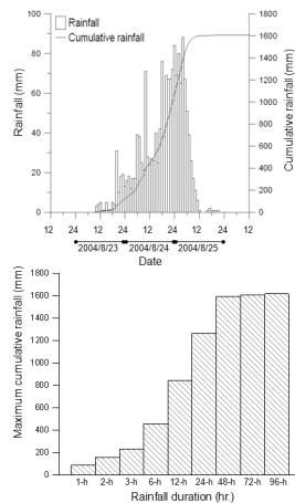
Figure 2. The temporal pattern of rainfall recorded from New Baishi station during Typhoon Aere.
