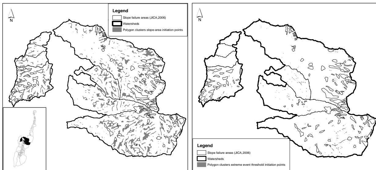
Fig 6. Comparison of the initiation points from the slope-area threshold and the extreme events threshold with photo-interpreted failure areas.
