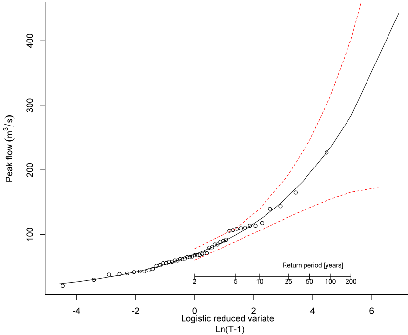
Fig. 4. GLO distribution fitted to the 49 AMAX events from the gauged record (1960-2010) at Lewes with confidence limits at the 95% level.
