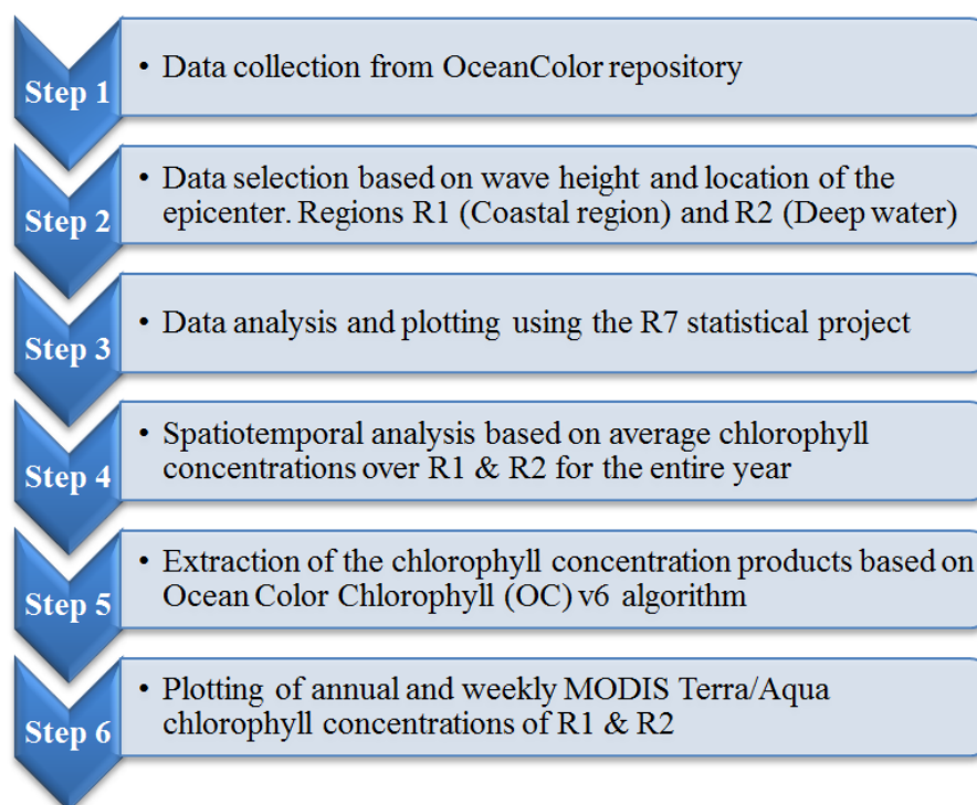
Fig. 1. An outline of steps taken when conducting the research and analyzing the data.
