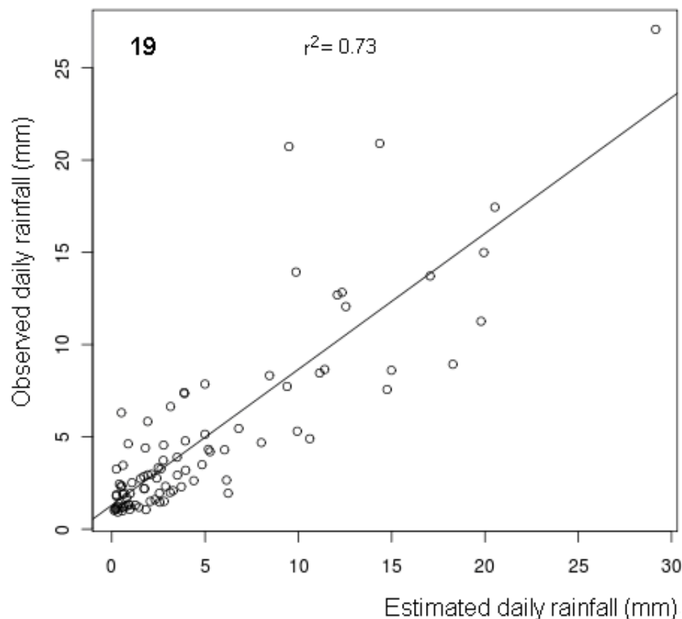
Fig. 7. Fig 8c. Comparing estimated and observed values of daily mean rainfall in the network (mm). Estimations are based on Eq. (2) with observatories number 22, 18 and 19 (marked in the upper-left side of e
