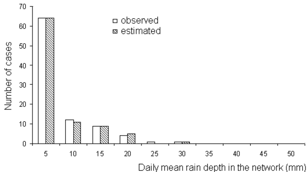
Fig. 8. Fig. 9. Frequency distribution of observed and estimated daily mean rain depth in the network (mm).
