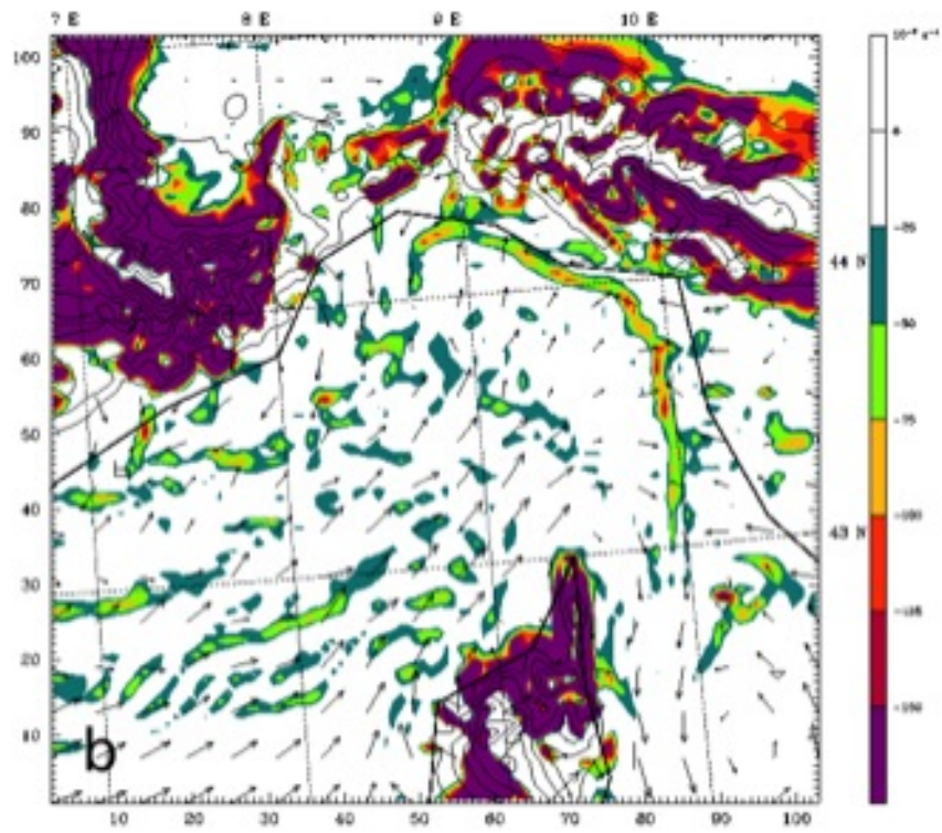
Fig. 2. Simulated negative divergence (convergence) at 03 UTC on 30 January 2008 for the GEN event.
