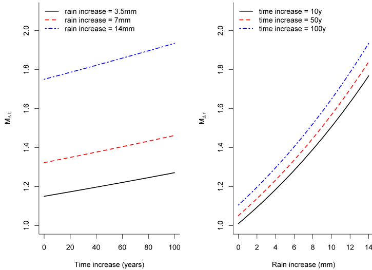
Fig. 7. Illustrative examples of magnification factors for river flows for different values of \Delta t and \Delta r , taking \beta_1 = 0.001 and \beta_2 = 0.045 .
