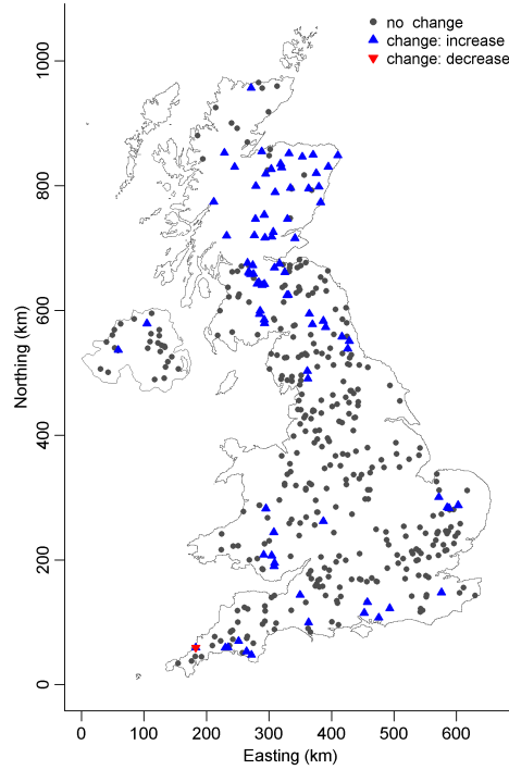
Fig. 6. Results for a Mann–Kendall test of no change in the annual series of the 99th quantile for daily rainfall. Significance tested at a \alpha_{\text{MK}} = 0.05 level.
