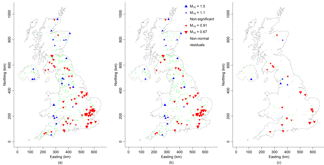
Fig. 11. Estimated decadal magnification factor M_{10} for model (c) for all the available series (left panel), for series with non-natural flow (central panel) and for series with nearly-natural flow (right panel) - summer maxima series.
