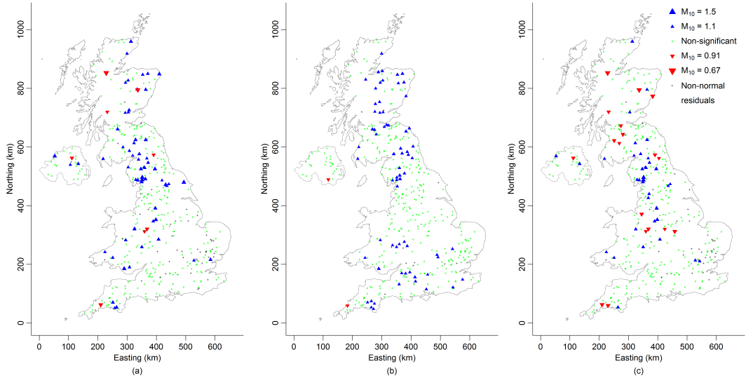
Fig. 9. Estimated decadal magnification factor M_{10} for model (a) for peak flow maxima with time as the only explanatory variable, (b) for daily rainfall maxima with time as the only explanatory variable and (c) for peak flow maxima with time and the 99th quantile of daily rainfall as explanatory variables – winter maxima series.
