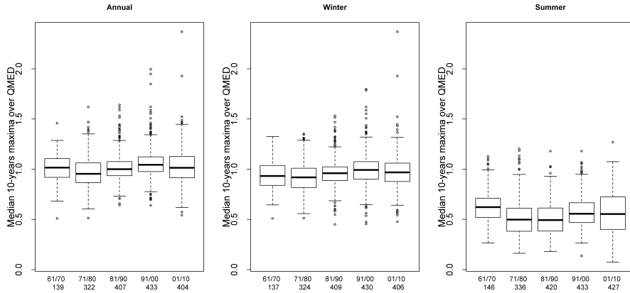
Fig. 3. Median ratio of annual and seasonal maximum peak river flow over long-term median of the annual maximum, shown separately for each decade. The number of stations with at least 7 years of data used to compute the proportions is indicated below the x -axis.
