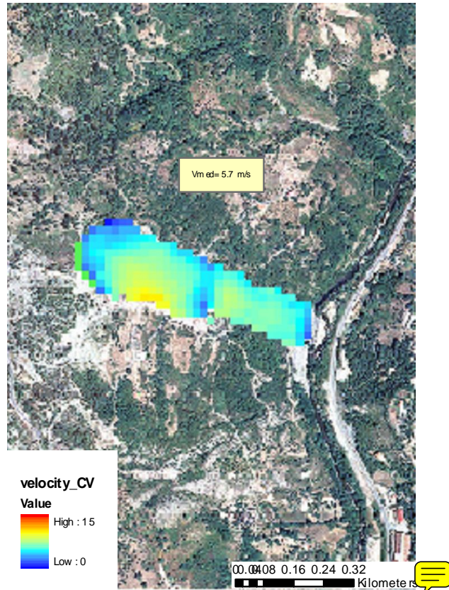
Fig. 7. Back analysis of the 1997 earth-flow using dfwalk model and rheological approach.
