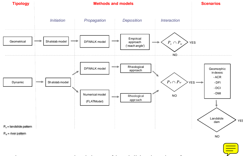
Fig. 5. Hazard assessment methodology of landslide-river interference.
