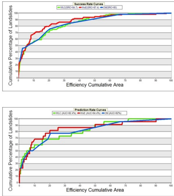
Fig. 3. The Areas Under Curves, using 22 independent landslides (i.e. 20% of the landslides inventory).
