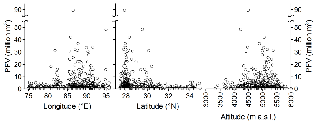
Fig. 1. PFV against lake locations
