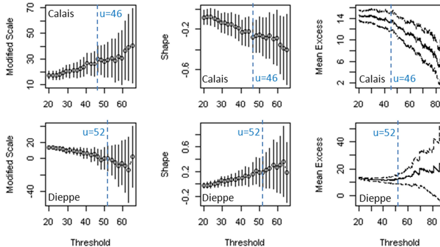
Fig. 3. Estimation of u (the threshold): the GPD modified scale and shape parameters and mean excess life plot with 95 % confidence intervals (Calais and Dieppe sites).
