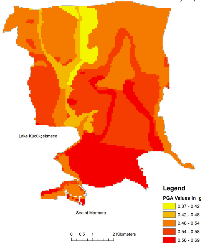
Fig. 7. PGA earthquake hazard map of Küçükçekmece district.
