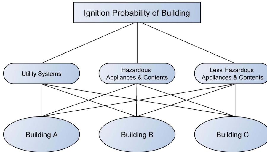
Fig. 4. Structure of AHP for post-earthquake ignition.
