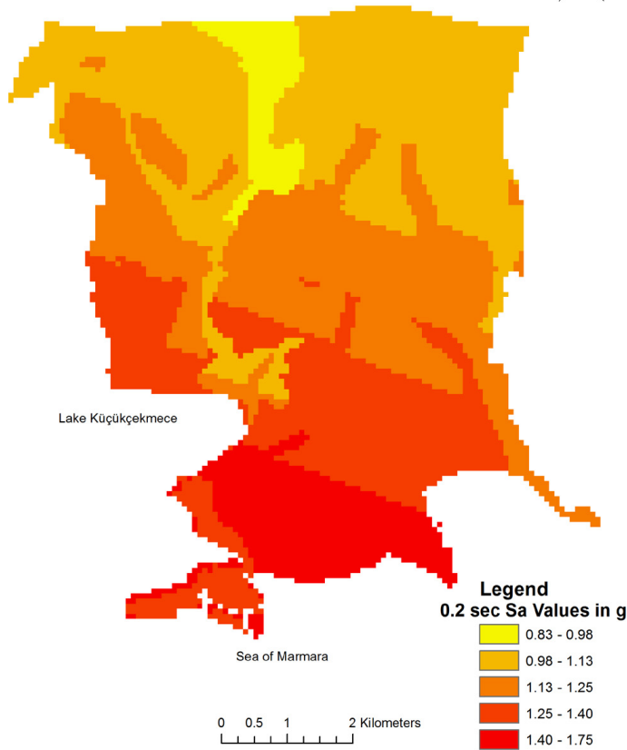
Fig. 6. 0.2 s S_a earthquake hazard map of Küçükçekmece district.
