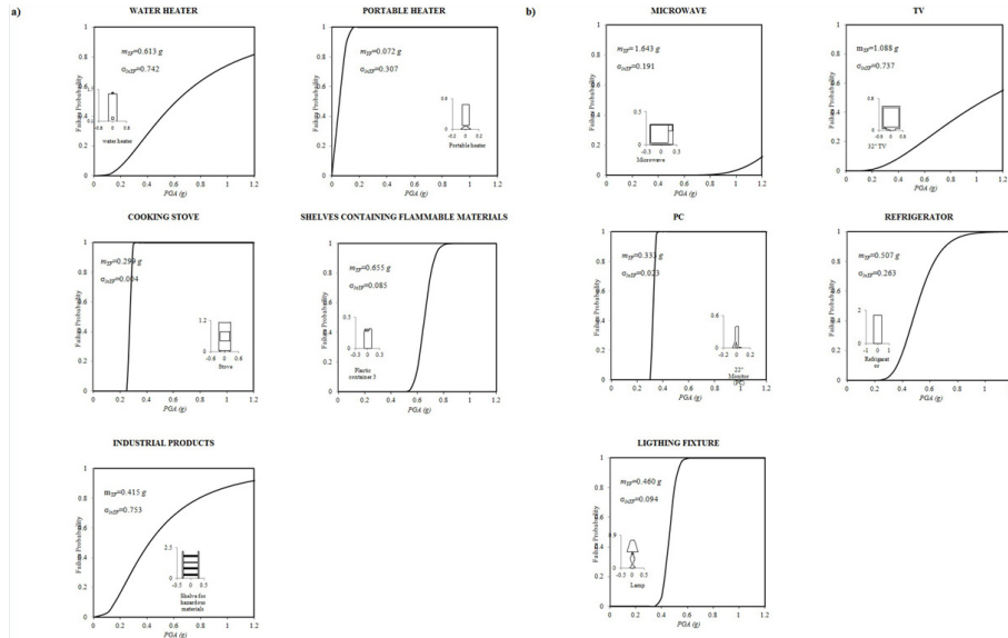
Fig. 3. Overturning probability for (a) hazardous appliances and (b) less hazardous appliances (Reinoso et al., 2010).
