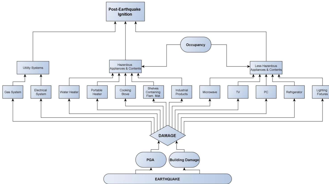
Fig. 1. Structure of post-earthquake ignition model.
