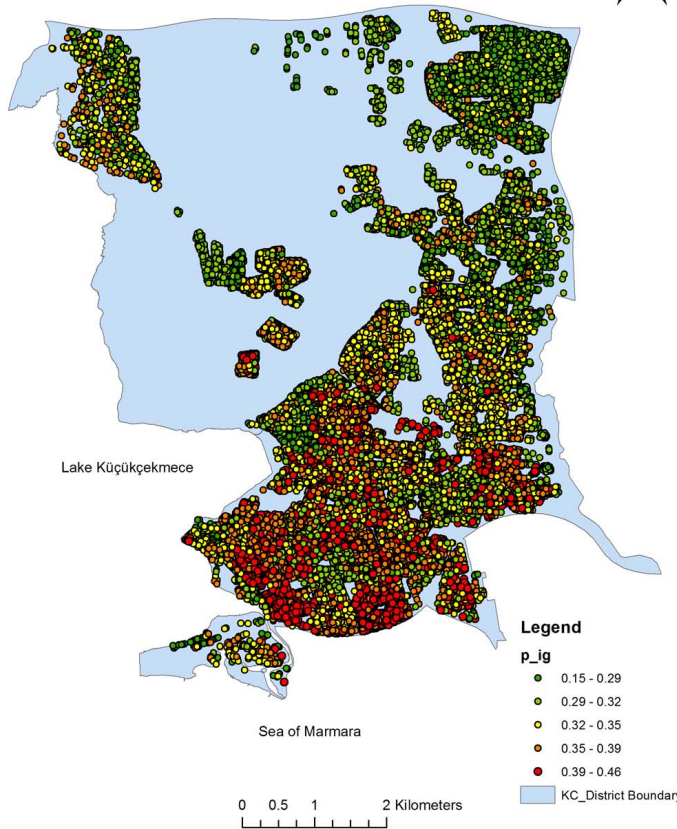
Fig. 9. Visualized results of post-earthquake ignition analysis.
