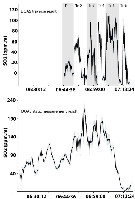
Fig. 4. Plots of traverse (above) and static (below) measurement results obtained on Papandayan. Time axis were aligned highlighting the increase of SO 2 column amounts in both static and traverse measurements.
