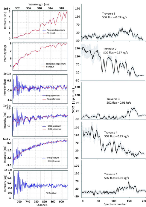
Fig. 5. Example of DOAS SO 2 fit on Bromo (left). Measurement spectra are blue. Traverse measurement profiles (right). Traverses 1, 3 and 5 did not catch the bulk concentration while traverses 2 and 4 commenced in the plume (see text).
