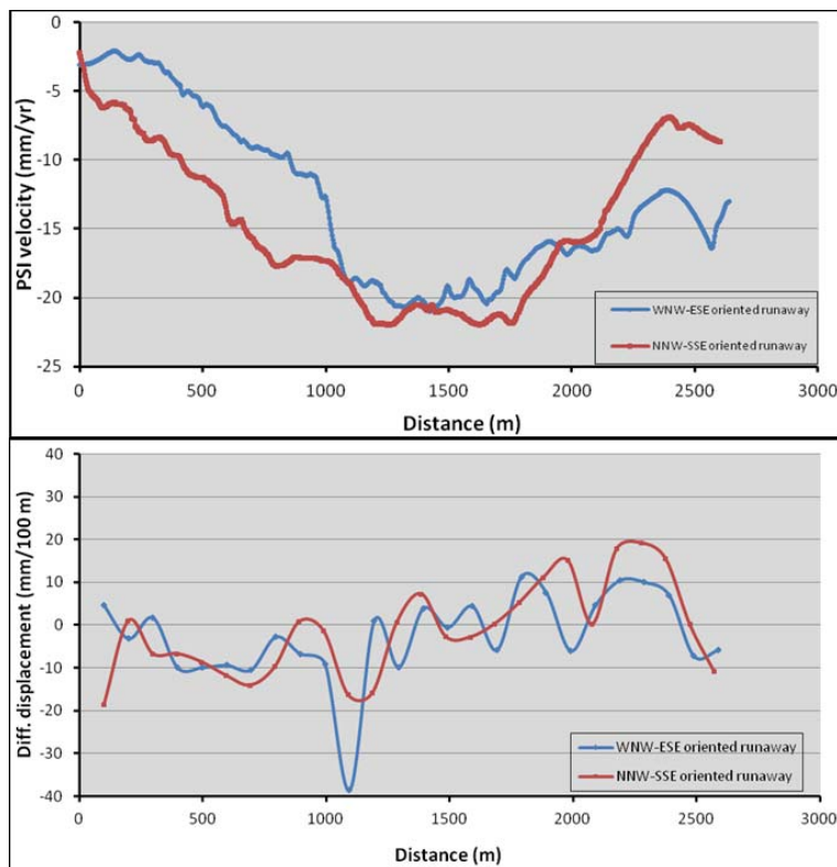
Fig. 8. Vertical deformation ( V_v ) of the LOS velocities measured along the runway areas of the Thessaloniki airport (above). Differential displacement along the runways area (below). Origin is set on the coastline.
