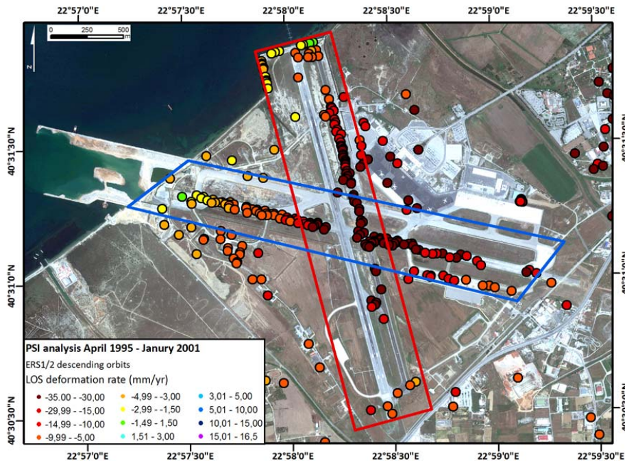
Fig. 7. LOS velocity map along the runway areas of “Macedonia” Airport. PSs inside the buffer zones have been extracted and analyzed to evaluate differential settlement.
