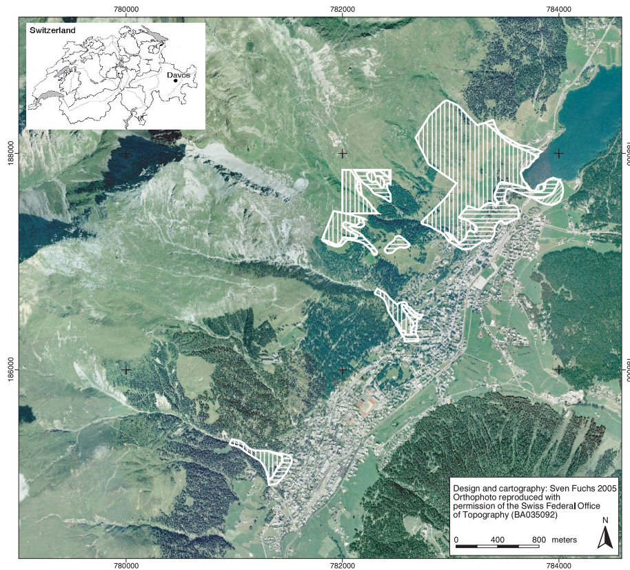
Fig. 1. Study area in the municipality of Davos. The hatched raster represents the avalanche run-out areas (scenario 2000 ). Vertical hatching corresponds to the red hazard zone (30-year scenario), horizontal hatching to the blue hazard zone (300-year scenario), and angular hatching to the yellow hazard zone (run-out area of powder snow avalanches). For explanations regarding hazard zoning in Switzerland, see the Appendix.
