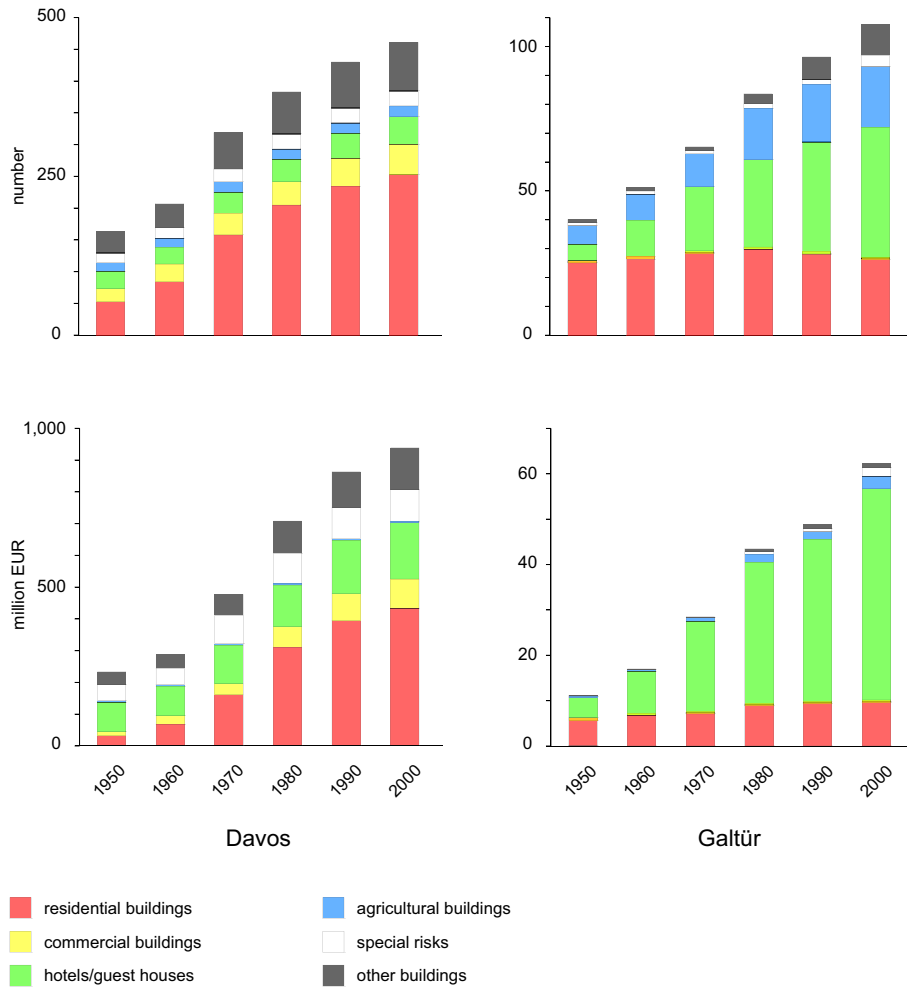
Fig. 3. Development of damage potential in Davos (CH) and Galtür (A) related to the respective avalanche-prone areas, subdivided in decades and building functions.
