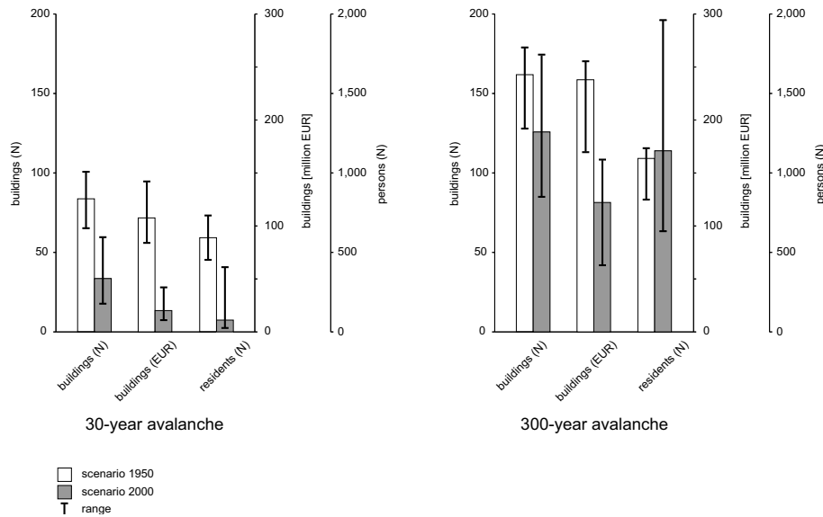
Fig. 2. Scenario 1950 and scenario 2000 resulting from 30-year and 300-year avalanche events in the municipality of Davos (CH), and associated uncertainties following the suggestions outlined in Barbolini et al. (2002). For the 30-year scenario, the ranges regarding the buildings are relatively similar, while the range resulting from the residents in the year 2000 is remarkably high. For the 300-year scenario in the year 2000, the highest range occurred within the category of endangered residential population, while the lowest variations were found for the number of buildings.
