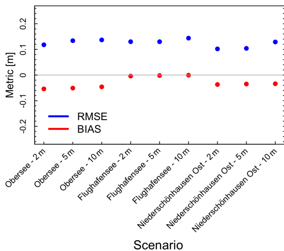
Figure 7. Comparison of RIM2D-simulated water depths with official city flood maps at spatial resolutions of 2, 5, and 10 m for a 100-year flood event in the Obersee, Flughafensee, and Niederschönhausen Ost catchments. Evaluation metrics include Root Mean Square Error (RMSE) and Bias.
