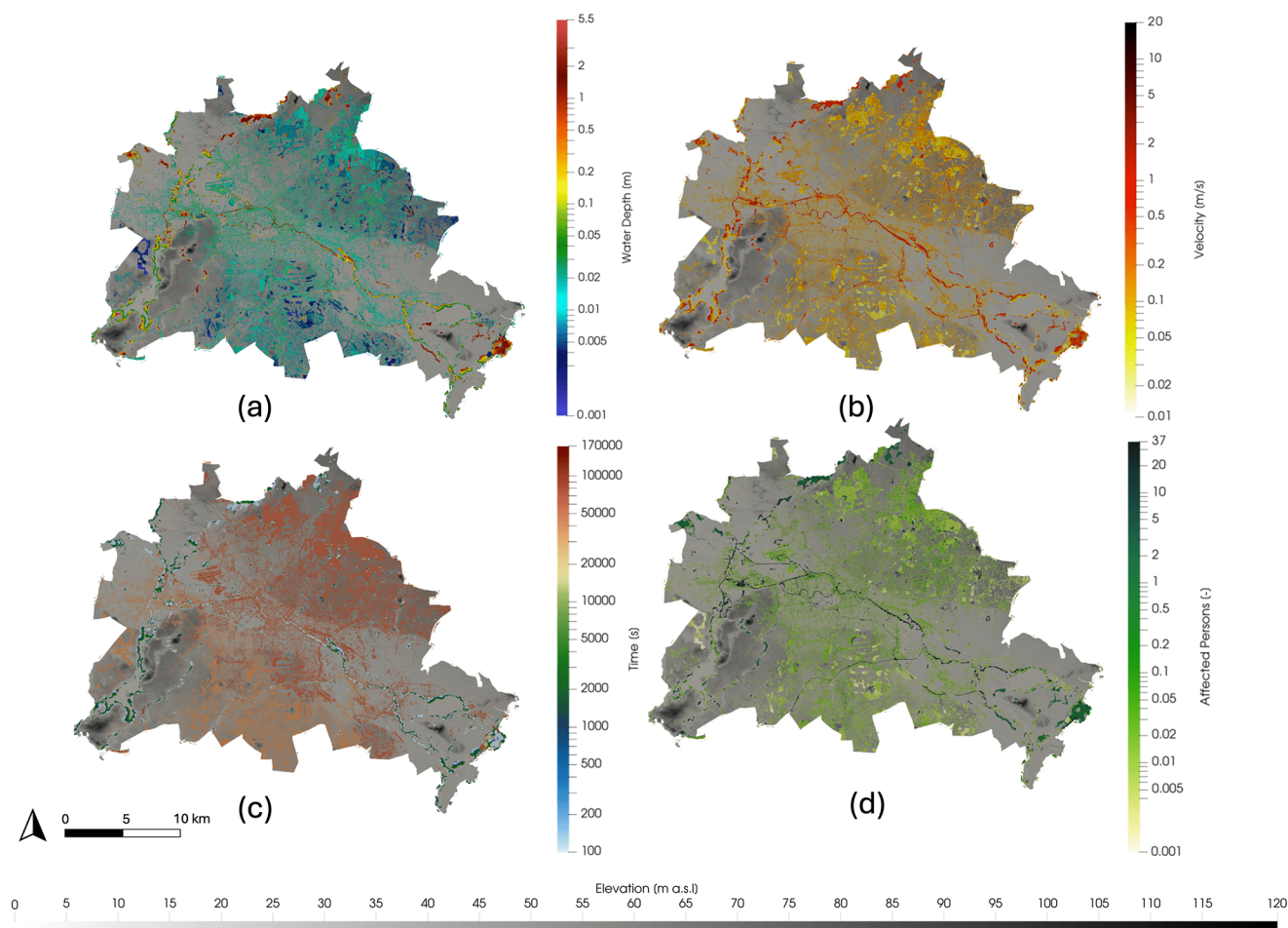
Figure 8. (a) Simulated max water depths [m], (b) max velocities [ \text{m s}^{-1} ], (c) time of max water depth [s] and (d) affected population [number of persons] for the June 2017 flood event at \text{dx} = 5 \text{ m} .
