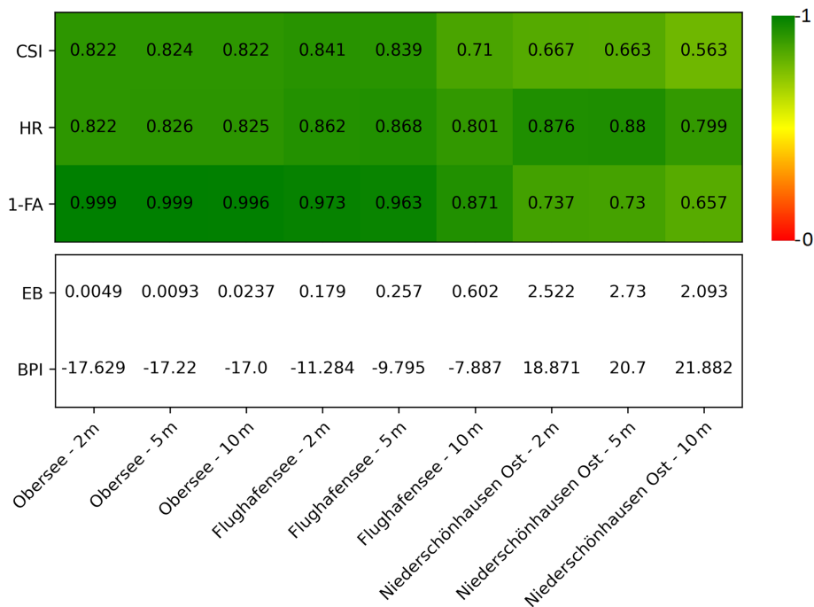
Figure 6. Comparison of RIM2D-simulated flooded areas with official city flood maps at spatial resolutions of 2, 5, and 10 m for a 100-year flood event in the Obersee, Flughafensee, and Niederschönhausen Ost catchments. Evaluation metrics include the Critical Success Index, Hit Rate, False Alarm Ratio, Error Bias, and Bias Percentage Indicator.
