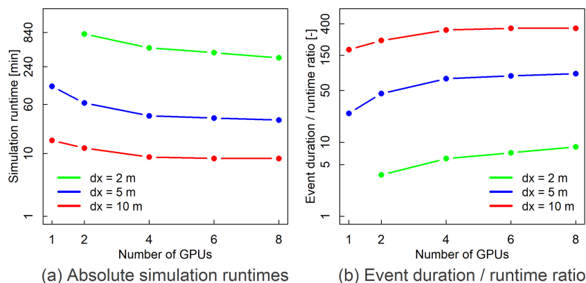
Figure 2. (a) Absolute simulation runtimes and (b) the ratio of simulation duration to runtime for dx = 10, 5 , and 2 m resolutions during the June 2017 flood event (48 h simulation), using 1, 2, 4, 6, and 8 GPU configurations.
