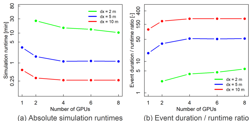
Figure 3. (a) Absolute simulation runtimes and (b) the ratio of simulation duration to runtime for dx = 10, 5 , and 2 m resolutions for the HQ100 scenario (1 h simulation), using 1, 2, 4, 6, and 8 GPU configurations.
