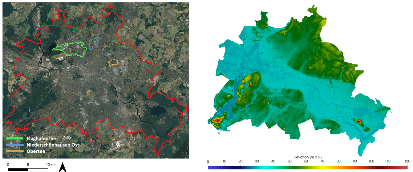
Figure 1. The red line in the left figure marks the administrative boundary of Berlin (Senatsverwaltung für Stadtentwicklung, Bauen und Wohnen Berlin, 2022) and also the boundary of our simulations domain. The catchments Obersee (orange line), Flughafensee (green line) and Niederschönhausen Ost (blue line), defined by the city administration for the creation of pluvial hazard maps are also displayed. The right figure depicts the topography of the city. Imagery © 2025 Landsat/Copernicus, Map data © 2025 Google.
