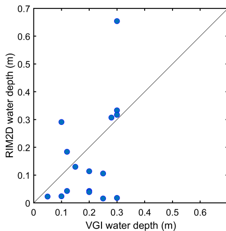
Figure 5. Validation of the \Delta x = 5 m June 2017 flood RIM2D simulation water depths at 16 VGI validation locations in Berlin using measured water marks. The figure shows RIM2D simulated water depths compared to estimated VGI water depths derived from field measurements.
