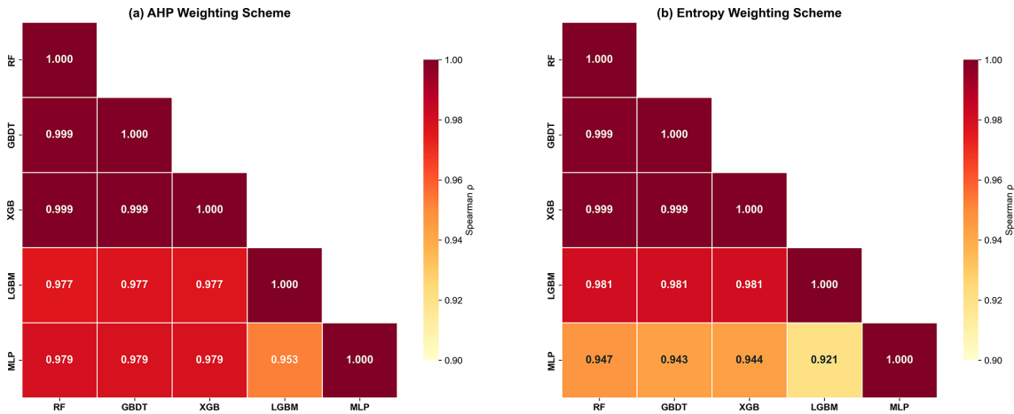
Figure 3. Correlation matrix of severity rankings across five machine learning models using AHP and Entropy Weight methods, highlighting the average Spearman rank correlation coefficient
