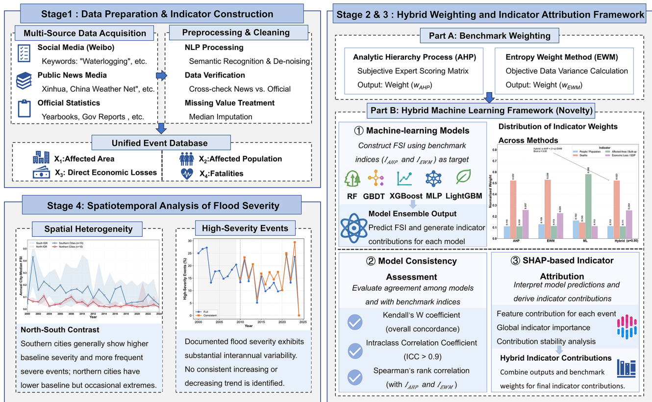
Figure 2. Flowchart of the hybrid machine learning-based weighting framework.
