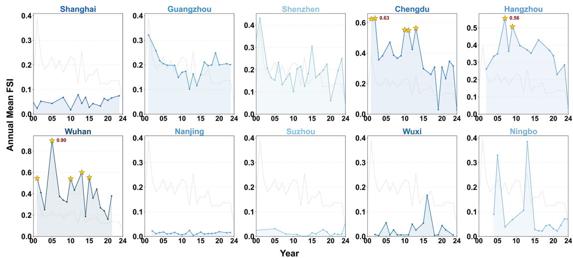
Figure 9. Temporal trends of annual mean flood-event severity in southern cities during 2000–2024.
