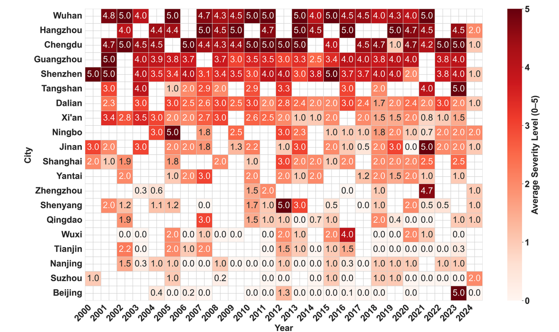
Figure 8. Spatiotemporal distribution of documented flood-event severity across the 20 cities during 2000–2024.
