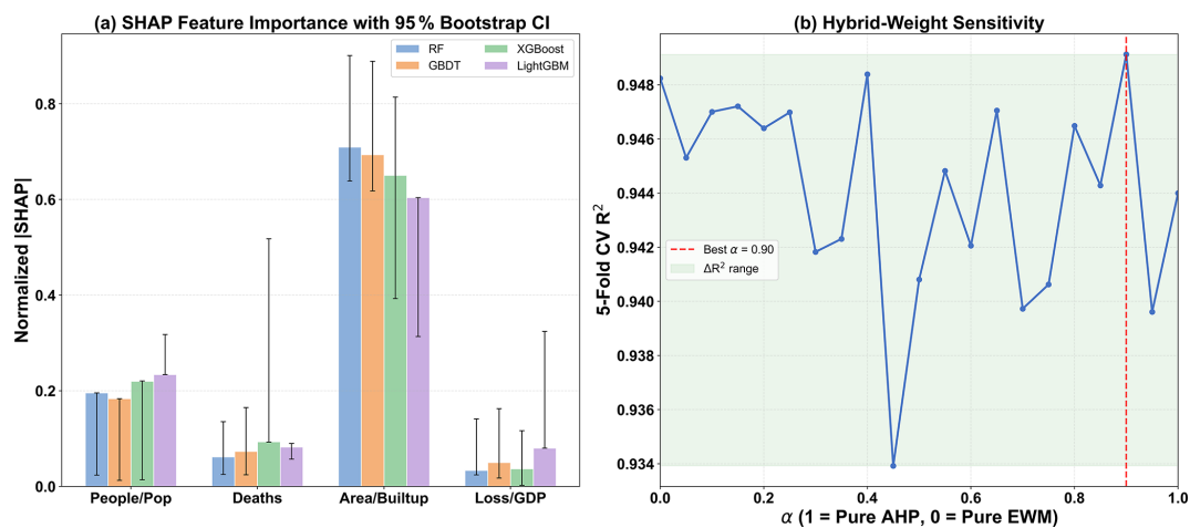
Figure 4. Recommended presentation: (a) normalized out-of-fold SHAP contributions with bootstrap intervals; (b) hybrid-weight sensitivity across \alpha .
