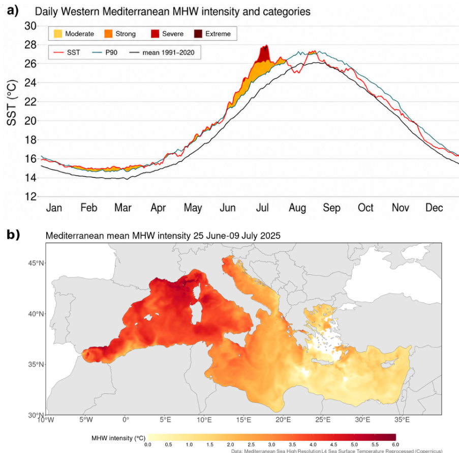
Figure 1. (a) Daily SST averaged over the Western Mediterranean Sea for 2025 (red), together with the 1991–2020 daily climatological mean (black line) and the 90th percentile MHW threshold (P90, teal line). Shading indicates the MHW category (moderate, strong, severe, extreme) following Hobday et al. (2016, 2018). (b) Mean MHW intensity (temperature anomaly above the 1991–2020 climatology, in °C) over the Mediterranean Sea for the 25 June–9 July 2025 period, i.e. the most intense (severe category) phase highlighted in panel (a). White areas over the sea are grid points where no MHW was detected. SST data obtained from the Mediterranean Sea-High Resolution L4 Sea Surface Temperature Reprocessed (MED-REP-L4) dataset from Copernicus.
