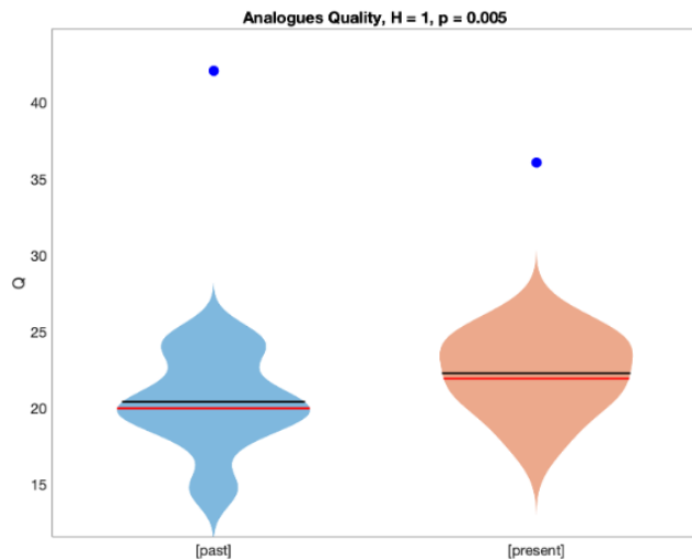
Figure 4. Analogue quality scores ( Q ) for the analogue dates selected in the past (1950–1986, blue) and present (1987–2024, orange) periods. Violin plots show the distribution of mean Euclidean distances between 42 analogue SST patterns and randomly selected JJAS days from the same period. The horizontal red and black lines indicate the mean and median of each distribution, respectively. The filled blue dots mark the actual Q values computed between the target 2025 SST event and its selected analogues. A lower Q indicates a better match. The statistical difference between past and present distributions is confirmed by a two-tailed Cramér–von Mises test ( p = 0.005 ).
