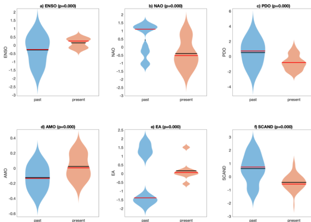
Figure 3. Violin plots comparing the distributions of natural variability indices during analogue dates in the past (1950–1986, blue) and present (1987–2024, orange) periods. The indices include: (a) El Niño–Southern Oscillation (ENSO), (b) North Atlantic Oscillation (NAO), (c) Pacific Decadal Oscillation (PDO), (d) Atlantic Multidecadal Oscillation (AMO), (e) East Atlantic pattern (EA), and (f) Scandinavian pattern (SCAND). Each violin shows the full probability density of the distribution, with horizontal red and black lines indicating the mean and median, respectively. The width of the violin reflects the relative frequency of values. All comparisons yield statistically significant differences between past and present periods (two-tailed Cramér–von Mises test, p < 0.001 ), suggesting that the underlying state of large-scale climate modes has shifted over time.
