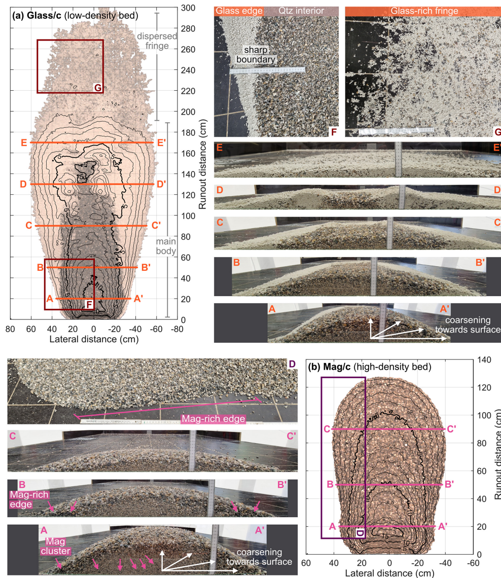
Figure 6. Internal structure and spatial distribution of the (a) Qtz–Glass and (b) Qtz–Mag deposit from coarse-particle experiments. Positions of lateral cross sections and surface views are indicated on the contoured surface scan. Contour lines are spaced at 1 cm intervals. Note that thicknesses in the cross sections may appear slightly reduced compared to the corresponding contour-plot position, as inserting the glass plate for vertical cutting could drag material downward at the front. Photographs are from Exp18 (Glass/c) and Exp19 (Mag/c).
