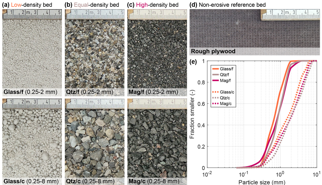
Figure 1. Materials used to establish the systematically imposed solid-particle-density contrast scenarios in the dry granular flow experiments. (a–c) Erodible bed materials with (a) expanded glass (Glass) for the low-density scenario, (b) quartz (Qtz) for the equal-density scenario, and (c) magnetite (Mag) for the high-density scenario. (d) Rough plywood used as rigid bed for a non-erosive reference. (e) Cumulative particle-size distributions. Note that Qtz/f and Qtz/c shown in (b) were also used as initial sliding material in the corresponding fine- or coarse-particle experiments. /f: fine particles; /c: coarse particles.
