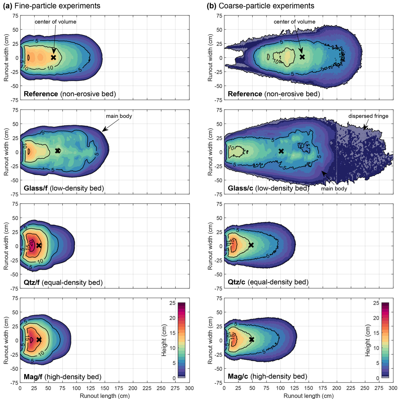
Figure 4. Deposit morphology of (a) fine- and (b) coarse-particle experiments. From top to bottom: contours of deposit height for the non-erosive reference, the glass bed, the quartz bed, and the magnetite bed. Representative runs are shown (see Sect. 2.4). Note that the flume was repositioned to the horizontal before deposit scanning. Therefore, only material deposited beyond the flume outlet was analyzed, and the apparent thickness drop towards (0|0) is a systematic artifact (see Fig. S5). /f: fine particles; /c: coarse particles.
