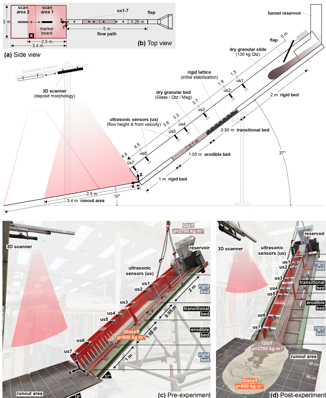
Figure 2. Experimental flume setup. (a) Side- and (b) top-view schematic. (c) Flume with planar erodible bed and filled reservoir before the experiment. (d) Deposit after the experiment. Flume sections and measurement positions are indicated. Photographs are from Exp5 (Glass/f).
