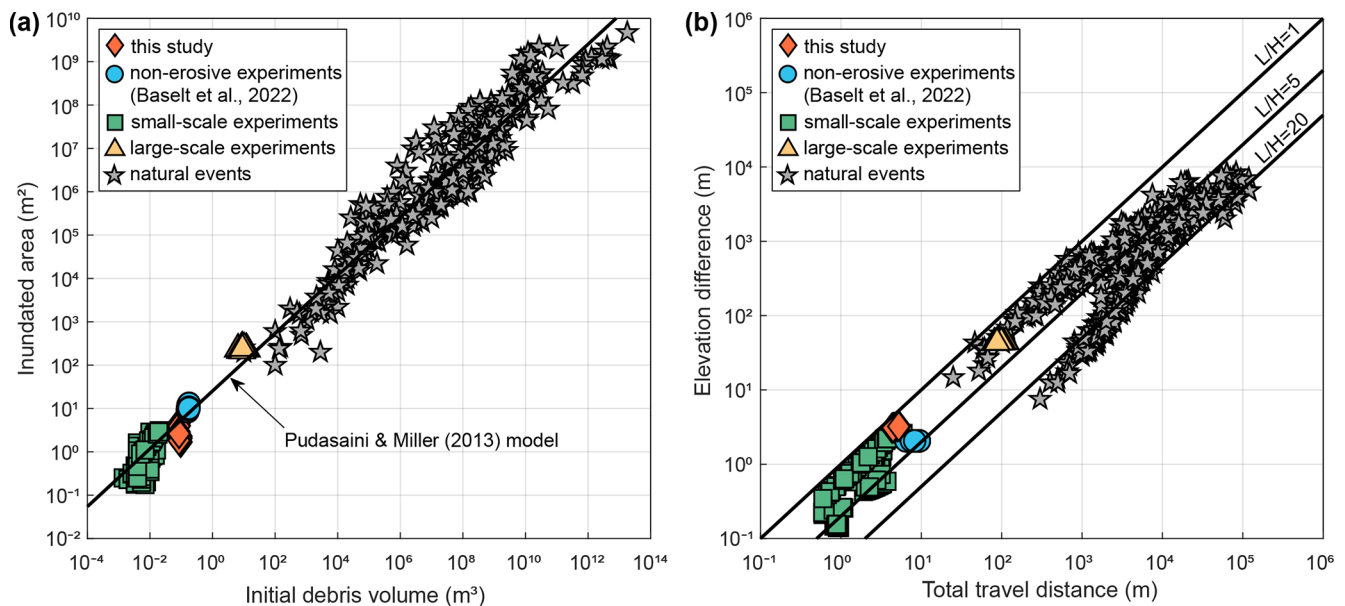
Figure 7. Evaluation of deposit geometry and mobility in comparison with other experiments and natural events. (a) Inundated area as a function of the initial debris volume and in comparison with the volume-area model by Pudasaini and Miller (2013) (volume-area slope S = 25 ). (b) Mobility expressed as elevation difference over total travel distance. The mobility reference lines represent typical values for natural events (figure modified and extended from Baselt et al., 2022).
