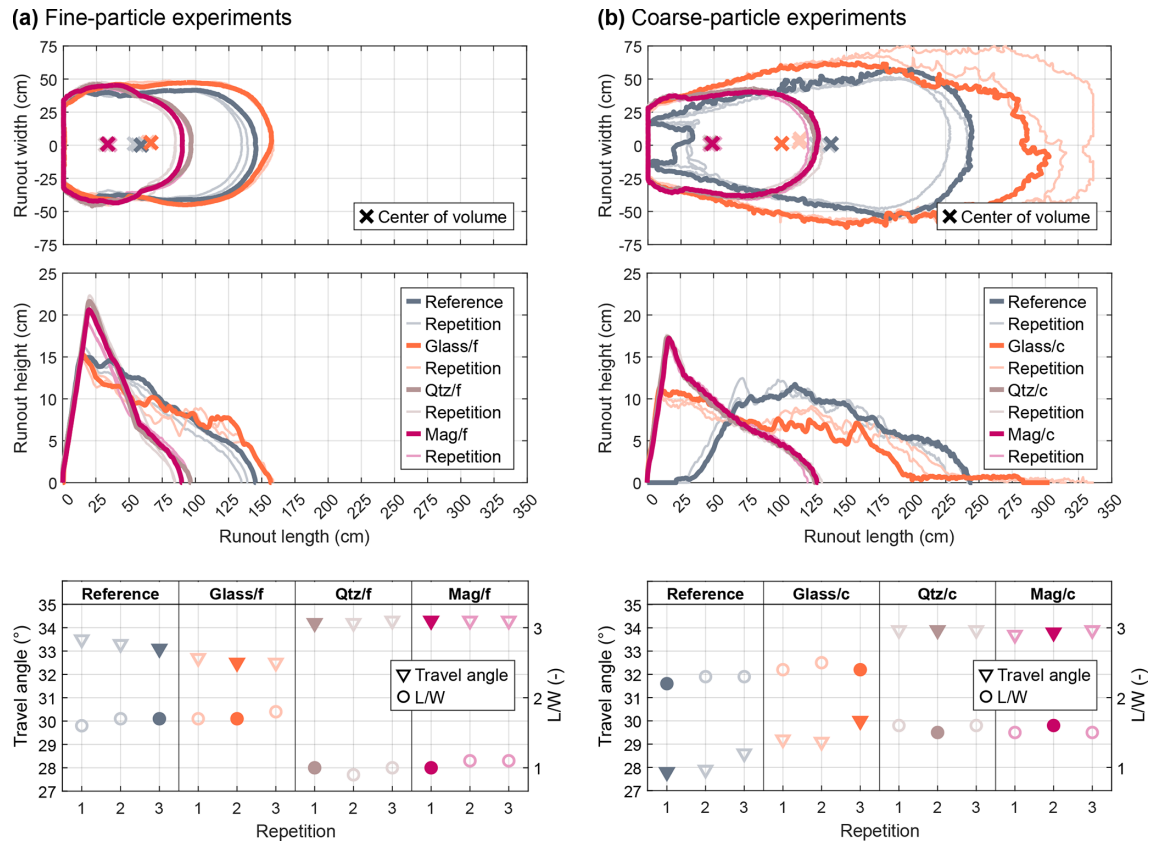
Figure 5. Deposit geometry and experimental reproducibility for (a) fine- and (b) coarse-particle experiments. From top to bottom: deposit outlines, downslope runout height along the central deposit line, as well as travel angle and L/W for all repetitions. Bold lines and filled symbols indicate the representative runs (see Sect. 2.4); thin lines or open symbols show their repetitions. /f: fine particles; /c: coarse particles; L/W : length-to-width ratio.
