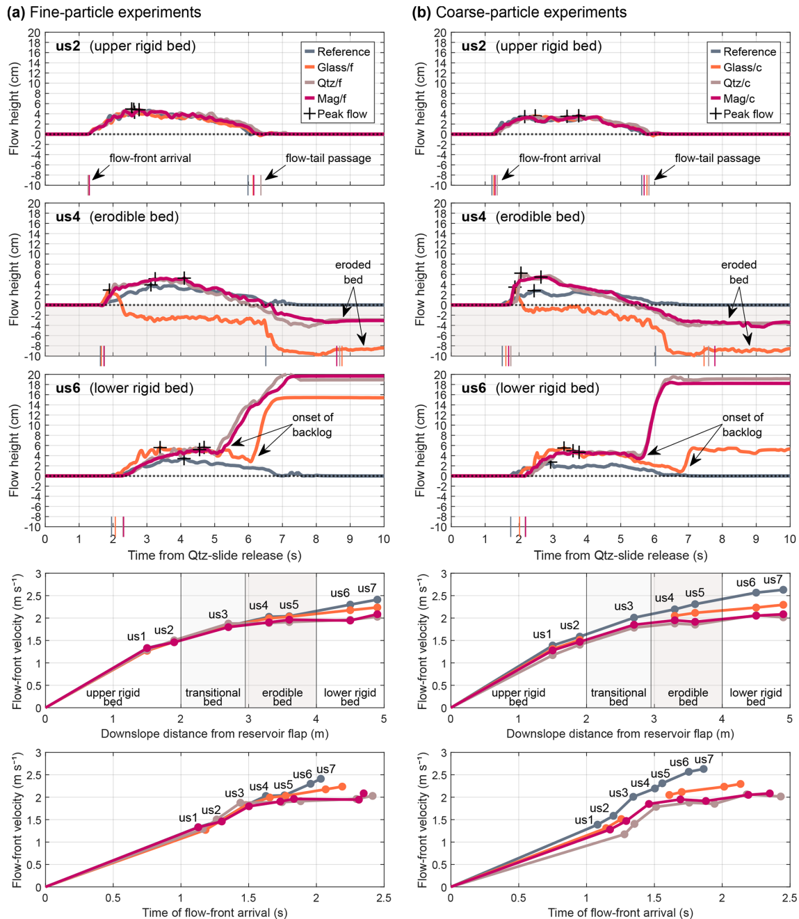
Figure 3. Spatiotemporal flow evolution of (a) fine- and (b) coarse-particle experiments. From top to bottom: evolution of flow height over time at us2 (before the erodible bed), us4 (on the erodible bed), and us6 (before the runout area), as well as average flow-front velocity from reservoir flap to sensor over downslope distance, and over time. Representative runs are shown (see Sect. 2.4). Note that in panel (b), no data point is shown at us3 for the Glass/c experiment in the two lower panels due to a brief ultrasonic signal loss during flow-front passage. /f: fine particles; /c: coarse particles; us: ultrasonic sensor.
