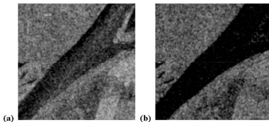
Figure 2. Comparison of different polarization images on the surface of roughened water bodies. Panel (a) shows VV polarization image. Panel (b) shows VH polarization image.
