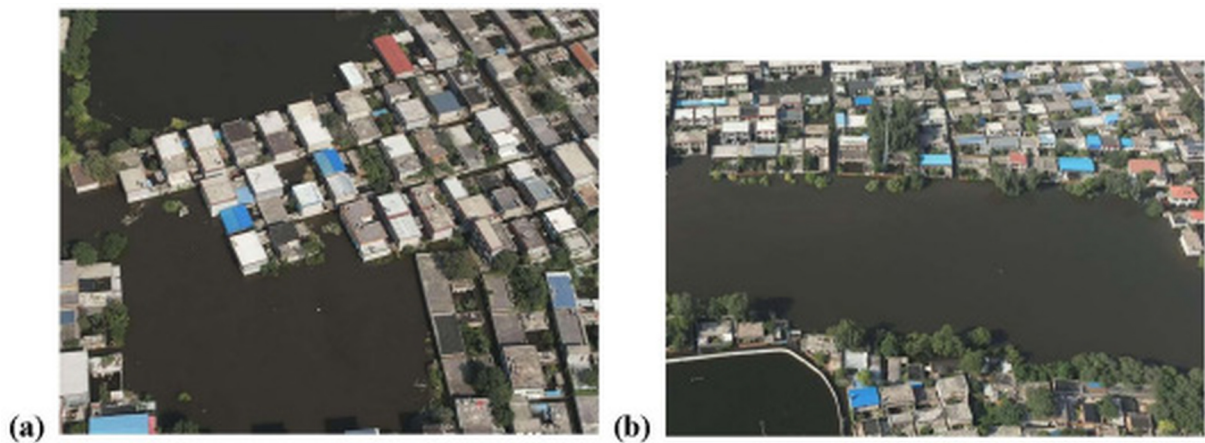
Figure 8. UAV optical images when floods occurred in Weiwei City. Panel (a) represents areas severely inundated by floods; panel (b) represents areas with moderate flood inundation. UAV image source: authors’ field survey.
