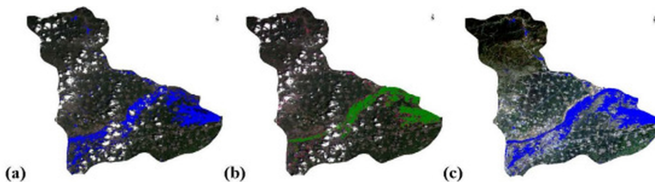
Figure 5. Comparison of monitoring results in the flood area of Weihui City based on the Z-score method. (a) 26 July 2021, (b) 27 July 2021, (c) 31 July 2021. The blue or green areas in the picture represent the areas affected by the flood.
