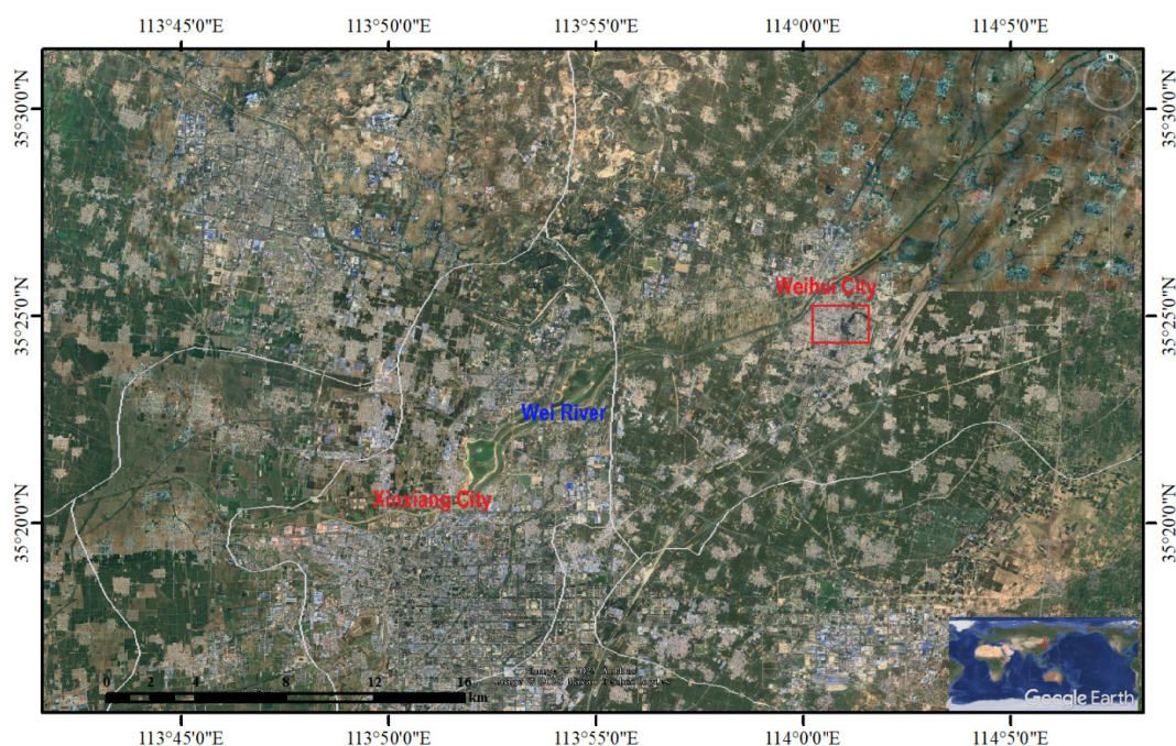
Figure 1. The geographical location of the study area (Map data © 2025 Google). The red box represents the UAV imaging coverage.
