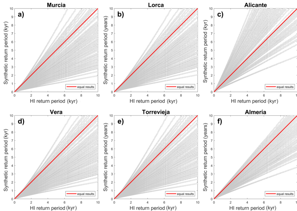
Figure 10. Comparison of the return periods obtained in the hazard curves for the synthetic scenarios and the historical-instrumental, HI, one (grey squares) in the cities of: (a) Murcia, (b) Lorca, (c) Alicante, (d) Vera, (e) Torrevieja and (f) Almería. The red line indicates the hypothetical scenario in which the results were identical for both datasets.
