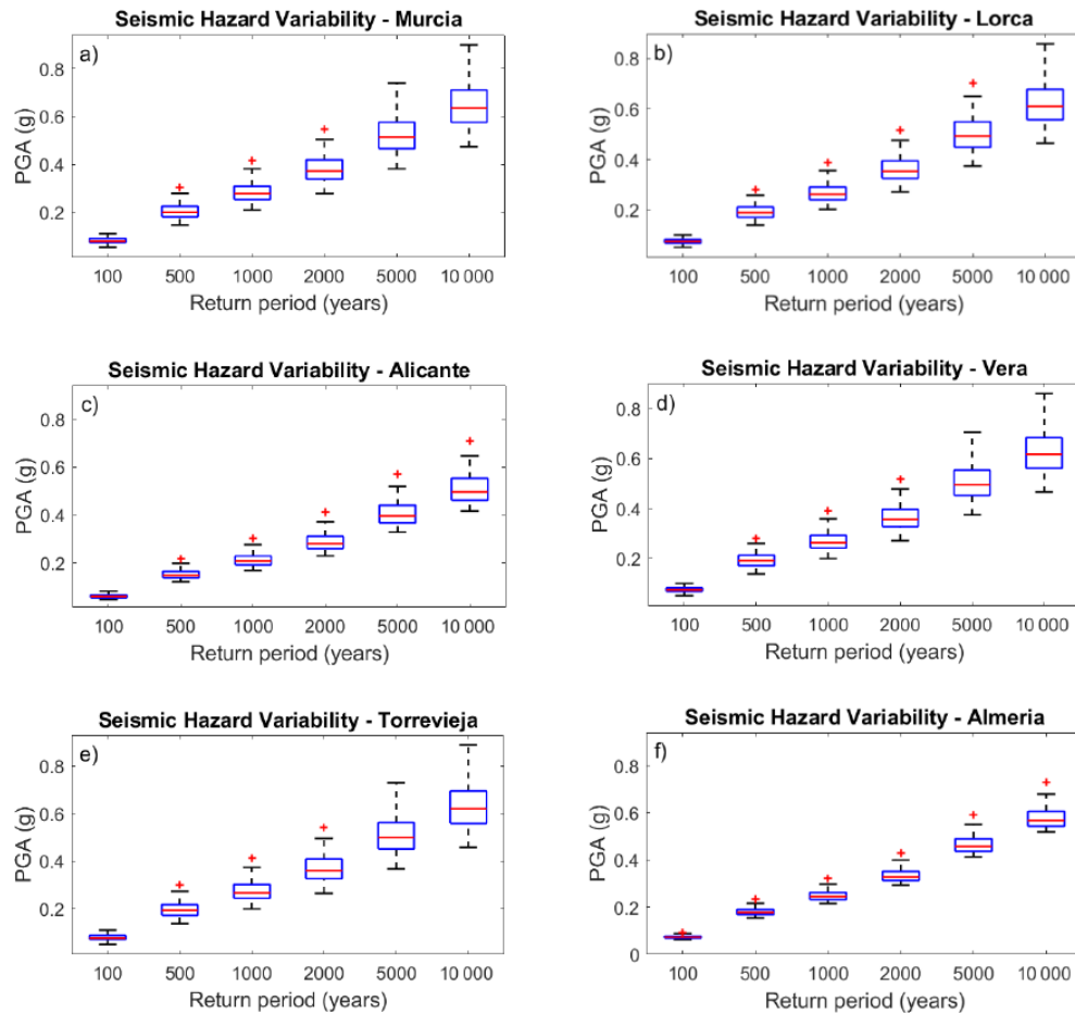
Figure 8. PGA variability for different return periods at the cities of (a) Murcia, (b) Lorca, (c) Alicante, (d) Vera, (e) Torrevieja y (f) Almería. The median is plotted in red; percentiles 25 % and 75 %, in blue; minimum and maximum values, in black and anomalous values as a “+” in red.
