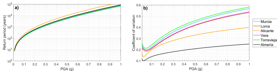
Figure 9. Comparison among the cities studied in this work: (a) mean hazard curves and (b) variability coefficient.
