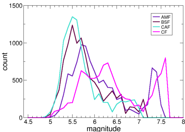
Figure 6. Distribution of maximum magnitudes for 10 000 sub-catalogues divided by faults: the Alhama de Murcia Fault (AMF), the Carboneras Fault (CF), the Carrascoy Fault (CAF) and the Bajo Segura Fault (BSF). The “count” represents the number of times the 10 000 sub-catalogues show the corresponding magnitude as the maximum magnitude on the indicated fault.
