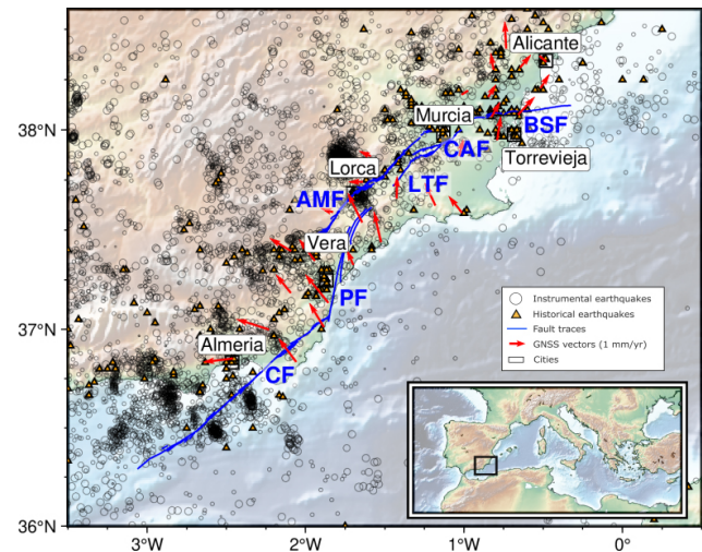
Figure 1. Main faults which constitute the EBSZ (García-Mayordomo et al., 2012b, 2017): the Carboneras Fault (CF), the Palomares Fault (PF), the Alhama de Murcia Fault (AMF), the Los Tollos Fault (LTF), the Carrascoy Fault (CAF) and the Bajo Segura Fault (BSF). The representation of GNSS vectors (Echeverría et al., 2013; Borque et al., 2019) is made with fixed Eurasia. The earthquakes are sourced from the catalogue used in this study (IGN, 2022).
