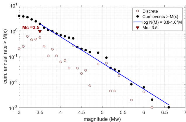
Figure 3. MFD of the EBSZ obtained from the historical and instrumental record since 1048 to 2022. Discrete rate of annual earthquakes, in pink; cumulative annual rate, in black; Gutenberg-Richter relationship (Eq. 1) using maximum likelihood fitting technique (Eq. 8, Utsu, 1964; Aki, 1965), in blue; and the magnitude of completeness ( M_c ), in red.
