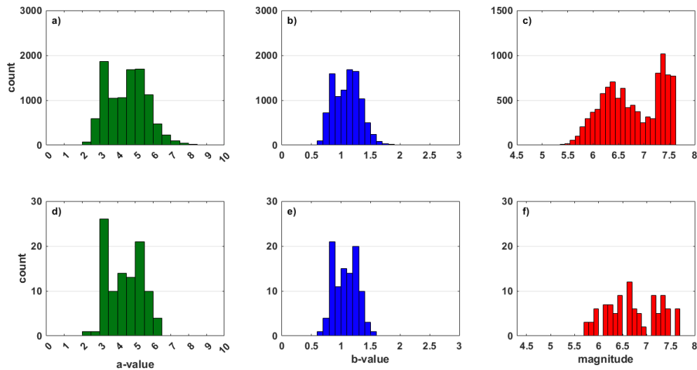
Figure 5. Statistical variability of (a) a – parameter (Gutenberg-Richter relationship), (b) b – parameter (Gutenberg-Richter relationship) and (c) M_{\max} for 10 000 synthetic sub-catalogues and (d), (e) and (f) for 100 synthetic sub-catalogues.
