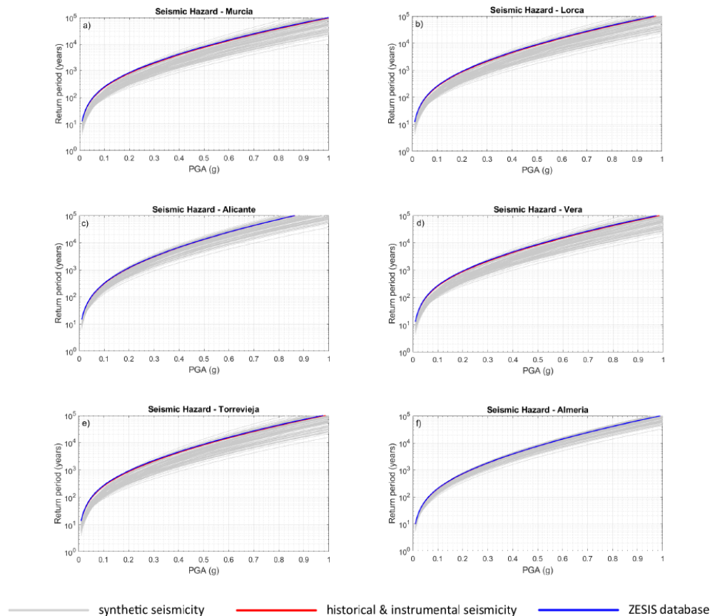
Figure 7. Seismic hazard curves obtained from 100 sub-catalogues of a thousand years build upon a million-year synthetic catalogue (Herrero-Barbero et al., 2021), in grey; upon updated to 2022 catalogue, in red; upon ZESIS database (IGME, 2015), in blue at cities: (a) Murcia, (b) Lorca, (c) Alicante, (d) Vera, (e) Torrevieja y (f) Almería.
