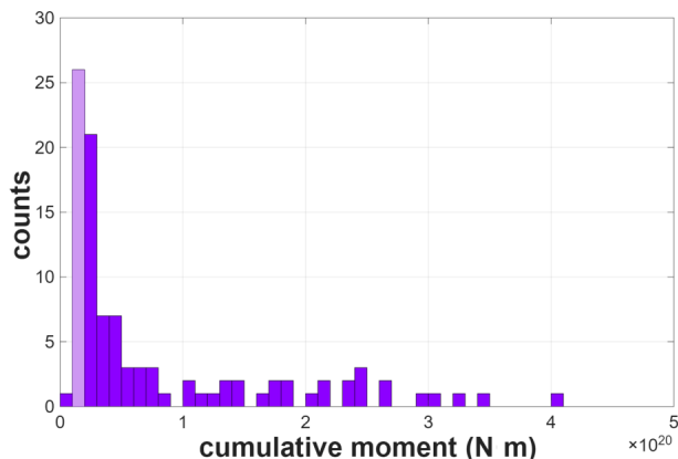
Figure 11. Frequency distribution of cumulative seismic moment for 100 sub-catalogues including the historical and instrumental result (in lilac).
