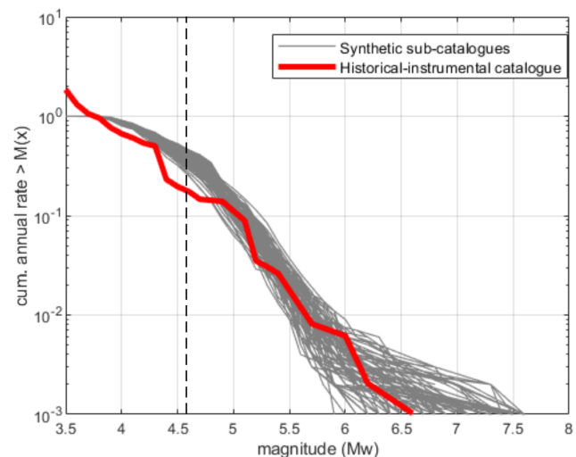
Figure 4. Frequency magnitude distribution for the 100 synthetic catalogues (grey lines) and the historical-instrumental catalogue (red line). The dashed line represents the magnitude of completeness for the full length of synthetic catalogues according to Herrero-Barbero et al. (2021). The magnitude of completeness for the historical-instrumental catalogue is M_w 3.5 (IGN and UPM, 2013).
