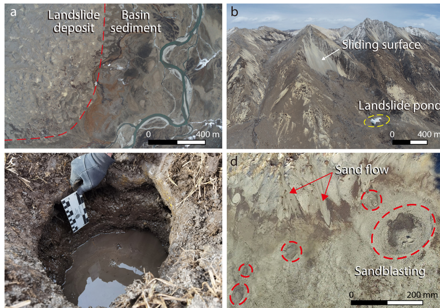
Figure 4. The Luanshibao landslide's geological and hydrogeological features. (a) Aerial photo shows the direct contact boundary of the landslide deposit and alluvial sediment; (b) a frozen landslide pond on the upper part of the landslide, indicating the hydraulic head difference within the landslide mass; (c) shallow groundwater surface exposed after removal of 0.2 m humus soil layer; (d) sandblasting formed craters at the front edge of the landslide.
