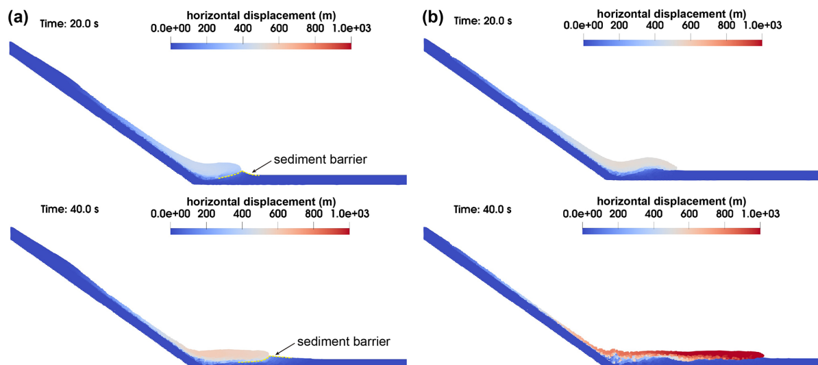
Figure 11. Two possible runout patterns caused by different material properties. (a) A stiffer sliding mass with Young's modulus of 1 \times 10^5 kPa; (b) a more deformable sliding mass with a Poisson's ratio of 0.25.
