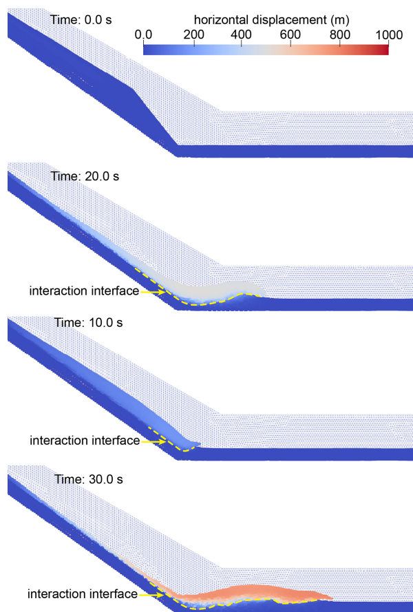
Figure 8. Simulation result of the benchmark scenario shown in the horizontal displacement field.
