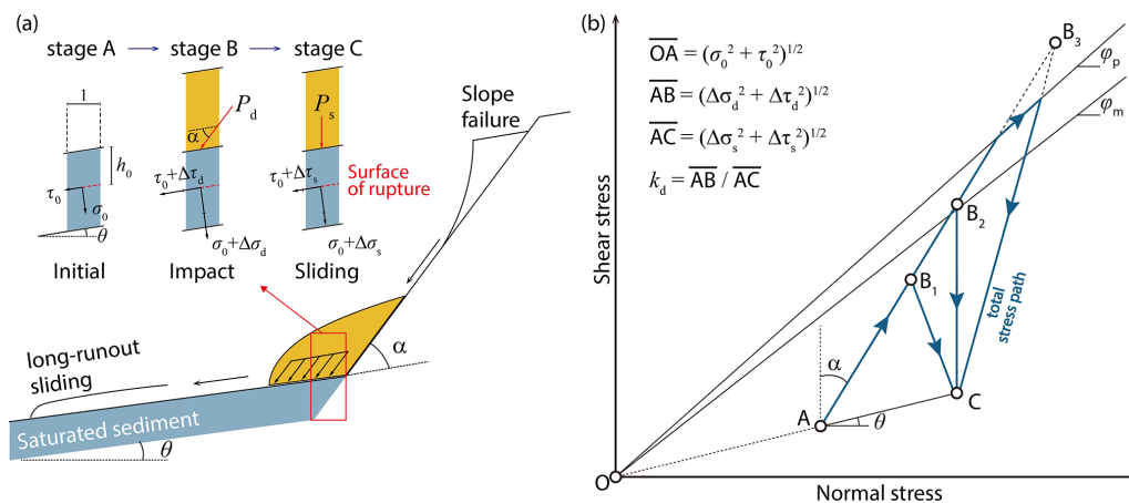
Figure 5. Schematic diagram of the landslide impact effect discussed in this study. (a) Three-stages model of landslide impact-runout process ( h_0 denotes the assumed burial depth of the rupture surface within the sediment layer; \alpha denotes the angle between the initial sliding surface and the sediment surface; \theta denotes the slope angle of the sediment layer); (b) theoretical stress paths of the impact-loading ring-shear tests (modified from Sassa et al., 2004) ( \varphi_p denotes the peak friction angle; \varphi_m denotes the mobilised friction angle). Note that \theta is not necessarily identical in panels (a) and (b) , as the slope of the rupture surface within the sediment layer may differ from the sediment surface slope in real cases.
