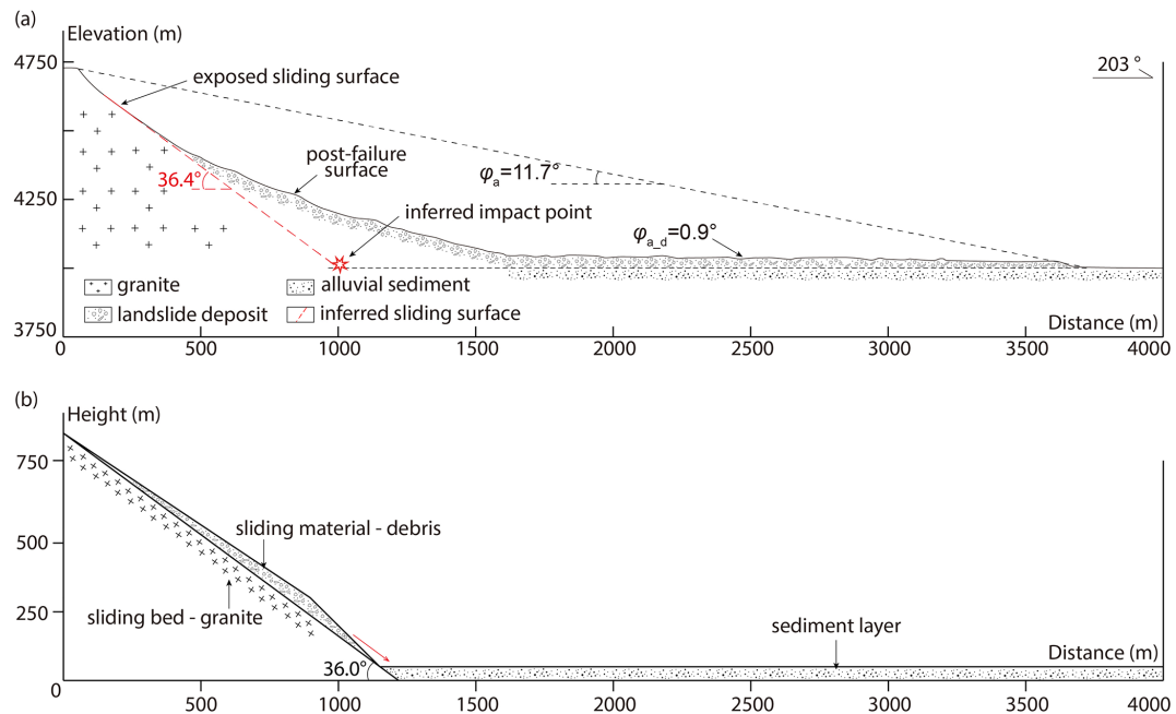
Figure 3. Cross-sectional profiles of the Luanshibao landslide. (a) Longitudinal cross-section of the landslide area showing key kinematic features; (b) geometry of the numerical model cross-section constructed from an adjacent unfailed slope.
