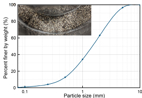
Figure 6. The LSB sand sample and its grain size distribution curve.
