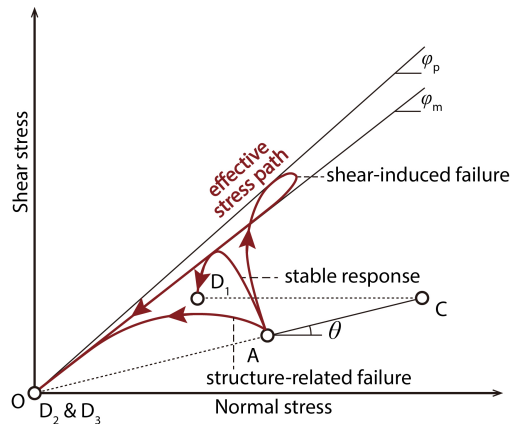
Figure 13. Effective stress paths for three impact responses induced by varying impact coefficient levels.
