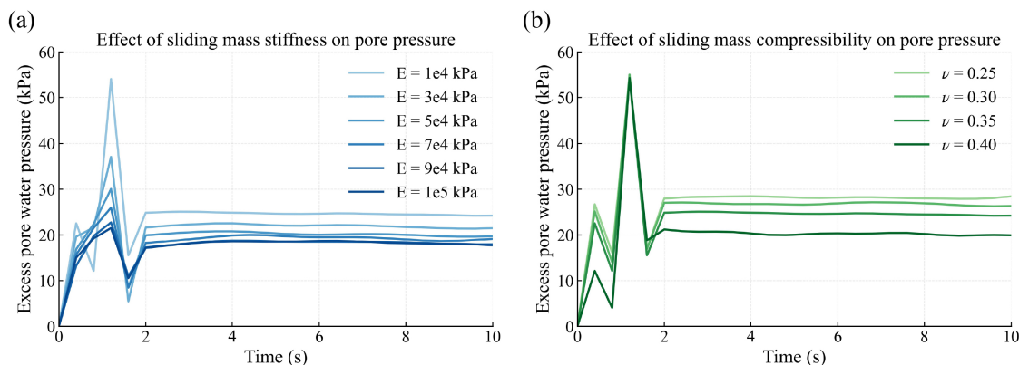
Figure 12. Pore pressure response under varying impact duration determined by elastic parameters. (a) Excess pore pressure response at a representative material point subjected to impacts from sliding masses with different stiffness values; (b) excess pore pressure response at the same point for sliding masses with different compressibility.
