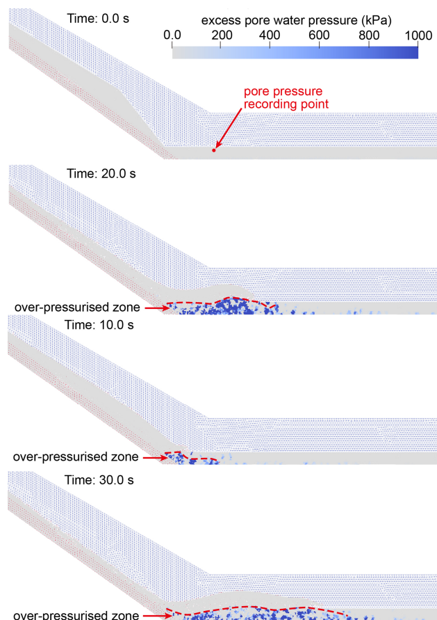
Figure 9. Simulation result of the benchmark scenario shown in the pore water pressure field.
