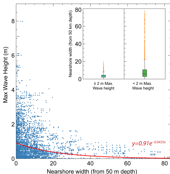
Figure 13. Maximum tsunami wave height from 6879 sampling points across the coastal regions in central and southern Philippines and the corresponding nearshore width (km) relative to 50 m depth. Boxplots show the interquartile range (1.5 IQR) of nearshore width between coastlines with \geq 2 and < 2 m maximum tsunami wave height. Orange circles indicate the outliers of the interquartile range.
