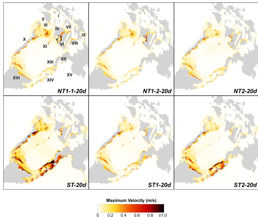
Figure 10. Maximum flow velocity ( \text{m s}^{-1} ) from the 4 h tsunami simulation of six segments with a megathrust dipping at 20^\circ .
