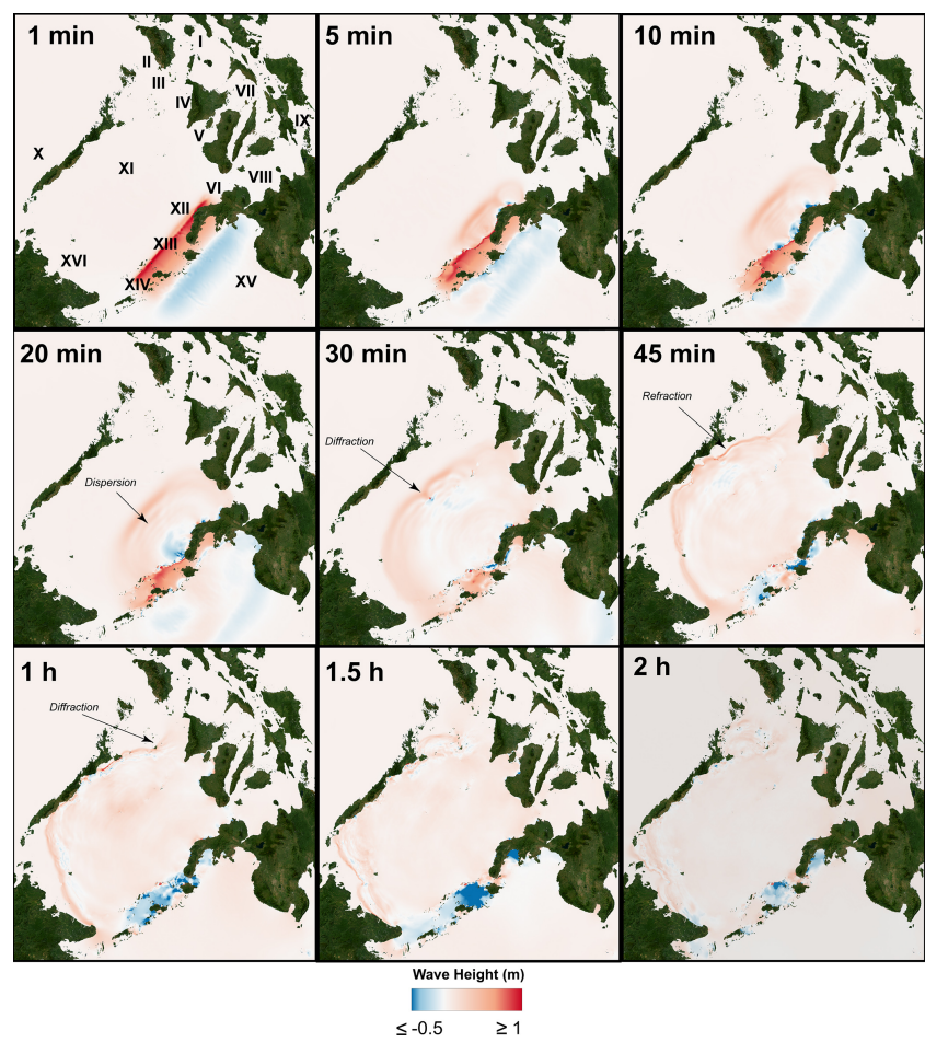
Figure 5. Tsunami wave (2 h) propagation from ST segment at 20° dip angle. Basemap from World Imagery Esri | Powered by Esri.
