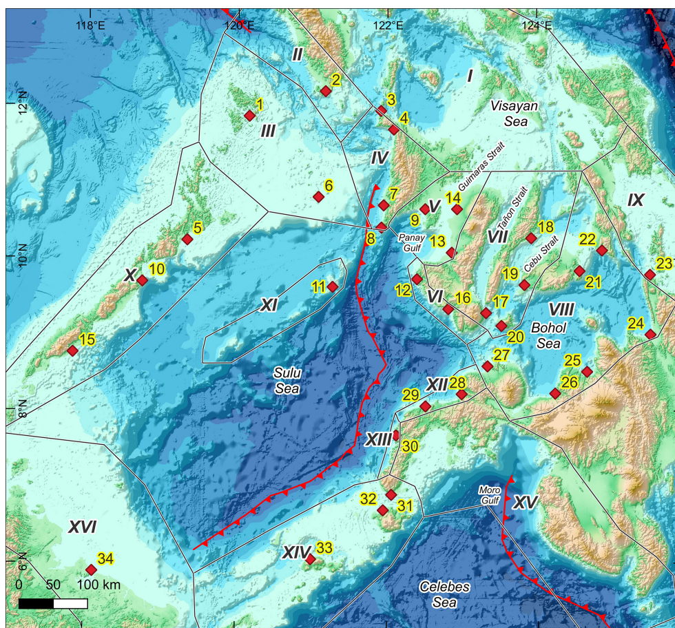
Figure 4. The 16 coastal regions surrounding the Negros–Sulu subduction zone and the 34 synthetic tide gauge stations (TGS). (I) Visayan Sea; (II) Mindoro; (III) Coron–Cuyo; (IV) West Panay; (V) Panay Gulf; (VI) Sipalay–Bayawan; (VII) Tañon–Cebu Strait; (VIII) Bohol Sea; (IX) Leyte Gulf; (X) Palawan; (XI) Cagayancillo; (XII) Sindangan–Labason; (XIII) Siocon–Sibuco; (XIV) Basilan–Sulu; (XV) Moro Gulf; (XVI) northeast Borneo. Basemap from © GEBCO Compilation Group (2024).
