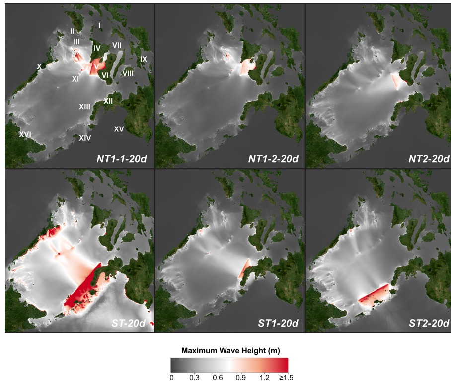
Figure 9. Maximum wave height (m) from the 4 h tsunami simulation of six segments with a megathrust dipping at 20^\circ . Basemap from World Imagery Esri | Powered by Esri.
