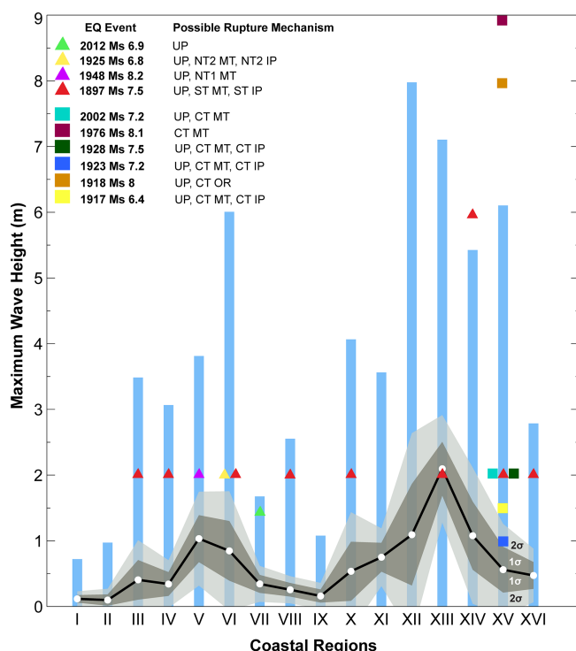
Figure 15. Comparisons of maximum wave heights among the 16 coastal regions from the models and eyewitness accounts (triangles and squares) of historical tsunamigenic earthquakes in the Sulu and Celebes Sea from Bautista et al. (2012). White circles and blue bars indicate the mean and maximum values, respectively, while the envelope indicates the 1\sigma and 2\sigma standard deviations. (I) Visayan Sea; (II) Mindoro; (III) Coron–Cuyo; (IV) West Panay; (V) Panay Gulf; (VI) Sipalay–Bayawan; (VII) Tanon–Cebu Strait; (VIII) Bohol Sea; (IX) Leyte Gulf; (X) Palawan; (XI) Cagayancillo; (XII) Sindangan–Labason; (XIII) Siocon–Sibuco; (XIV) Basilan–Sulu; (XV) Moro Gulf; (XVI) northeast Borneo. Rupture mechanisms: UP, upper plate; MT, megathrust; IP, intraplate; OR, outer rise. Subduction zones: NT, Negros Trench; ST, Sulu Trench; CT, Cotabato Trench.
