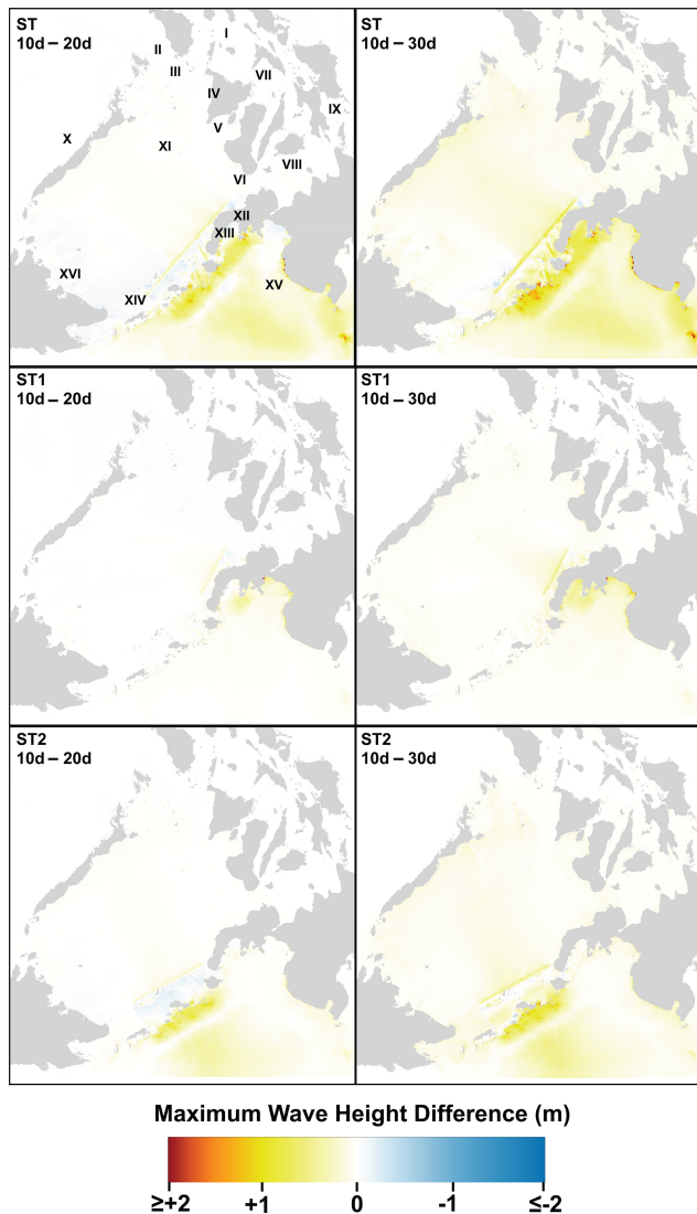
Figure 11. Maximum wave height differences (10–20 and 10–30°) comparing 10°-dip megathrust with those of 20 and 30° in the Sulu Trench (ST) segments.
