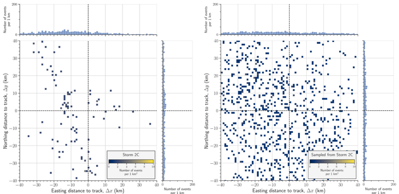
Figure F5. 2D spatial count of lightning strokes per 1 km 2 of easting and northing distances to the movement track in natural time k for thunderstorm 2C (left panel) and for a bivariate Gaussian distribution based on thunderstorm 2C (right panel) for window sizes \Delta w = 500 . Only bins with more than 1 lightning stroke are coloured and the plot is zoomed onto [-40, 40] km intervals for both easting and northing distance. The marginal bin counts per 1 km are given for both dimensions.
