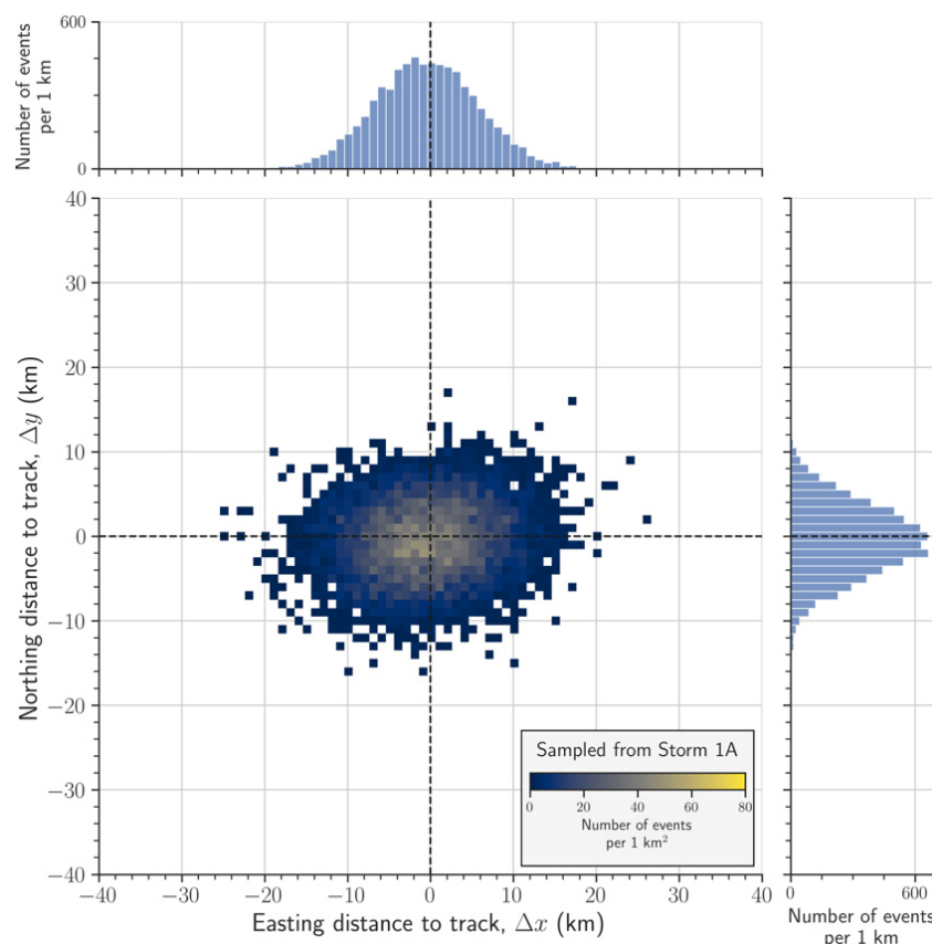
Figure 12. 2D spatial count of lightning strokes per 1 \text{ km}^2 of easting and northing distances to the movement track in natural time k for a bivariate Gaussian distribution based on storm 1A with window size \Delta w = 500 events. Only bins with more than 1 lightning stroke are coloured and the plot is zoomed onto [-40, 40] km intervals for both easting and northing distance. The marginal bin counts per 1 km are given for both dimensions and the parameters of the bivariate Gaussian distribution are (\mu_x = -0.46 \text{ km}, \mu_y = -0.61 \text{ km}, \sigma_{xx} = 37.25 \text{ km}^2, \sigma_{yy} = 17.83 \text{ km}^2, \sigma_{xy} = 2.33 \text{ km}^2) .
