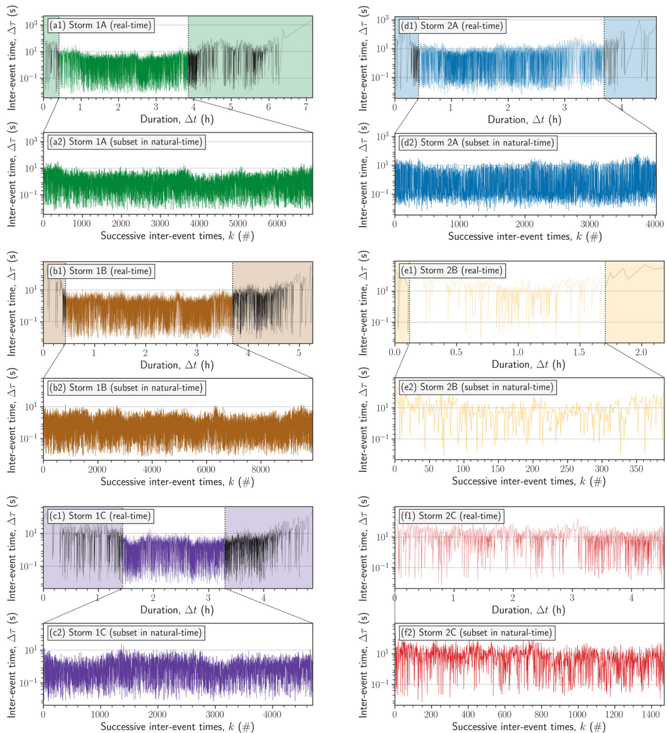
Figure D1. Subplots showing the cutting of inter-event time \Delta\tau time-series in real-time t (removal of black line in upper panel) and the subsequent inter-event time time-series in natural time k (lower panel) for thunderstorms (a1, a2) 1A, (b1, b2) 1B, (c1, c2) 1C, (d1, d2) 2A, (e1, e2) 2B and (f1, f2) 2C.
