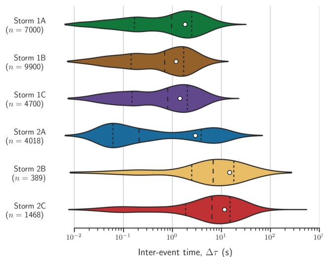
Figure 6. Violin plots of inter-event time \Delta\tau distributions for all six selected thunderstorms. For each thunderstorm, the total number of observations after removing inter-event time values of the time-series is indicated by n , dotted lines denote the quartiles, and the white-dot represents the mean.
