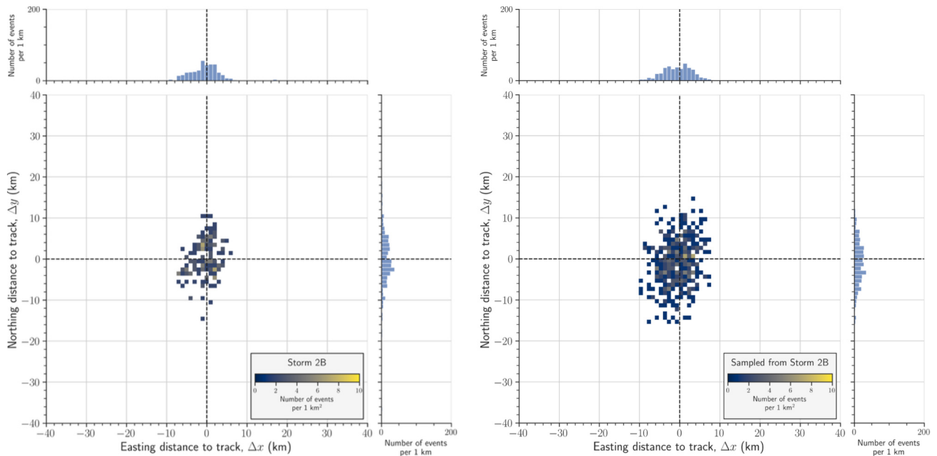
Figure F4. 2D spatial count of lightning strokes per 1 km 2 of easting and northing distances to the movement track in natural time k for thunderstorm 2B (left panel) and for a bivariate Gaussian distribution based on thunderstorm 2B (right panel) for window sizes \Delta w = 500 . Only bins with more than 1 lightning stroke are coloured and the plot is zoomed onto [-40, 40] km intervals for both easting and northing distance. The marginal bin counts per 1 km are given for both dimensions.
