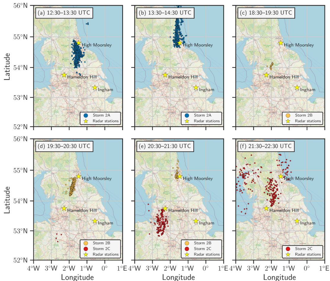
Figure 5. Spatial extent for 1 July 2015 of the lightning stroke occurrences as recorded by the ATDnet system over times intervals corresponding to the relevant synoptic analysis (a) 12:30–13:30 UTC, (b) 13:30–14:30 UTC, (c) 18:30–19:30 UTC, (d) 19:30–20:30 UTC, (e) 20:30–21:30 UTC and (f) 21:30–22:30 UTC. Note that not every 1 h interval is plotted. Only lightning strokes assigned to any of the three selected thunderstorms (Storms 2A, 2B, 2C) are shown. Locations of relevant Doppler radar stations are added as per the legend for direct comparison with synoptic analysis. Background map information from OSM (© OpenStreetMap contributors 2022). Distributed under the Open Data Commons Open Database License (ODbL) v1.0.).
