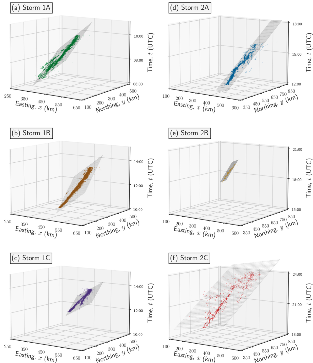
Figure E1. Least-squares plane-fit solution to the lightning stroke datasets for thunderstorms (a) 1A, (b) 1B, (c) 1C, (d) 2A, (e) 2B and (f) 2C. The colour scheme for lightning strokes of each storm is consistent with Figs. 4 and 5 and the best-fit plane is drawn as grey wireframe. Note that all three axes have different extents for each storm, while the ratio between the axes is constant.
