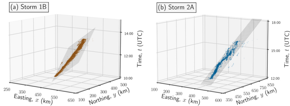
Figure 7. Least-squares plane-fit solution to the lightning stroke datasets for (a) Storm 1B (28 June 2012, n = 9901 events, v = 13 \text{ m s}^{-1} ( 47 \text{ km h}^{-1} )), and (b) Storm 2A (1 July 2015, n = 4019 events, v = 30 \text{ m s}^{-1} ( 108 \text{ km h}^{-1} )). Note that all three axes have different extents for each storm, while the ratio between the axes is constant. The best-fit plane solution is overlaid as a wireframe over the individual lightning strokes.
