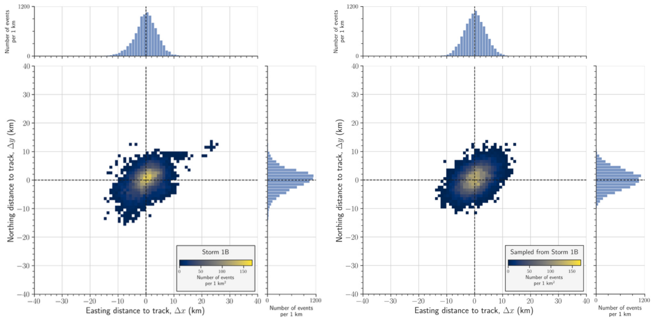
Figure F1. 2D spatial count of lightning strokes per 1 km 2 of easting and northing distances to the movement track in natural time k for thunderstorm 1B (left panel) and for a bivariate Gaussian distribution based on thunderstorm 1B (right panel) for window sizes \Delta w = 500 . Only bins with more than 1 lightning stroke are coloured and the plot is zoomed onto [-40, 40] km intervals for both easting and northing distance. The marginal bin counts per 1 km are given for both dimensions.
