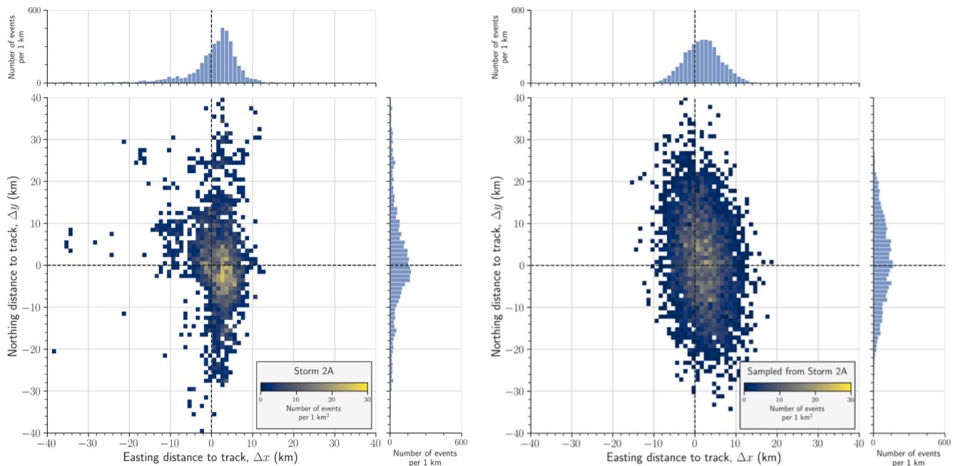
Figure F3. 2D spatial count of lightning strokes per 1 km 2 of easting and northing distances to the movement track in natural time k for thunderstorm 2A (left panel) and for a bivariate Gaussian distribution based on thunderstorm 2A (right panel) for window sizes \Delta w = 500 . Only bins with more than 1 lightning stroke are coloured and the plot is zoomed onto [-40, 40] km intervals for both easting and northing distance. The marginal bin counts per 1 km are given for both dimensions.
