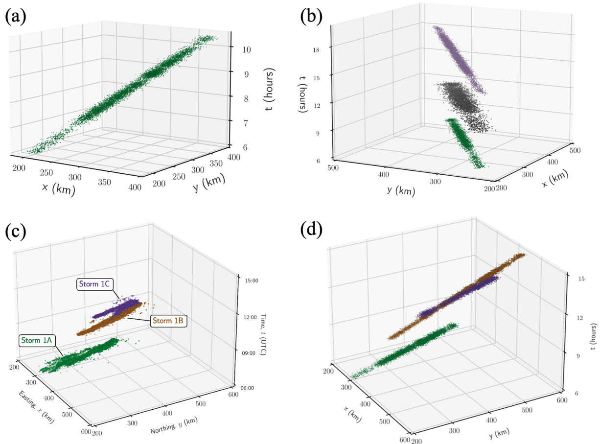
Figure 13. (a) A single run of the spatio-temporal model to produce a lightning stroke dataset representative of storm 1A and a (b) synthetic three-storm system with varying spatial spread parameters. In panel (a), the initiation point is set at (x_0 = 200 \text{ km}, y_0 = 200 \text{ km}, t_0 = 6 \text{ h}) . The movement speed value is set at v = 16 \text{ m s}^{-1} as per the characterisation of the movement speed variable (Appendix Fig. E1). Inter-event times are sampled, sorted and re-indexed as per Fig. 11a1–a4. Easting and northing distances are sampled from the bivariate Gaussian distribution shown in Fig. 12. The first (green) storm is identical to panel (a) with bivariate Gaussian distribution parameter set from parameter characterisation ( \mu_x = -0.46 \text{ km} , \mu_y = -0.61 \text{ km} , \sigma_{xx} = 37.25 \text{ km}^2 , \sigma_{yy} = 17.83 \text{ km}^2 , \sigma_{xy} = 2.33 \text{ km}^2 ). The second (dark grey) storm is based on bivariate Gaussian distribution with parameters ( \mu_x = 0 , \mu_y = 0 , \sigma_{xx} = 100 \text{ km}^2 , \sigma_{yy} = 100 \text{ km}^2 , \rho = 0 ). The third (purple) storm has parameters ( \mu_x = 0 , \mu_y = 0 , \sigma_{xx} = 100 \text{ km}^2 , \sigma_{yy} = 100 \text{ km}^2 , \rho = 0.9 ). For all storms, the movement speed is kept the same at v = 16 \text{ m s}^{-1} and inter-event time distribution is representative of storm 1A. A synthetic three-storm system representative of Storms 1A, 1B and 1C from case study 1 (c). The movement speed values, re-indexed inter-event time values and spatial spread parameter distributions are selected for each storm using Table 3.
