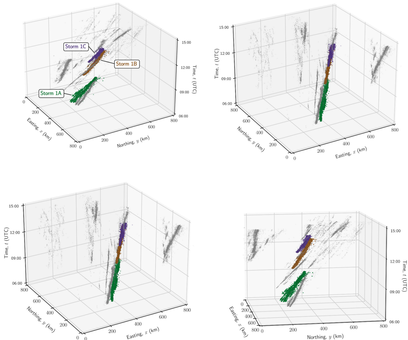
Figure B1. Angles of the 3D spatial extent and propagation of the lightning stroke occurrences plots in Fig. 4. Lightning strokes are projected onto the OSGB 1936/British National Grid northing/easting coordinates, assigned to the identified thunderstorms corresponding to the relevant synoptic analysis.
