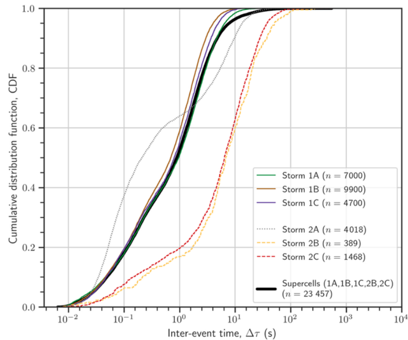
Figure 10. Cumulative distribution function (CDF) for the inter-event time \Delta\tau for all six identified thunderstorms and the combined supercell thunderstorm dataset (black solid line). Individual storms within the storm system recorded on 28 June 2012 (Storms 1A, 1B and 1C) are indicated by solid lines, while those from storm system recorded on 1 July 2015 (Storms 2A, 2B and 2C) are indicated by dashed lines. Storm 2A is indicated by a grey line due to being single-cell thunderstorm and is not added to the supercell dataset.
