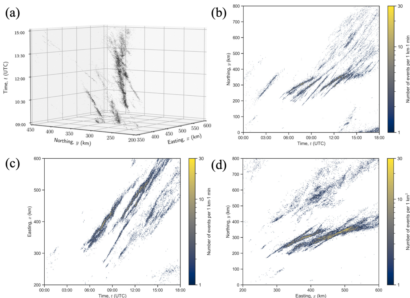
Figure 2. The lightning stroke data subset available for assignment to Storm 1B of the first case study in (a) three-dimensional, (b) two-dimensional northing-time, (c) two-dimensional easting-time and (d) two-dimensional northing easting views. The case study is based on a synoptic analysis of three supercell thunderstorms that crossed the English Midlands on 28 June 2012. For assignment and three-dimensional view, the spatial extent was restricted to x = (350, 600) km and y = (200, 450) km in the OSGB 1936 (EPSG:27700) easting/northing coordinates and the temporal extent from 09:00–15:00 UTC. All available lightning strokes are indicated as black scatter points in three-dimensional view and bin counts according to the colourscale in the two-dimensional views.
