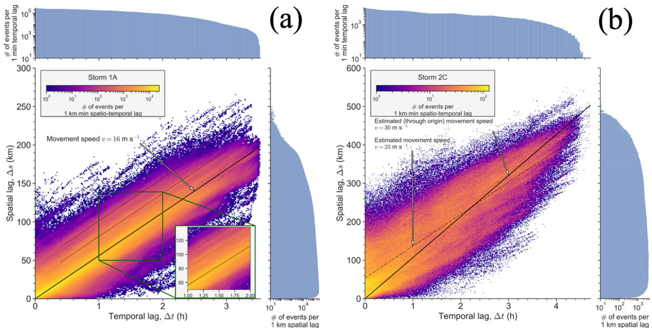
Figure 8. (a) Storm 1A (28 June 2012, n = 7001 events, v = 16 \text{ m s}^{-1} ( 59 \text{ km h}^{-1} )) and (b) storm 2C (1 July 2015, n = 1469 events, v = 30 \text{ m s}^{-1} ( 108 \text{ km h}^{-1} )) least-squares linear-fit solution and 2D count of lightning strokes per 1 km min in the spatio-temporal lag space. Bins are coloured according to the given logarithmic colour scale. The marginal bin counts per 1 km spatial lag and 1 min temporal lag are given above and to the right of the main plot. The abrupt vertical end of lightning stroke data in panel (a) at \Delta t = 3.45 \text{ h} occurs due to the removal of inter-event time values. The solid black line indicates the best-fit linear line passing through the point of origin, while the dash-dotted line in panel (b) indicates the best-fit linear line. The two dashed lines in panel (a) parallel to the dark line, both set with identical v = 16 \text{ m s}^{-1} ( 59 \text{ km h}^{-1} ) indicate other areas of increased count density (bandings of orange pixels as seen in the enlarged panel in the lower right corner). These lines are set manually to emphasise the visually observable structure in the data.
