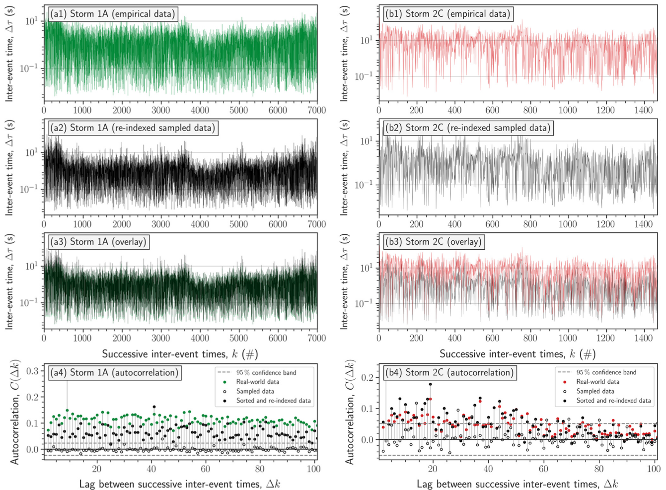
Figure 11. Sampling, sorting and re-indexing procedure based on the combined supercell inter-event time \Delta\tau dataset and thunderstorm (a) 1A, (b) 2C. The first panel (a1, b1) shows the original cut inter-event time-series in natural time k . The second panel (a2, b2) shows this sampled time-series being sorted and re-indexed based on the individual thunderstorm, where the indices of sorted time-series coincide between the two time-series. The third panel (a3, b3) shows the overlay between the original time-series and the sorted and re-indexed one in natural time k . The fourth panel (a4, b4) shows the autocorrelation comparison, including the confidence band.
