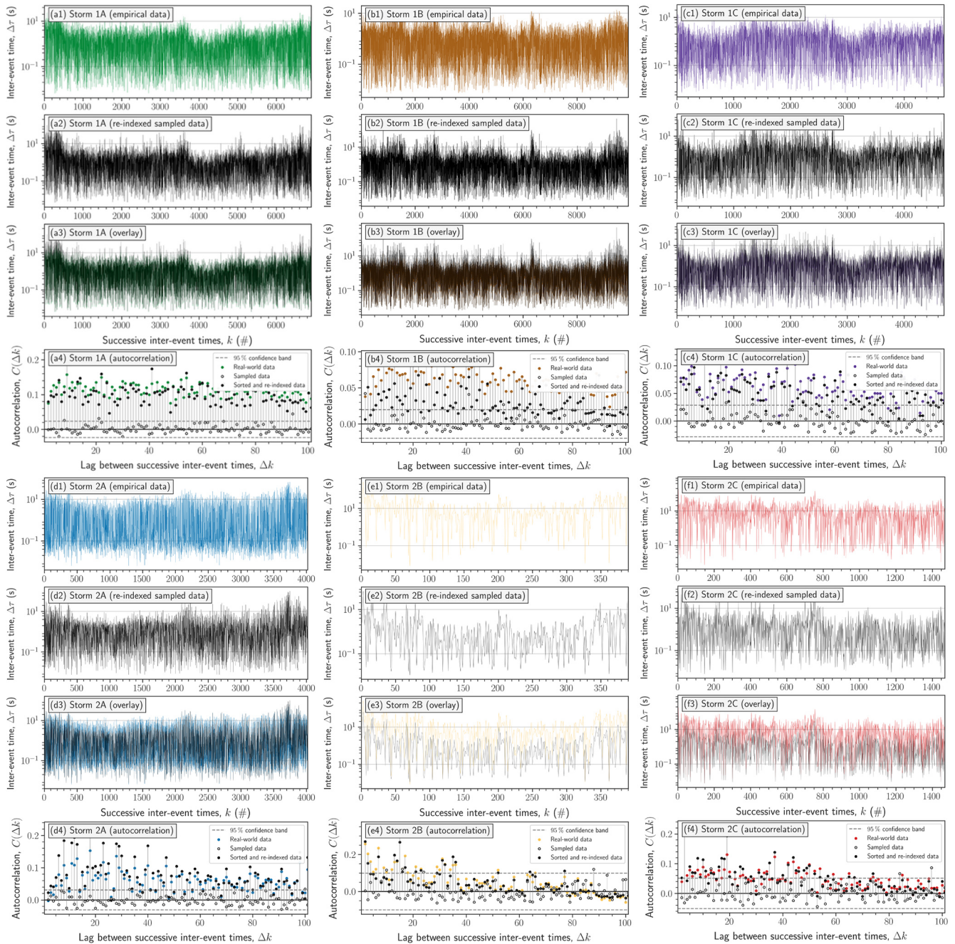
Figure G1. Sampling, sorting and re-indexing procedure based on the combined supercell inter-event time \Delta\tau dataset and thunderstorm (a) 1A, (b) 1B, (c) 1C, (d) 2A, (e) 2B and (f) 2C. The first panel (a1, b1, c1, d1, e1, f1) shows the original cut inter-event time series in natural time k . The second panel (a2, b2, c2, d2, e2, f2) shows this sampled time series being sorted and re-indexed based on the particular thunderstorm, where the indices of the sorted time series coincide between the two time series. The third panel (a3, b3, c3, d3, e3, f3) shows the overlay between the original time-series and the sorted and re-indexed one in natural time k . The fourth panel (a4, b4, c4, d4, e4, f4) show the autocorrelation comparison, including the 95 % confidence band.
