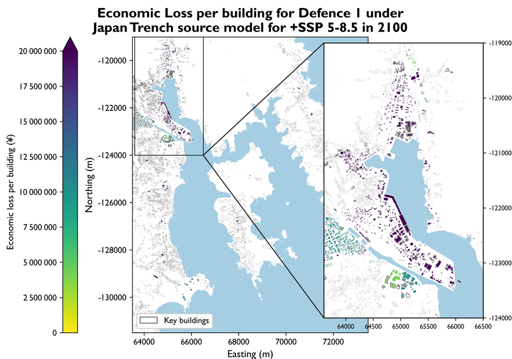
Figure 14. Spatial distribution of economic loss per building for Defence 1 under the Japan Trench source, SSP5–8.5 scenario in 2100. Loss hotspots are concentrated around Kesennuma's port, waterways, and coastal margins, where inundation depth and building density are highest. Inland and elevated zones exhibit minimal losses due to reduced exposure and topographic protection.
