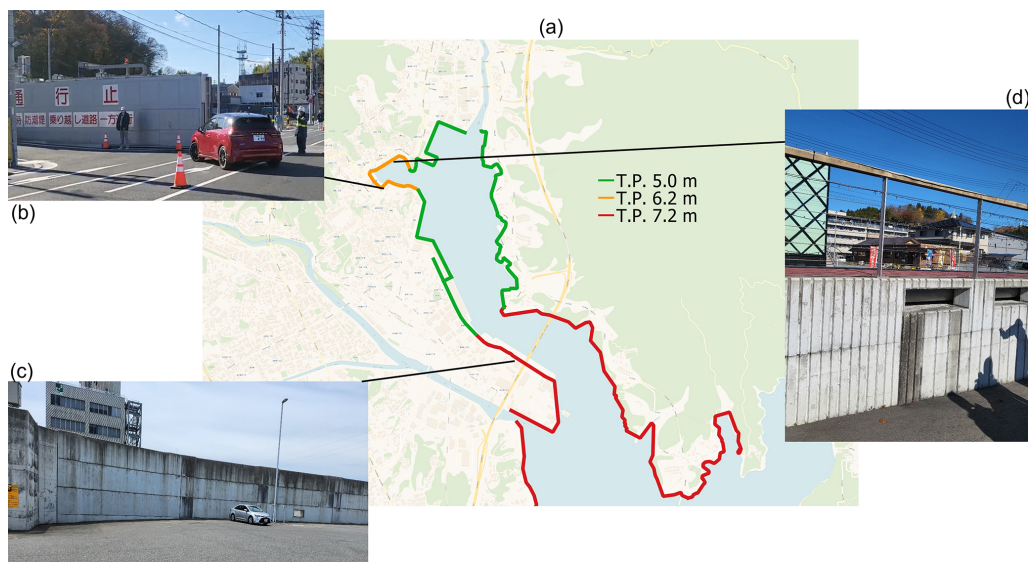
Figure 2. Current tsunami mitigation infrastructure in Central Kesennuma (a) Seawall heights, (b) automatic seagate controlled remotely by J Alert in Tokyo, (c) tallest concrete seawall observed at Kesennuma Port, (d) barrier hydraulically activated by water ingress, increasing barrier height by 1 m. Base map from OpenStreetMap contributors.
