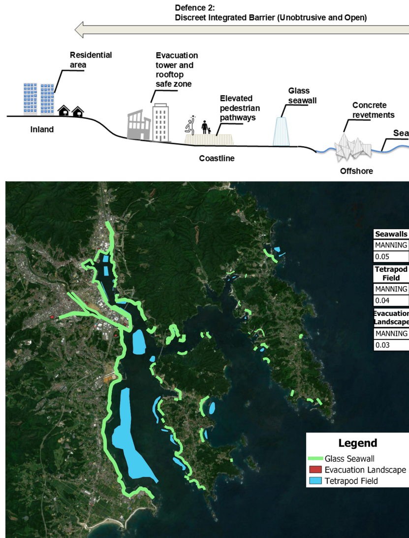
Figure 4. Multi-layered defence cross-section and in-situ placement for the Discreet Integrated Barrier system (Defence 2). Sentinel-2 imagery by © European Union, Copernicus Programme. All rights reserved.
