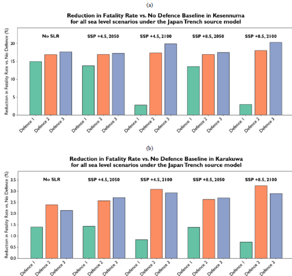
Figure 12. Fatality reduction relative to the no-defence baseline for the three defence configurations under all SLR scenarios for (a) Kesennuma and (b) Karakuwa, based on the Japan Trench tsunami source model. In Kesennuma, Defence 2 and Defence 3 show increasing reduction as SLR increases, while Defence 1's reduction falls sharply under late-century, high-emission scenarios. The same pattern is observed in Karakuwa.
