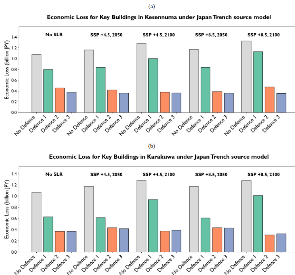
Figure 15. Economic loss for key buildings in (a) Kesennuma and (b) Karakuwa, mirroring results from all buildings where Defence 1 produces consistently higher losses across all scenarios and Defences 2 and 3 differ only marginally.
