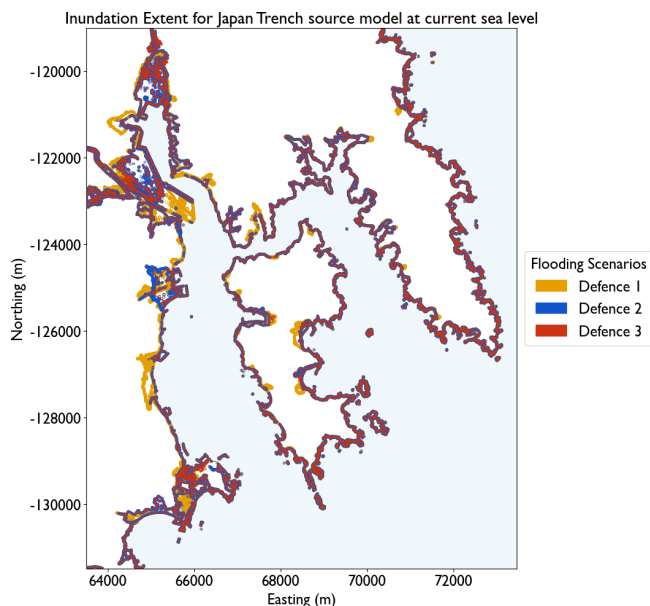
Figure 11. Spatial extents showing differences in inundation patterns and areas for each defence configuration.
