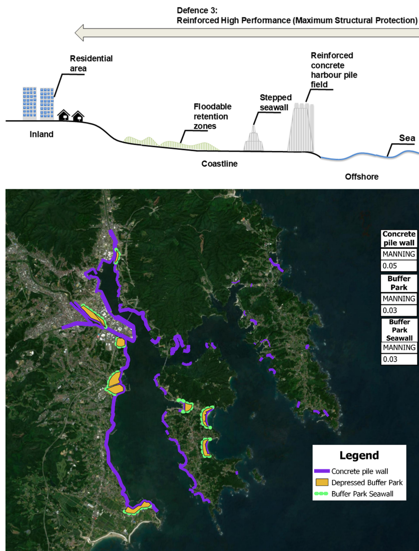
Figure 5. Cross-section and in-situ placement of the three elements from the Reinforced High-Performance system (Defence 3). Sentinel-2 imagery by © European Union, Copernicus Programme. All rights reserved.
