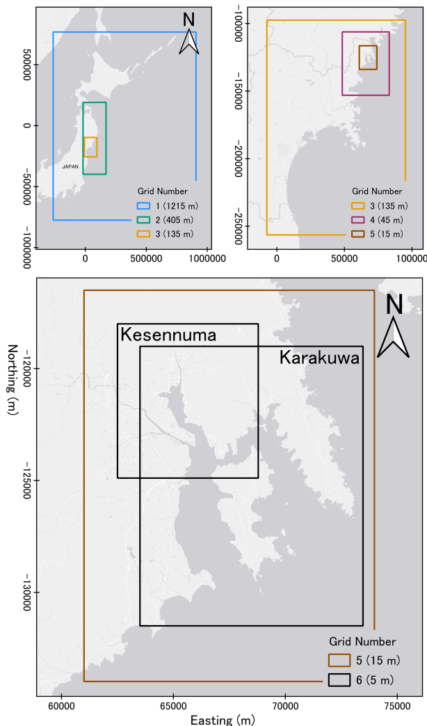
Figure 6. Computational Domain (Grid 1) and the subsequent nesting grids, showing the difference in locations of the Kesennuma and Karakuwa final grids. Sources: Esri (World Gray Canvas) | Powered by Esri.
