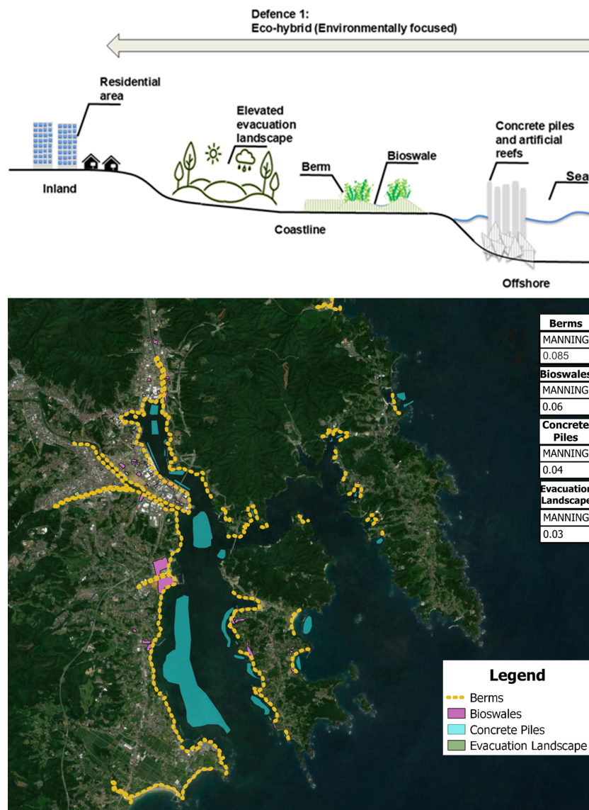
Figure 3. Multi-layered defence cross section and placement within Kesennuma for the Eco-hybrid defence system (Defence 1). Sentinel-2 imagery by © European Union, Copernicus Programme. All rights reserved.
