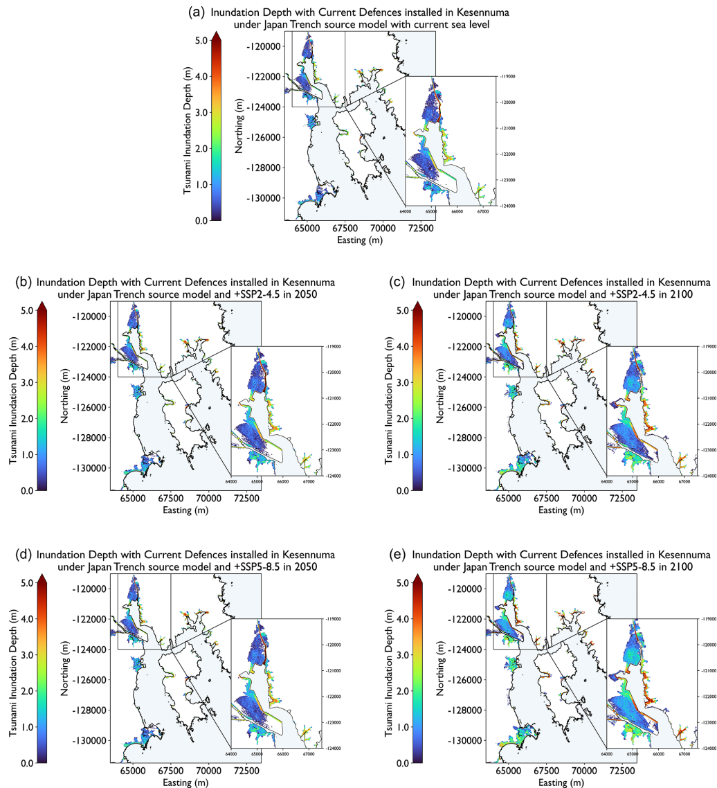
Figure 9. Increasing inundation extent and depth under different SLR scenarios (a) No SLR, (b) SSP2–4.5 in 2050, (c) SSP2–4.5 in 2100, (d) SSP5–8.5 in 2050 and (e) SSP5–8.5 in 2100 for the defences currently installed within Kesennuma. Results are shown for the Japan Trench scenario as the representative case, as all three modelled sources produced consistent relative patterns.
