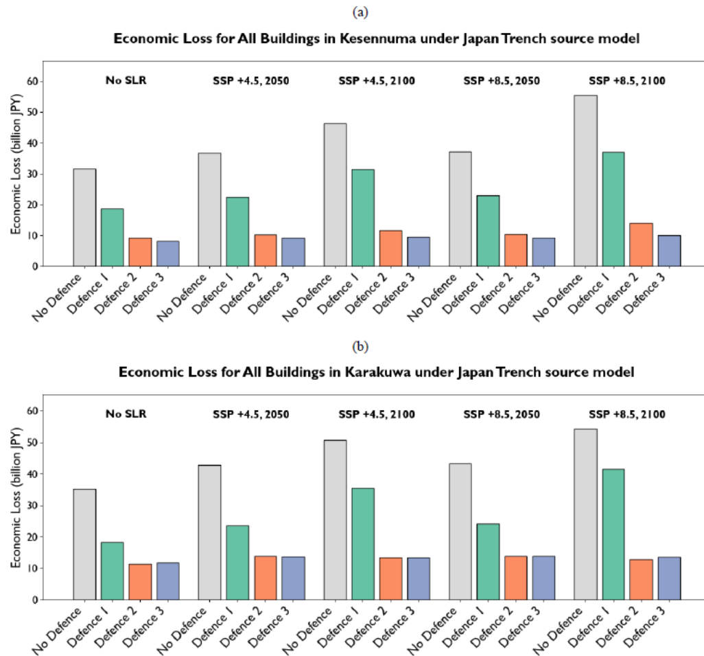
Figure 13. Economic loss for all buildings in (a) Kesennuma and (b) Karakuwa. Defence 1 produces consistently higher losses across all scenarios, while Defences 2 and 3 differ only marginally.
