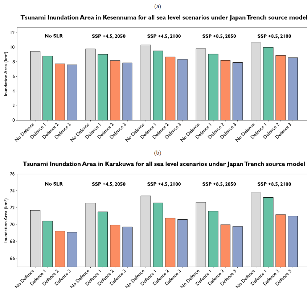
Figure 10. Inundation area for (a) Kesennuma and (b) Karakuwa across all SLR scenarios for the three defence configurations and a No Defence baseline, based on the Japan Trench tsunami source model, shown as the representative case because all three modelled sources produced the same relative performance hierarchy among the defence configurations. In both locations, inundation extent increases with SLR, with Defence 2 and Defence 3 limiting area more effectively than Defence 1.
