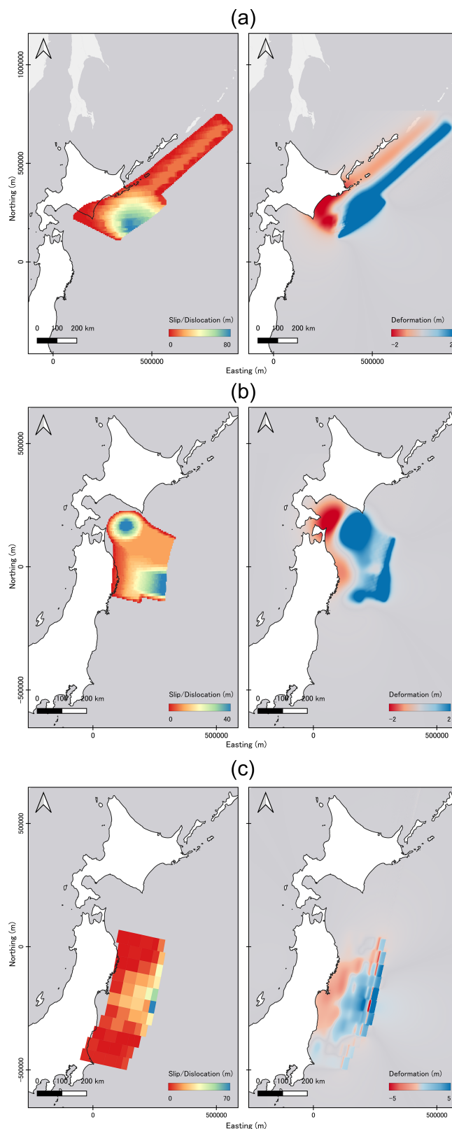
Figure 7. Tsunami source model locations, slip distribution and deformation for (a) Kuril Trench (b) Japan Trench and (c) 2011 GEJE (Tohoku).
