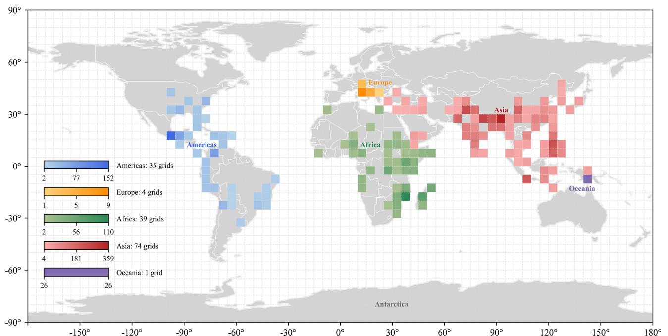
Figure 5. Global distribution of ARI in 5^\circ \times 5^\circ latitude–longitude grids across continental regions.
