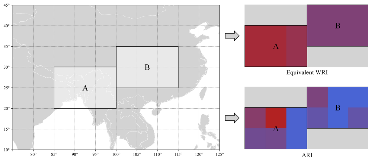
Figure 4. Local zoom-in comparison of ARI and Equivalent WRI in 5^\circ \times 5^\circ latitude–longitude grids.
