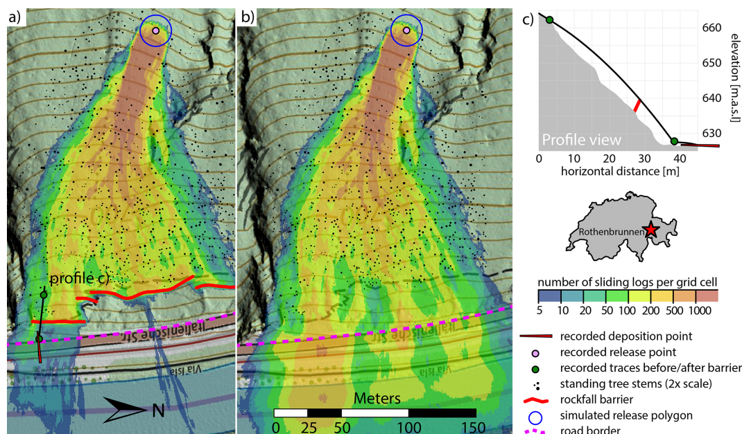
Figure 4. Reconstruction of the 2022 event in Plattawald, Rothenbrunnen (CH). All simulations were done with 20 000 randomly distributed upright logs within the release polygon and a friction coefficient of \mu = 0.25 . The colours indicate how many of the 20 000 released logs intersect their motion with each 0.5 \times 0.5 m grid cell, revealing preferential sliding paths of the deadwood. (a) Simulation with ALS-based tree locations and rockfall barriers. (b) Simulation with ALS-based tree locations without barriers. (c) Profile view in the vicinity of the presumably overjumped rockfall barrier with fitted flight parabola. Map and hillshade from swisstopo (2020–2024).
