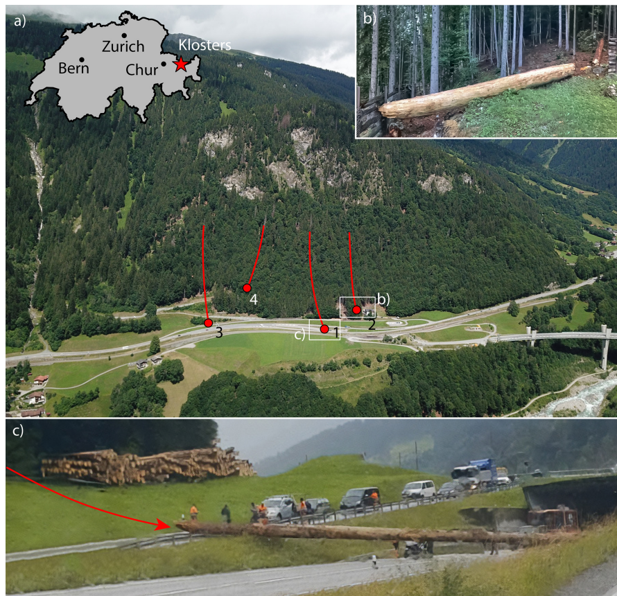
Figure 1. The four 2022 events in Gruobewald, Klosters (CH). (a) Overview of Gruobewald, including endangered residential area, road and railway. The trajectories and deposition points of the four events are shown qualitatively. Photograph by AWN GR. (b) Deposition of event 2 in a wooden palisade next to a house. (c) Deposition of event 1 on the road. Photograph credit for panels (b) and (c) : Flurin Wehrli.
