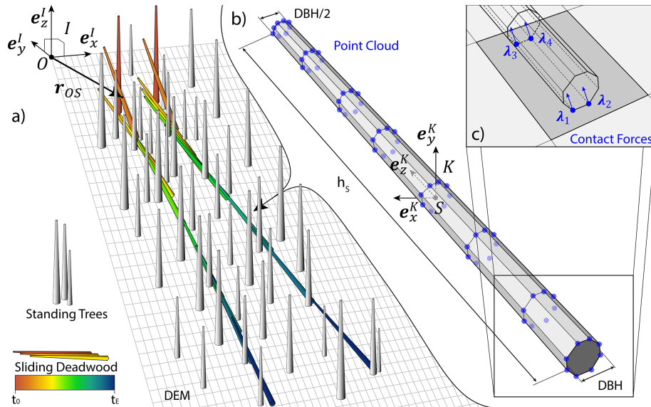
Figure 2. Simulation model of the sliding deadwood. (a) DEM and standing trees are described in the inertial frame I . Two sliding deadwood logs are exemplary shown as a time series starting at the mobilisation time t_0 up to the deposition time t_E . (b) Rigid, sliding deadwood with its geometry described as a point cloud in body-fixed frame K fixed at the centre of mass S . (c) Contact between deadwood geometry and terrain with contact forces \lambda_i acting at vertex points of the point cloud.
