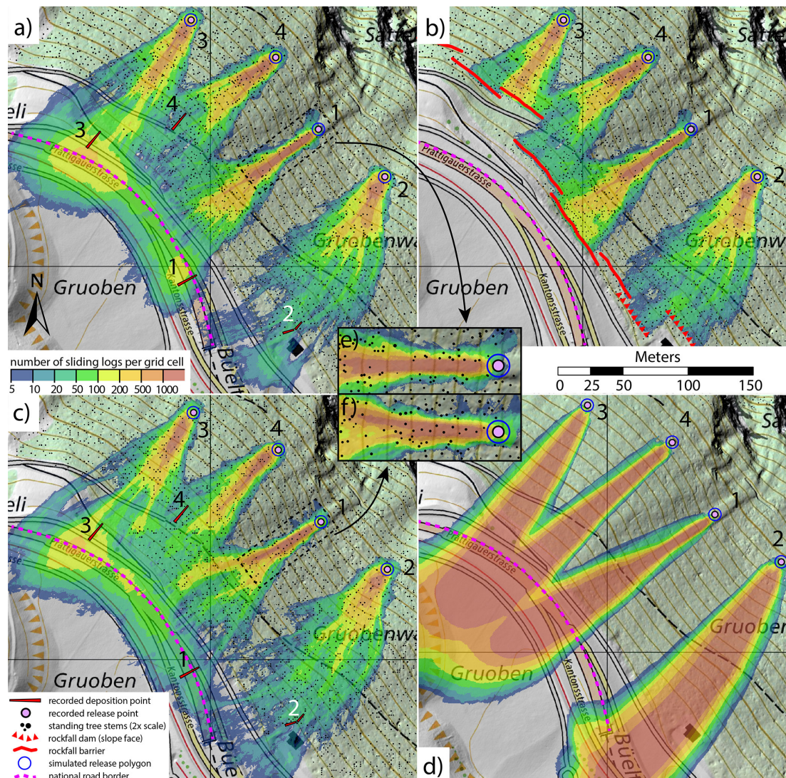
Figure 3. Reconstruction of the four events in Gruobenwald, Klosters (CH) with a friction coefficient of \mu = 0.25 . The colours indicate how many of the 20 000 released logs intersect their motion with each 0.5 \times 0.5 m grid cell, revealing preferential sliding paths of the deadwood. (a) Simulation without protection measures and ALS-based tree locations. (b) Simulation with protection measures finished in 2024 and ALS-based tree locations. (c) Simulation without protection measures and randomly generated forest. (d) Simulation without protection measures and no forest. Two magnified sections below release 1 reveal the differences of the forest structure between ALS-based forest (e) and randomly generated forest (f). Map and hillshade from swisstopo (2020–2024).
