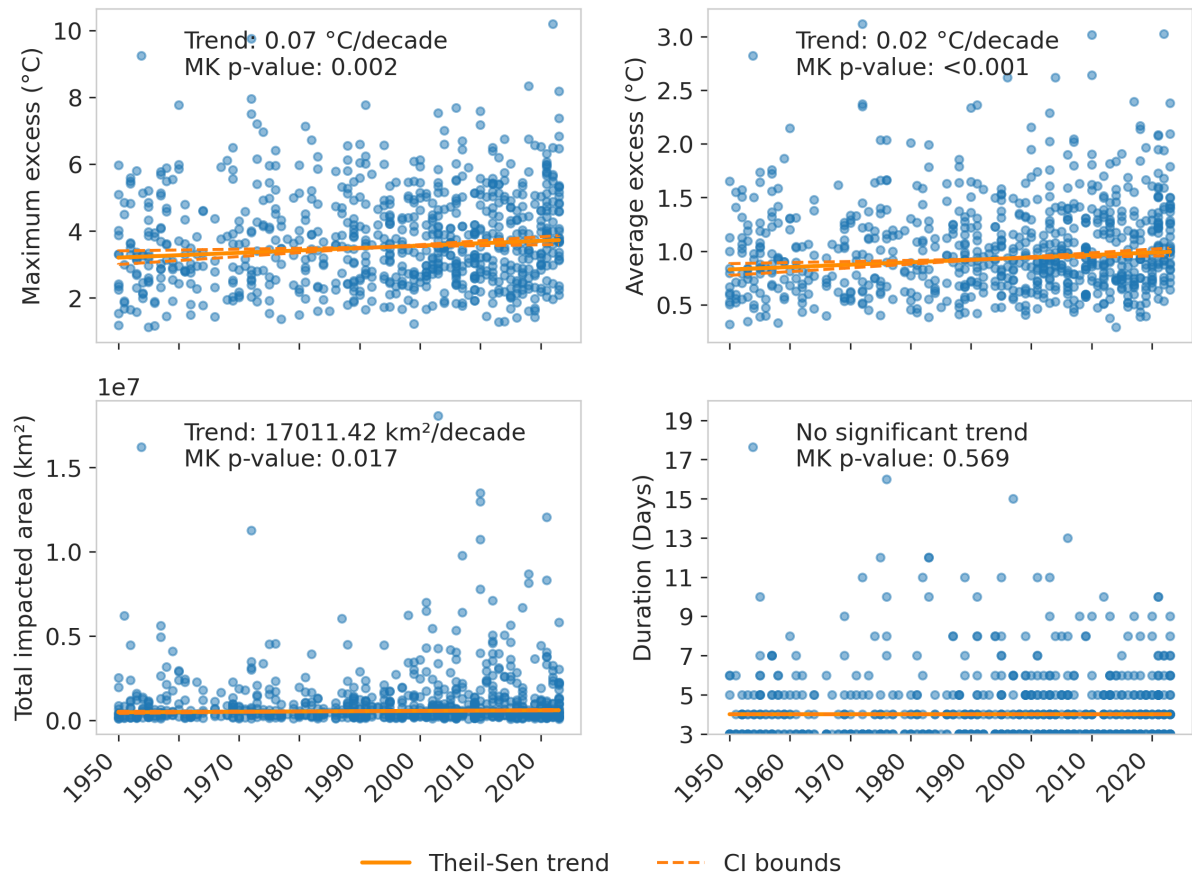
Figure S3. Trends in maximum excess, mean excess, total impacted area, and duration for heatwaves detected over Europe from 1950 to 2024.
