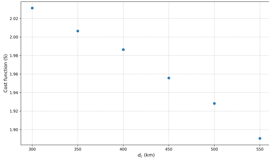
Figure S2. Cost function S as a function of d_c for heavy precipitation events, with A_{\min} = 25\,000 km 2 and d = 200 km.
