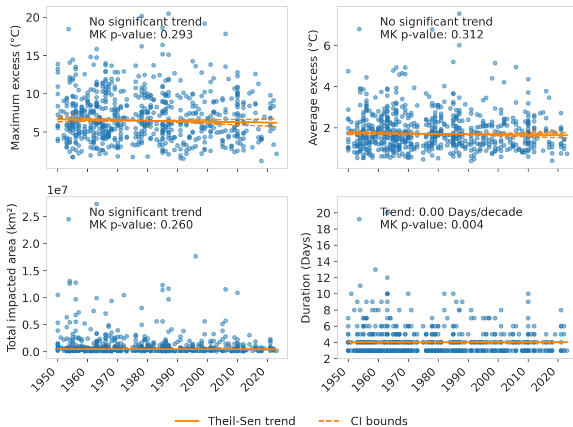
Figure S4. Trends in maximum excess, mean excess, total impacted area, and duration for cold spells detected over Europe from 1950 to 2024.
