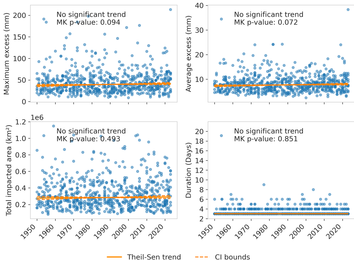
Figure S5. Trends in maximum excess, mean excess, total impacted area, and duration for heavy precipitation events detected over Europe from 1950 to 2024.
