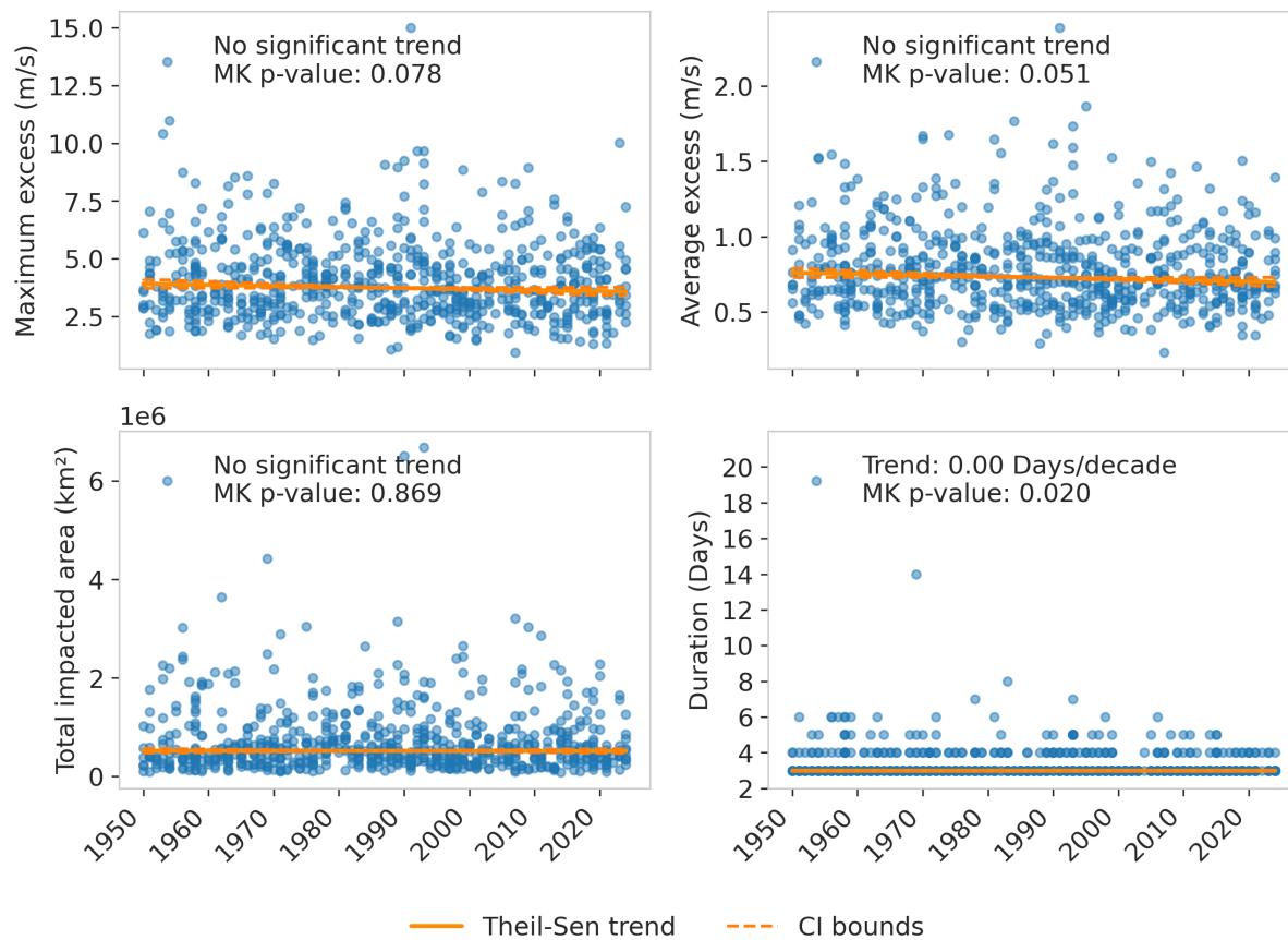
Figure S6. Trends in selected metrics for extreme wind events detected over Europe.
