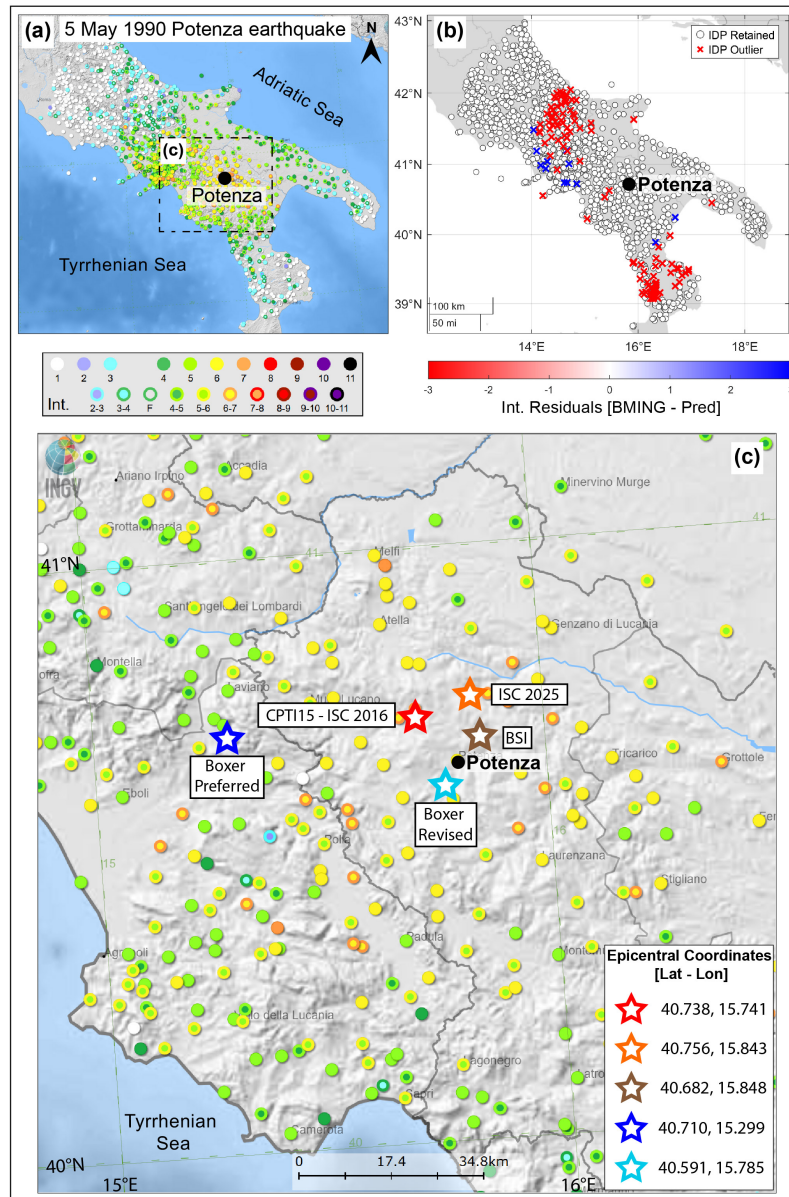
Figure 2. The 5 May 1990 ( M_w 5.8) Potenza earthquake. (a) Macroscopic intensity distribution of the BMING dataset (Bollettino Macro-sismico ING) from Gasparini et al. (1991b). (b) Intensity residuals (blue = positive; red = negative) between BMING observations and predictions from the IPE of Gomez-Capera et al. (2024), where crosses indicate the 116 identified outliers. (c) Comparison of epicentral locations: red, orange, and brown stars represent the instrumental epicentral solutions from CPTI15-ISC 2016 (International Seismological Centre, 2016), ISC 2025 (International Seismological Centre, 2025), and BSI, respectively. Blue and light blue stars indicate the macroseismic epicentres derived with Boxer from the preferred (BMING) and revised macroseismic fields. Maps in panels (a) and (c) are derived from the CPTI15-DBMI15 catalogue, which uses the TINITALY Digital Elevation Model as background. CPTI15-DBMI15 data courtesy of INGV. © INGV. All rights reserved.
