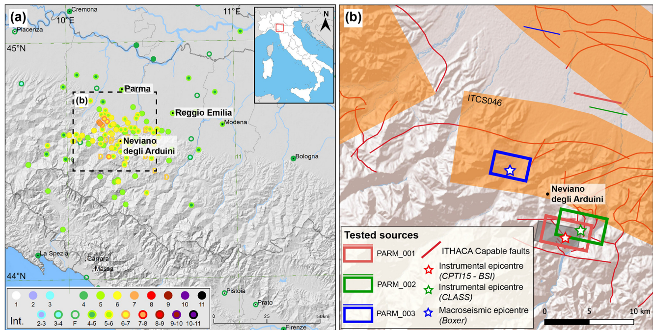
Figure 7. The 23 December 2008 ( M_w 5.36) Parmense earthquake. (a) Macroseismic intensity distribution of the ERCAL009 dataset from Ercolani et al. (2009). (b) Tested source configurations (coloured rectangles). Red lines represent capable faults from ITHACA. The orange shaded area represents the Composite Seismogenic Source (CSS) “ITCS046”, while the grey rectangle represents the “ITIS135 Neviano degli Arduini” proposed by the DISS database (DISS Working Group, 2025). Red, green, and blue stars represent the instrumental epicentral solutions from CPTI15 (BSI), CLASS, and the macroseismic epicentre, respectively. The map in panel (a) is derived from the CPTI15-DBMI15, which uses the TINITALY DEM, whereas panel (b) is generated using the Esri Shaded Relief basemap. Sources: Esri | Powered by Esri.
