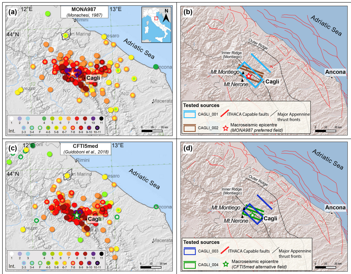
Figure 8. The 3 June 1781 Cagli earthquake. (a) Macroseismic intensity distribution of the MONA987 dataset from Monachesi (1987). (b) Tested source configurations (CAGLI_001 and CAGLI_002). (c) Macroseismic intensity distribution of the CFTI5med dataset from Guidoboni et al. (2018). (d) Tested source configurations (CAGLI_003 and CAGLI_004). Red lines represent capable faults from the ITHACA database, while black lines indicate the main frontal thrusts of the Apennines, including the Montiego thrust cited in the text. Red and green stars represent the macroseismic epicentre derived from MONA987 and CFTI5med datasets, respectively. The maps in panels (a) and (c) is derived from the CPTI15-DBMI15, which uses the TINITALY DEM, whereas panels (b) and (d) are generated using the Esri Shaded Relief basemap. Sources: Esri | Powered by Esri.
