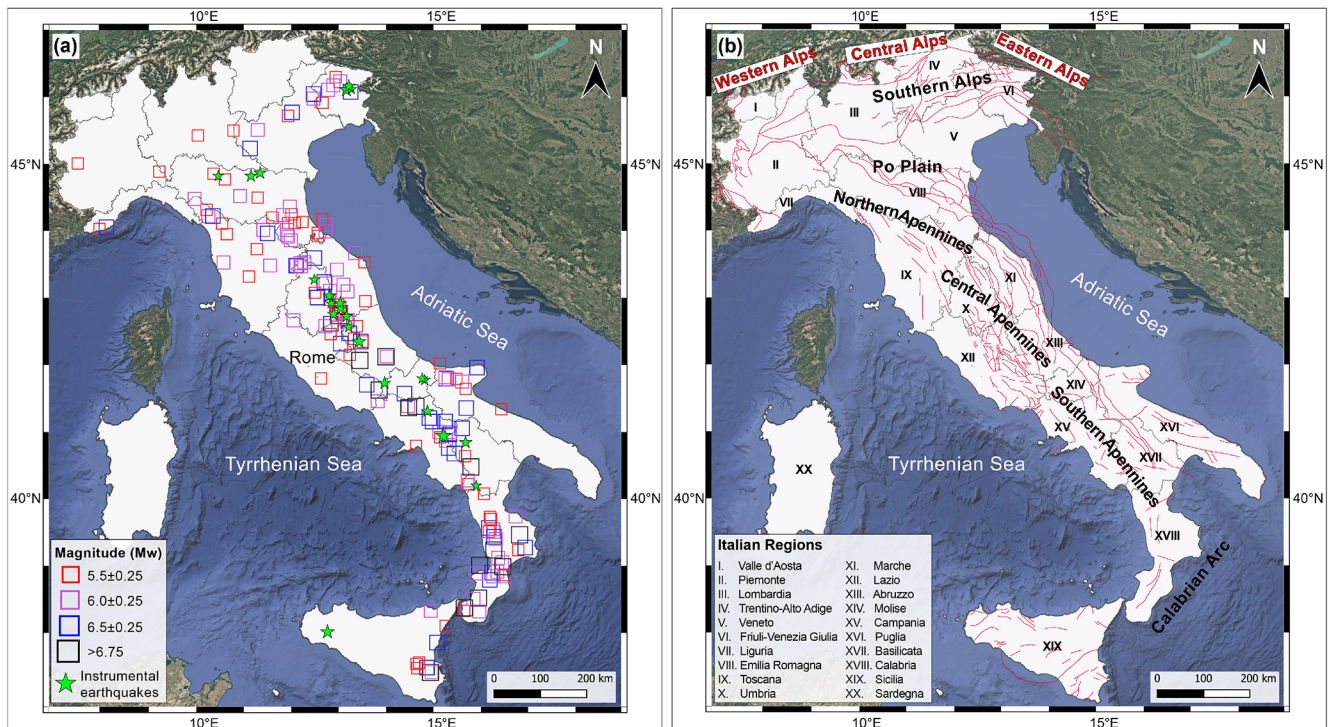
Figure 1. (a) Selected dataset of 191 earthquakes with M_w \geq 5.5 from the CPTI15 catalogue (Rovida et al., 2022). Square colours and sizes are proportional to the earthquake magnitude. Green stars indicate the subset of 24 earthquakes for which instrumental solutions are available. (b) Map of the main physiographic structures and tectonic lineaments of Italy (Bigi et al., 1989) cited in the text. Roman numerals (I to XX) refer to the Italian administrative regions with the names detailed in the legend. Basemap source: Google Satellite imagery. Map data © 2015 Google.
