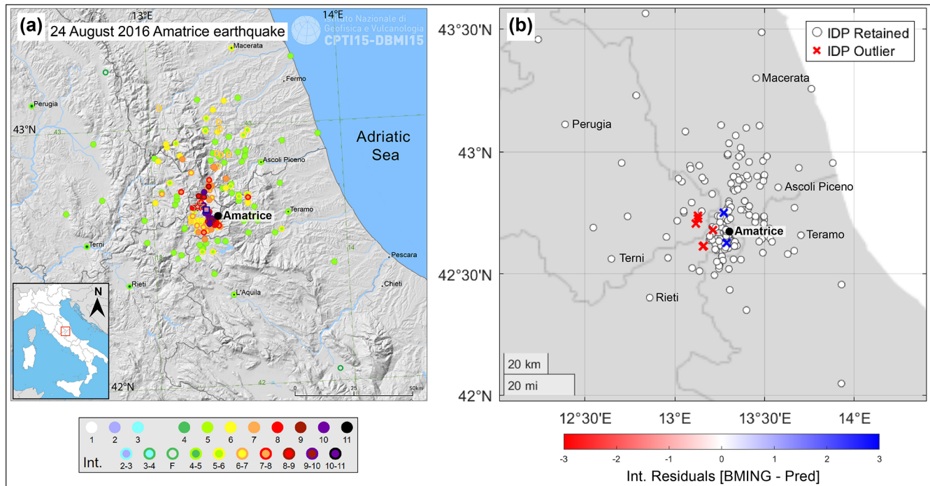
Figure 3. The 24 August 2016 ( M_w 6.18) Amatrice earthquake. (a) Macroseismic intensity distribution of the ROSAL019 dataset from Rossi et al. (2019). (b) Intensity residuals between ROSAL019 observations and predictions from the adopted IPE. Blue crosses indicate intensity outliers with positive residuals (Pescara del Tronto and Amatrice, I = 10 ), whereas red crosses indicate outliers with negative residuals (Terracina, I = 5 –6; Castel S. Maria, Cittareale, Savelli, and Valcaldara, I = 5 ). The map in panel (a) is derived from CPTI15-DBMI15 and uses the TINITALY DEM as background. CPTI15-DBMI15 data courtesy of INGV. © INGV. All rights reserved.
