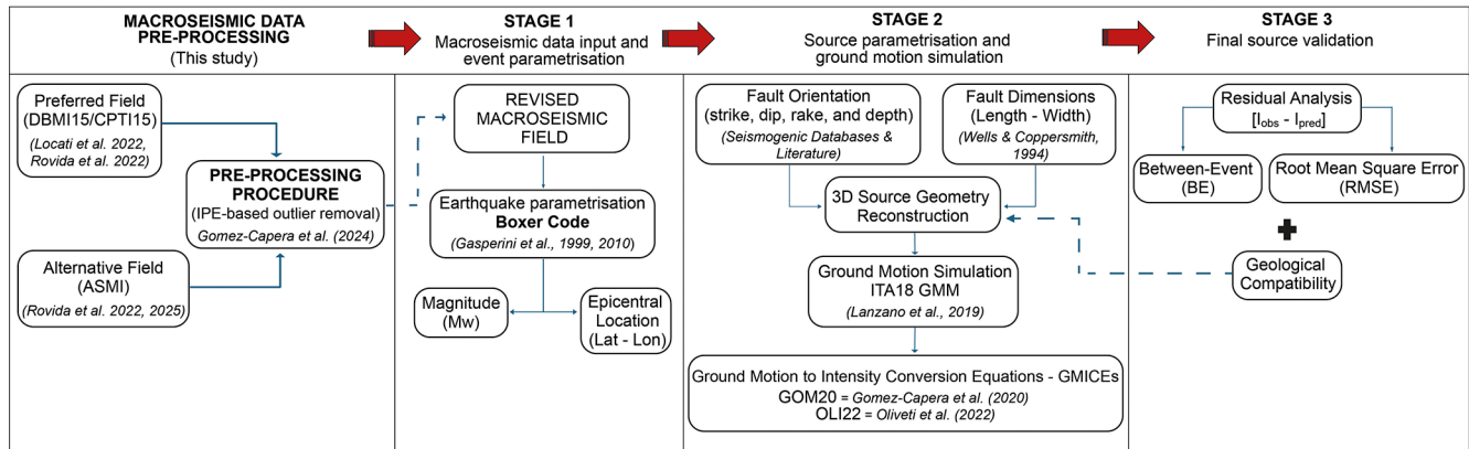
Figure 4. Schematic representation of the integrated workflow adopted for seismogenic source reconstruction, including the macroseismic data pre-processing step. Dashed blue arrows indicate that the revised macroseismic field serves as the primary input to Stage 1, while the results from Stage 3 are iteratively used to validate and refine the 3D source geometry. Notes: GMM, Ground Motion Model; GMICES, Ground Motion to Intensity Conversion Equations; BE, Between-Event error; RMSE, Root Mean Square Error; GOM20, conversion equation by Gomez-Capera et al. (2020); OLI22, conversion equation by Olivetti et al. (2022).
