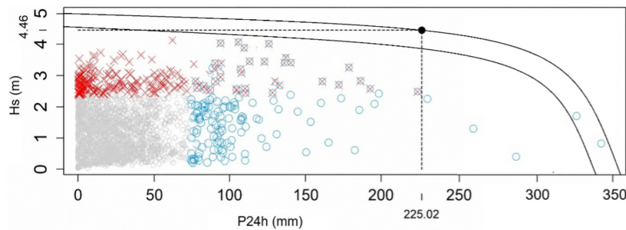
Figure 6. Estimated joint return period of the Gloria storm at the Tordera River mouth. Red crosses denote events with H_s exceeding the local storm threshold, blue circles denote events with P_{24h} exceeding the local precipitation threshold, and grey symbols represent non-extreme conditions. The overlap of red crosses and blue circles denotes compound extreme events. Curves indicate joint return periods of 50 years (inner curve) and 85 years (outer curve), the latter corresponding to Storm Gloria (black filled circle).
