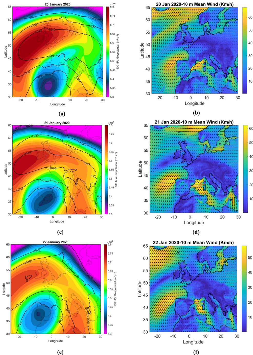
Figure 2. Sea level pressure and 500 hPa geopotential (a, c, e) and mean wind speed (b, d, f) for 20, 21 and 22 January 2020.
