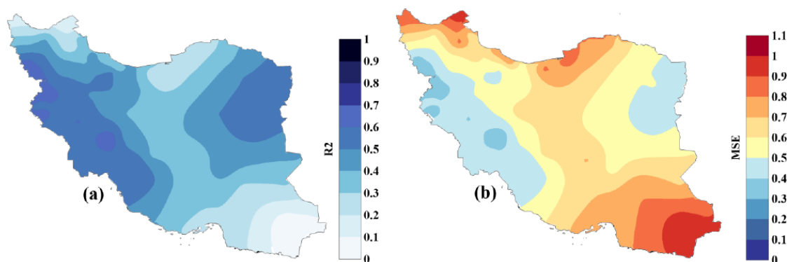
Figure 7. Spatial distribution of the performance of the best-selected model (LSTM) with a 12-month memory input (S2-4) for 1-month-ahead drought forecasting ( \text{SPI}_{t+1} ). (a) Coefficient of Determination ( R^2 ). (b) Mean Squared Error (MSE). The model demonstrates robust predictive capability in the west and northwest, while performance decreases in the hyper-arid southeastern regions.
