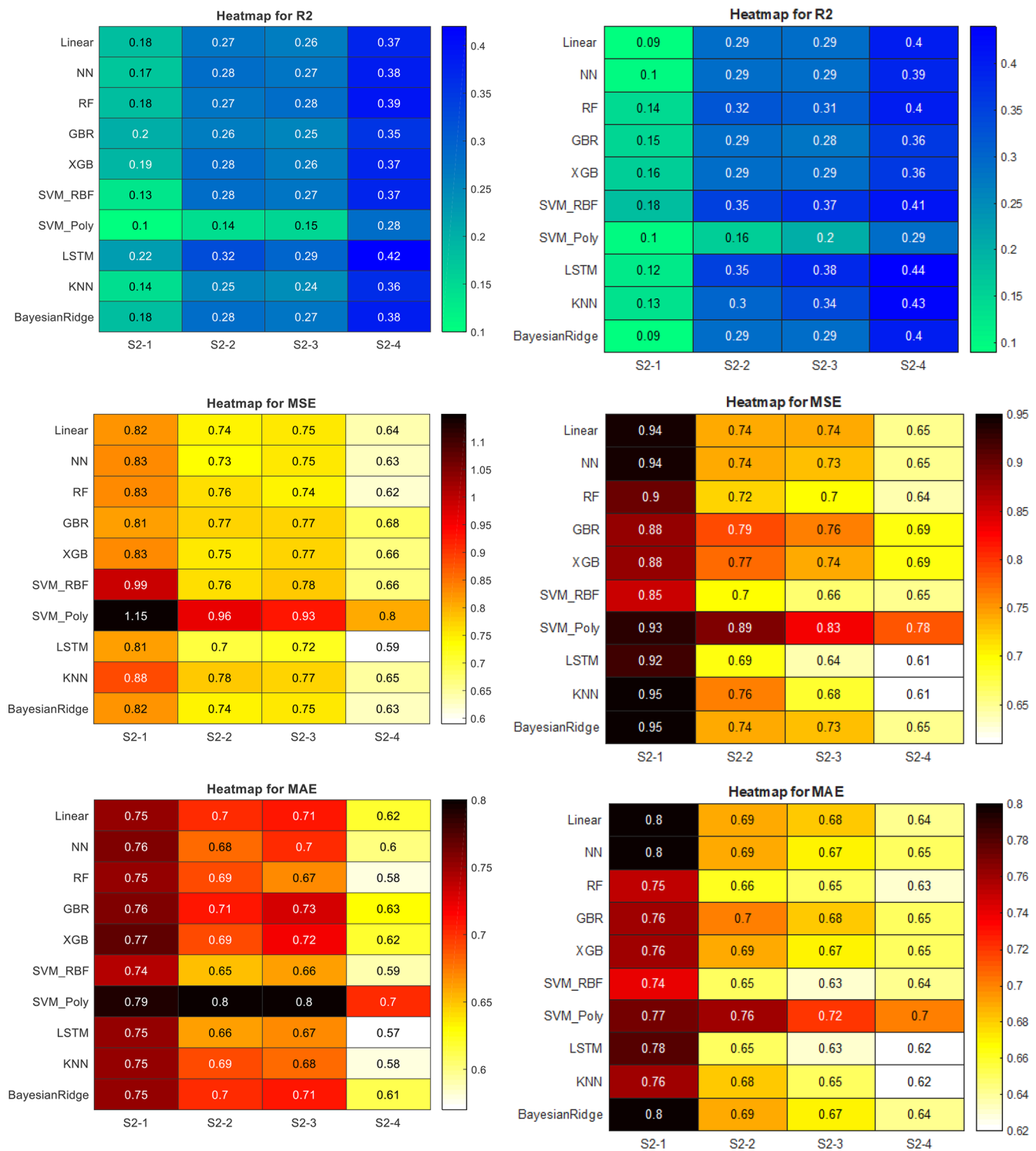
Figure 6. Heatmap of performance metrics ( R^2 , MSE, MAE) for 1-month-ahead SPI prediction ( SPI_{t+1} ) at the Anzali (right columns) and Zabol (left columns) stations under four temporal memory scenarios (S2-1 to S2-4). The results clearly demonstrate that for most models, particularly LSTM, increasing the memory length from 3 months (S2-1) to 12 months (S2-4) leads to a substantial increase in R^2 and a reduction in error, underscoring the importance of longer-term historical data.
