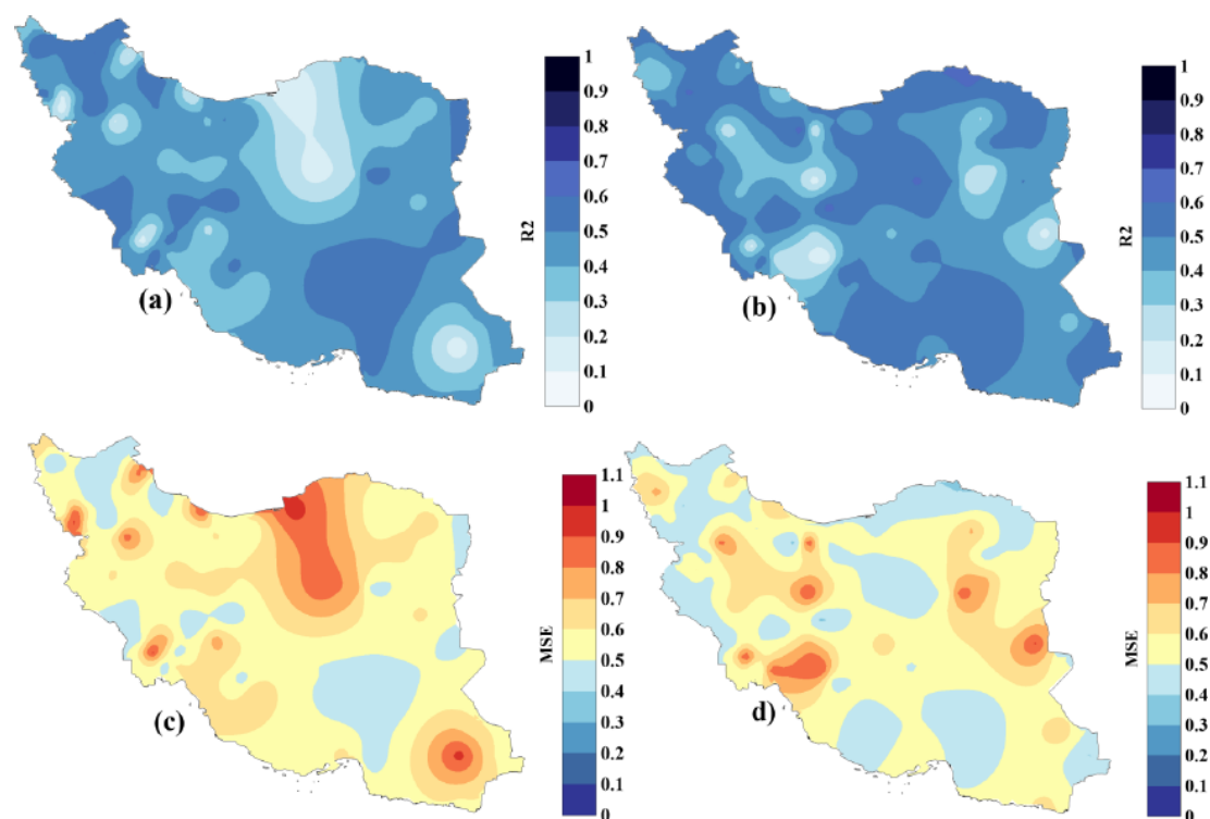
Figure 9. Spatial distribution of the performance ( R^2 and MSE) of the superior Random Forest (RF) model for 1-month-ahead prediction ( SPI_{t+1} ) under hybrid scenarios S3-1 and S3-2. The maps reveal a clear spatial complementarity: S3-2 (b, d) excels in the north and west, while S3-1 (a, c) provides necessary coverage and higher accuracy in the eastern and central regions.
