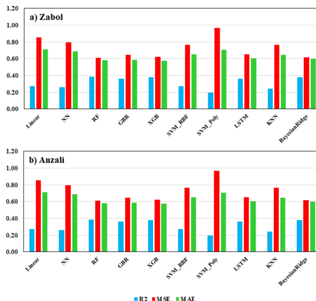
Figure 4. Performance comparison of different machine learning algorithms for 1-month-ahead drought forecasting ( SPI_{t+1} ) under Scenario S1 across selected representative stations. The Random Forest (RF) model demonstrates superior accuracy and lower error rates compared to other models.
