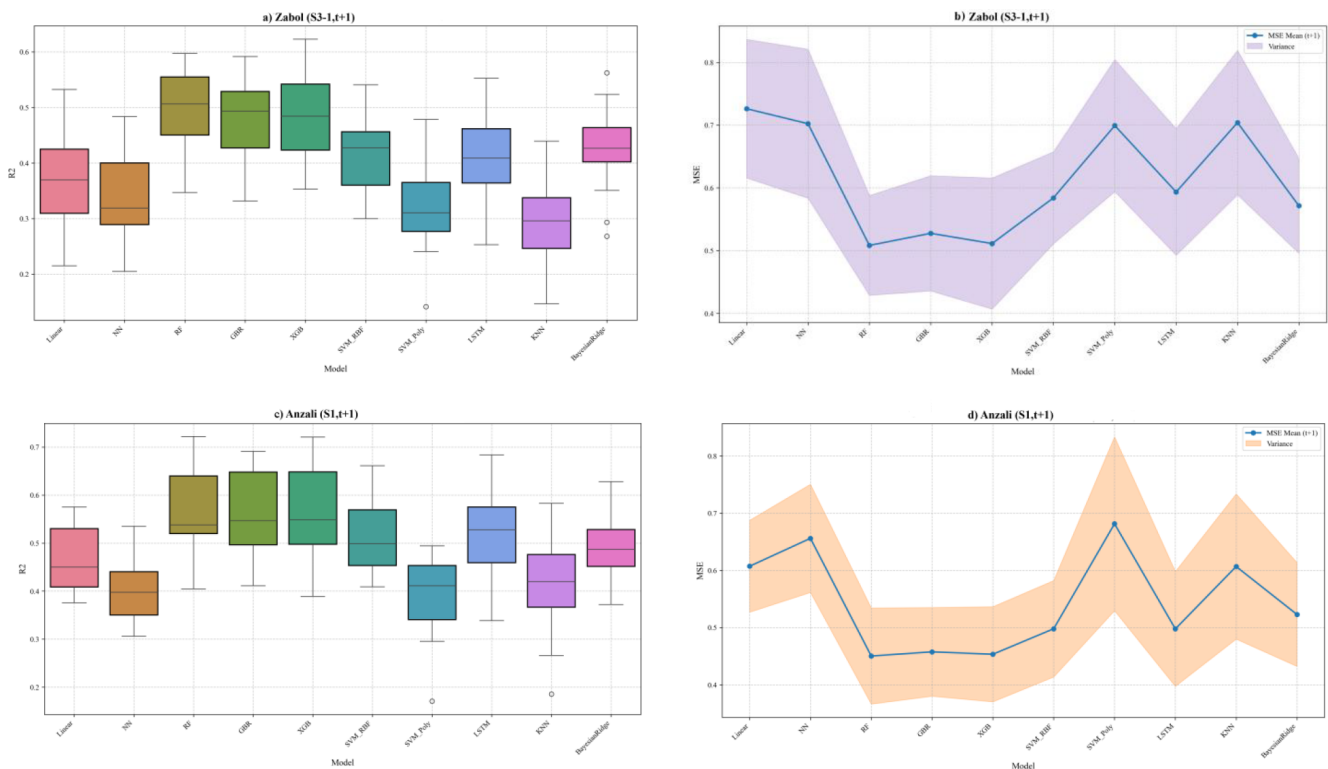
Figure 10. Uncertainty analysis of the models for the 1-month forecast horizon ( t + 1 ) based on 20 independent runs. (a, b) Zabol station under Scenario S3-1. (c, d) Anzali station under Scenario S1. Left panels display the distribution of R^2 (boxplots), and right panels show the mean MSE (solid line) with the 95 % confidence interval (shaded area).
