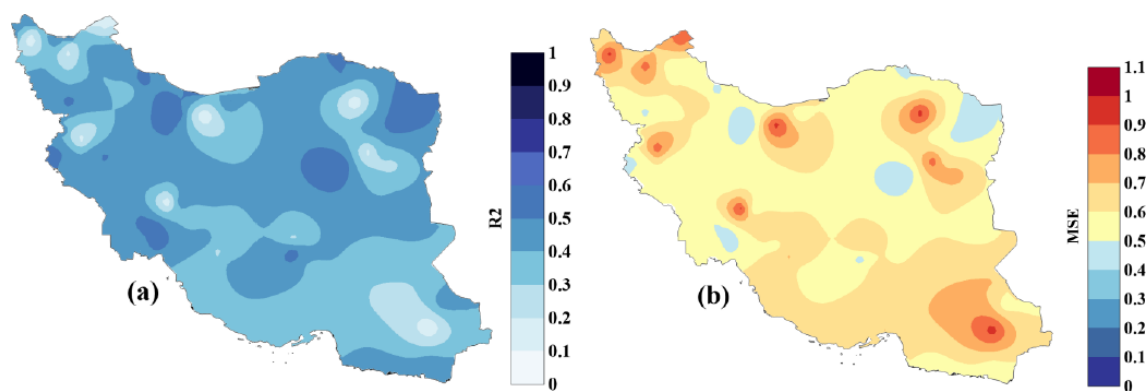
Figure 5. Spatial distribution of the performance of the best-selected model (Random Forest) for 1-month-ahead drought forecasting ( \text{SPI}_{t+1} ) under Scenario S1. (a) Coefficient of Determination ( R^2 ). (b) Mean Squared Error (MSE).
