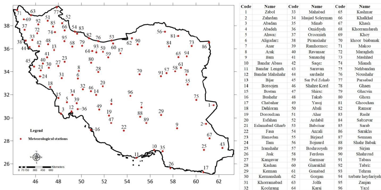
Figure 2. Spatial distribution of the 96 selected synoptic meteorological stations across Iran. The numerical code for each station is indicated on the map, and its corresponding name is provided in the legend table next to the map. This network covers Iran's extensive climatic diversity for the subsequent analyses.
