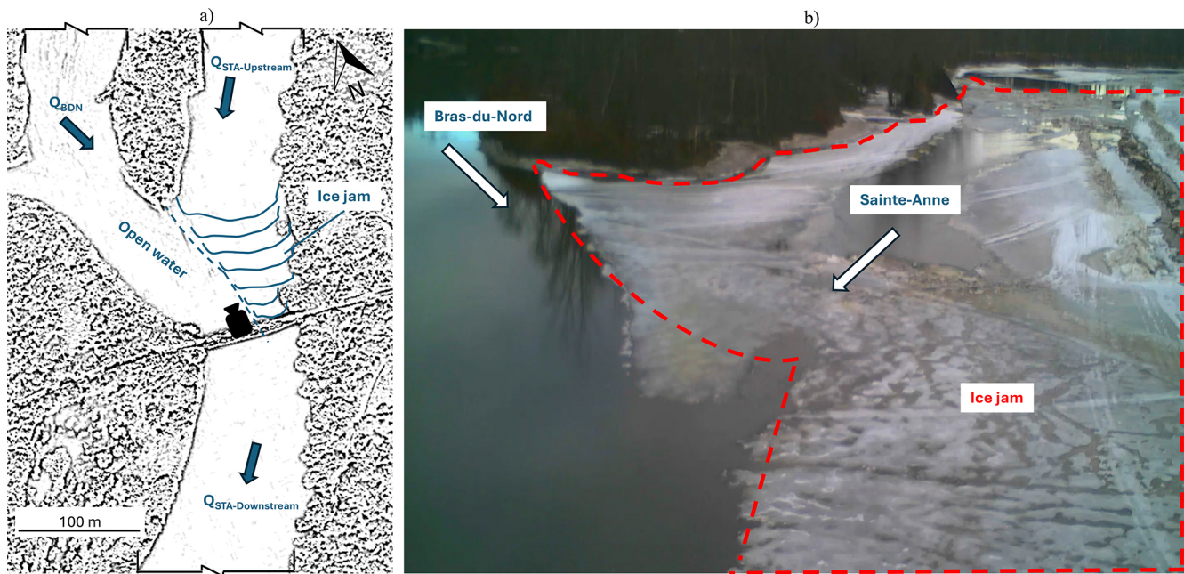
Figure 8. Jamming due to flow impact with (a) a schematic representation and (b) a picture taken at site BDN0-STA3 on 7 April 2021, looking upstream towards the flow as represented by the camera symbol in panel (a), where the ice jam appeared at STA-BDN. The red dotted line in panel (b) represents the ice jam caused by the effect of flow impact from the BDN on the ice in STA.
