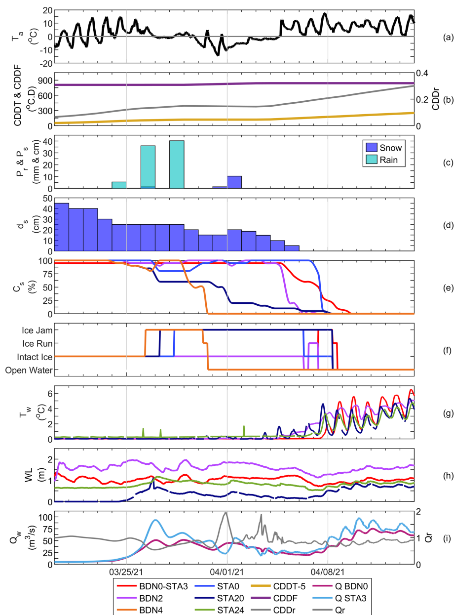
Figure 4. Time series of hydrometeorological conditions during the 2021 breakup at STA-BDN (20 March to 14 April 2021) showing (a) air temperature, (b) CDDT, CDDF and CDDr, (c) daily precipitation, (d) snow on ground, (e) surface ice concentration, (f) ice states, (g) water temperature, (h) water level above the pressure probe and (i) discharge and Qr.
