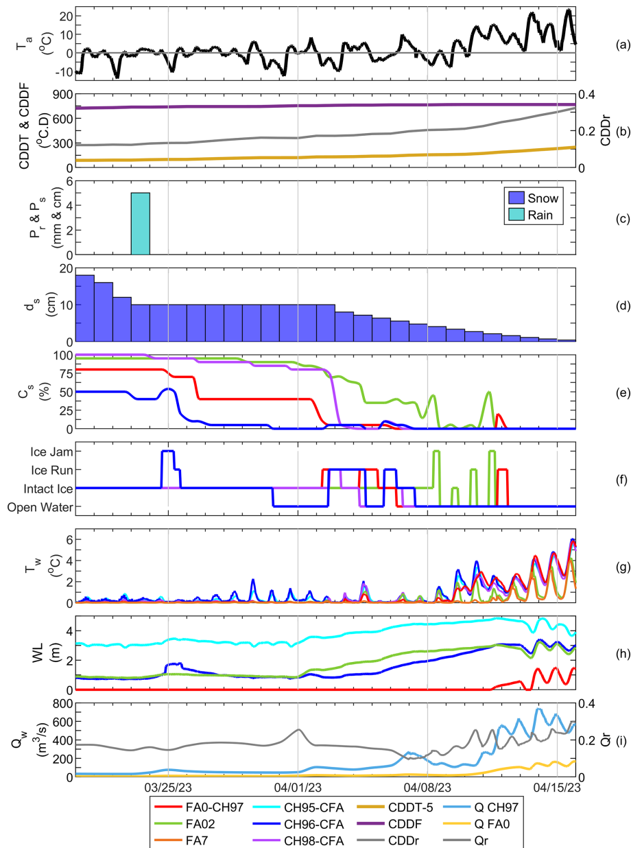
Figure 6. Time series of hydrometeorological conditions during the 2023 breakup at CH-FA (20 March to 16 April 2023) showing (a) air temperature, (b) CDDT, CDDF and CDDr, (c) daily precipitation, (d) snow on ground, (e) surface ice concentration, (f) ice states, (g) water temperature, (h) water level above the pressure probe and (i) discharge and Q_r .
