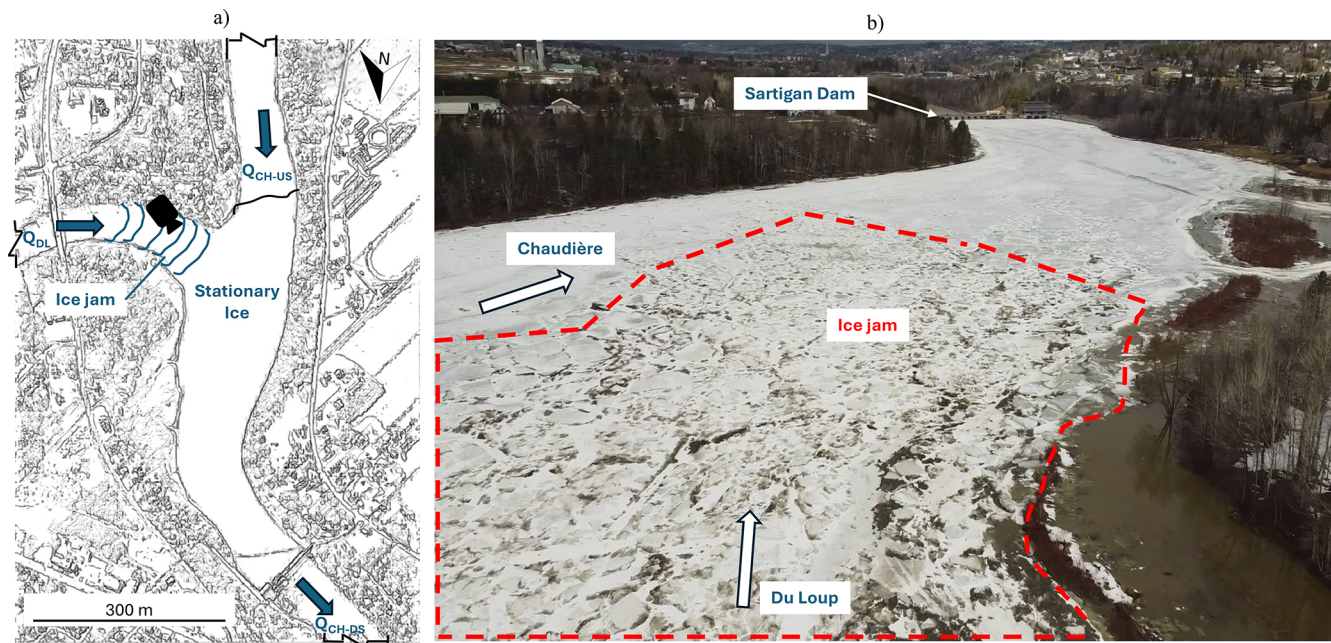
Figure 10. Jamming due to stationary ice with (a) a visual representation and (b) a drone picture taken at site DL0-CH104 on 31 March 2022, looking downstream in the flow direction as represented by the camera symbol in panel (a) where the ice jam appeared at CH-DL.
