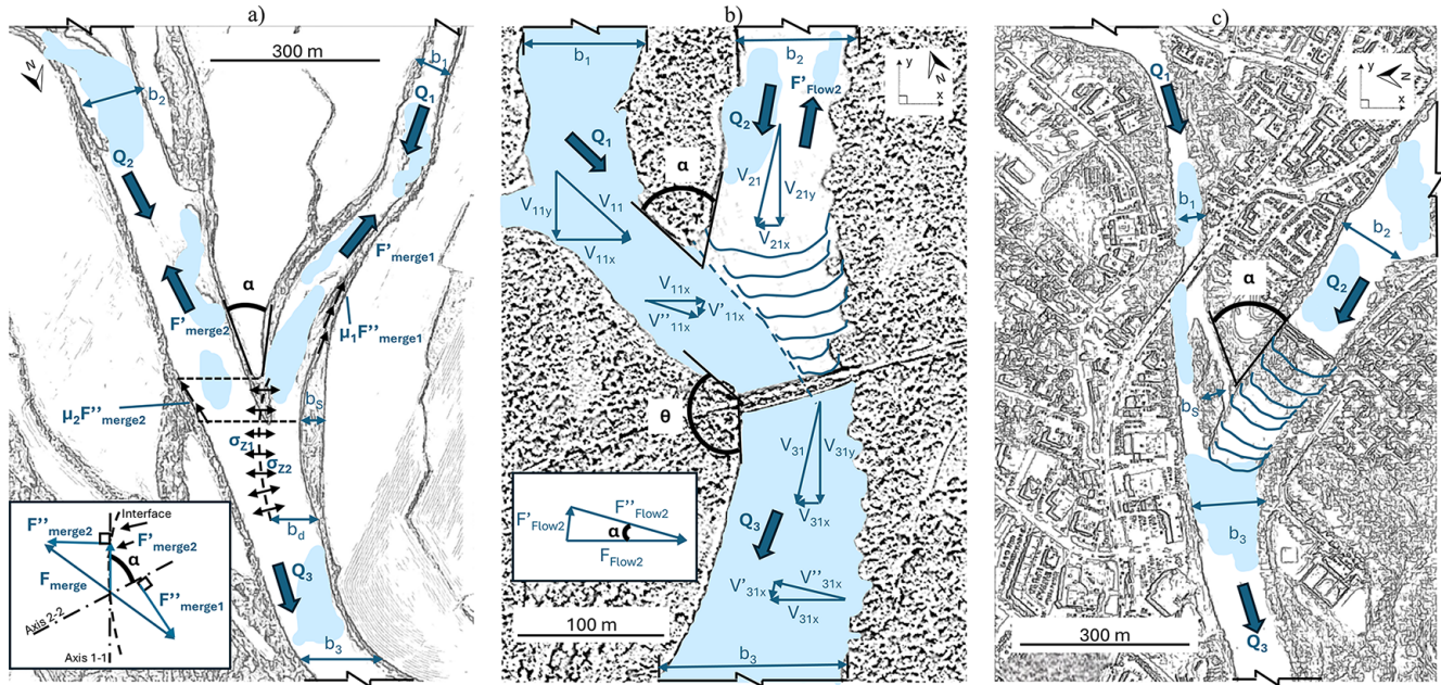
Figure 3. Visual representation of the forces applied showing (a) a plan view of the ice jam due to merging ice runs at CH-BSV (process 3), (b) a plan view of the flow impact mechanism at STA-BDN (process 5) and (c) a plan view of the ice jam due to a confluence bar at CH-FA (process 6). The light blue in the background corresponds to ice free.
