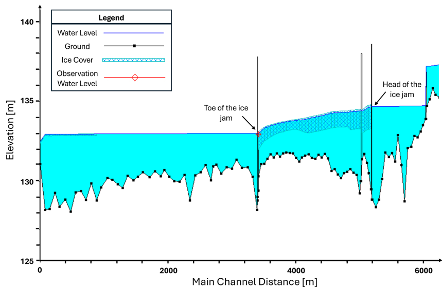
Figure 9. Profile of calibrated ice jam of 7 April 2021, on the STA River confluence.
