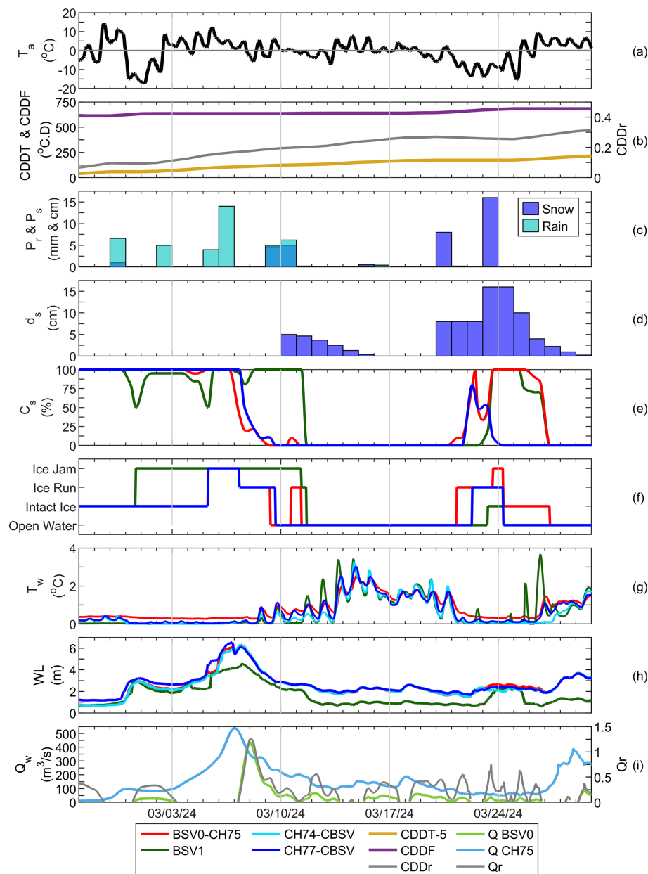
Figure 7. Time series of hydrometeorological conditions during the 2024 breakup at CH-BSV (26 February to 30 March 2024) showing (a) air temperature, (b) CDDT, CDDF and CDDr, (c) daily precipitation, (d) snow on ground, (e) surface ice concentration, (f) ice states, (g) water temperature, (h) water level above the pressure probe and (i) discharge and Q_r .
