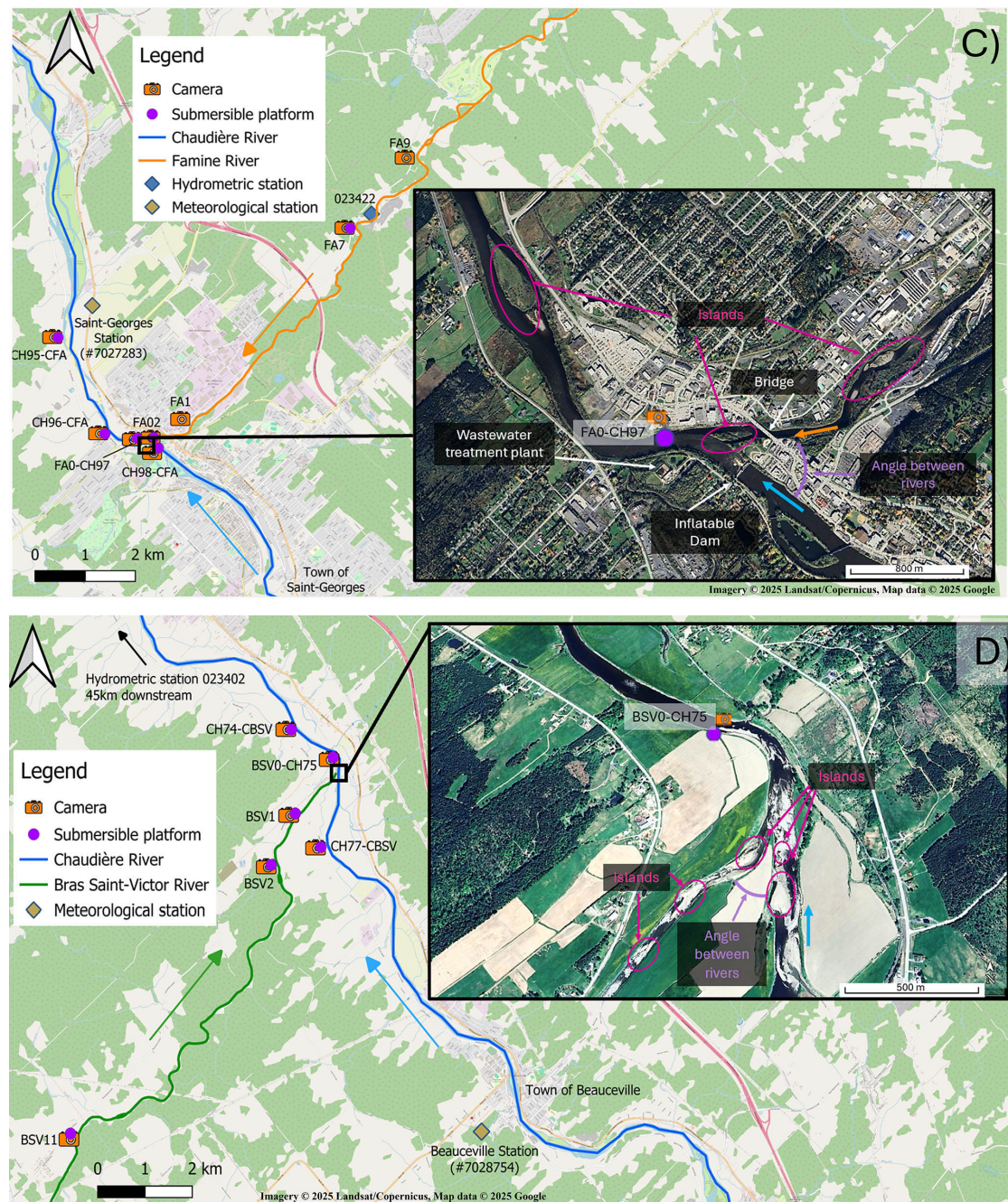
Figure 2. Study sites showing instrumentation locations at each measurement sites with their respective site ID for (A) STA-BDN, (B) CH-DL, (C) CH-FA, and (D) CH-BSV. The insert is an aerial zoomed in photo of the confluence to highlight the morphological features (A) Imagery © 2025 Airbus, Map data © 2025 Google; (B, C, D) Imagery © 2025 Landsat/Copernicus, Map data © 2025 Google) (Google, 2025a, b). The sites ID in these figures indicates the river where the instrument was located followed by its stationing from the downstream boundary (Chute-Panet Dam for STA and Innergex Dam for CH).
