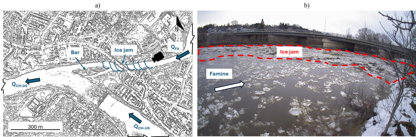
Figure 11. Jamming on depositional fan with (a) a visual representation and (b) a picture taken at site FA02 on 11 April 2023, looking downstream in the flow direction of FA as represented by the camera symbol in panel (a), where the ice jam appeared at the mouth of the FA.
