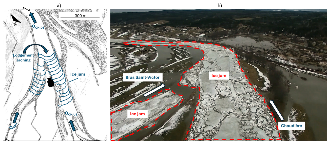
Figure 12. Jamming of arching ice pieces with (a) a visual representation and (b) a drone picture taken at site BSV0-CH75 on 6 March 2024, looking downstream in the flow direction as represented by the camera symbol in panel (a), where the ice jam occurred at CH-BSV.
