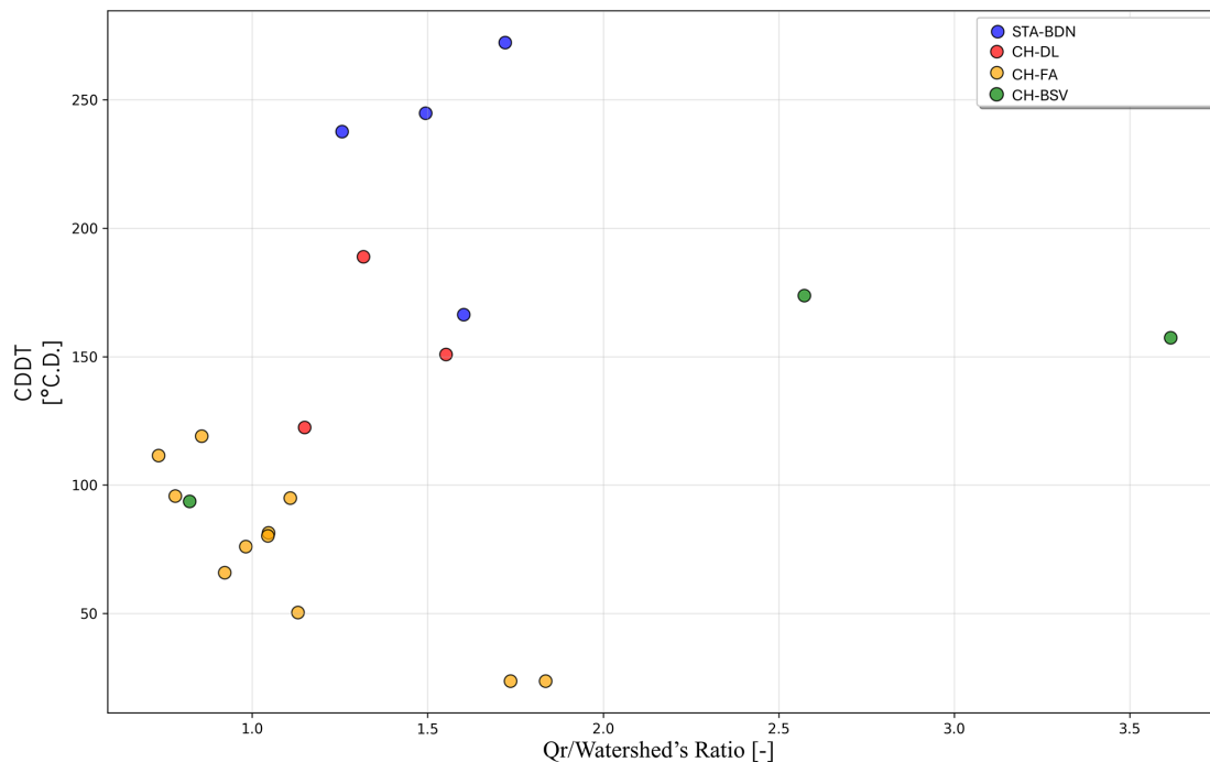
Figure 13. Relationship between discharge ratio ( Q_r ) divided by the Watershed's Ratio (from Table 1) and cumulative degree-days of thawing (CDDT) on the ice jam day at the confluence site over the study period for all four confluences studied.
