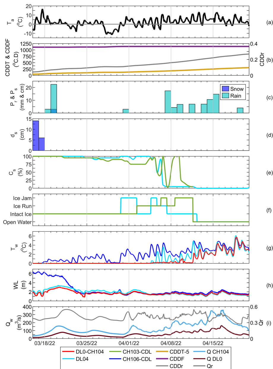
Figure 5. Time series of hydrometeorological conditions during the 2022 breakup at CH-DL (16 March to 21 April 2022) showing (a) air temperature, (b) CDDT, CDDF and CDDr, (c) daily precipitation, (d) snow on ground, (e) surface ice concentration, (f) ice states, (g) water temperature, (h) water level above the pressure probe and (i) discharge and Qr.
